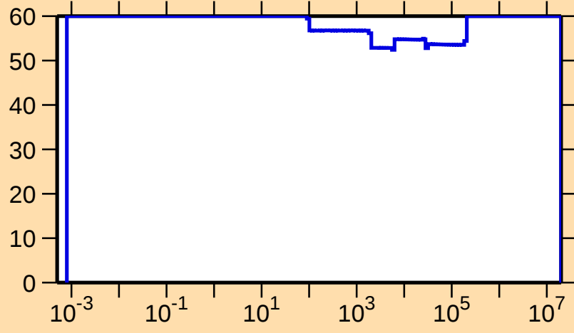
\Delta\sigma/\sigma vs. E for ^{113}\text{Te}(n,p)
