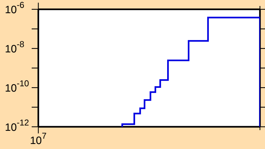
\sigma vs. E for ^{113}\text{Te}(\text{mt } 34)
