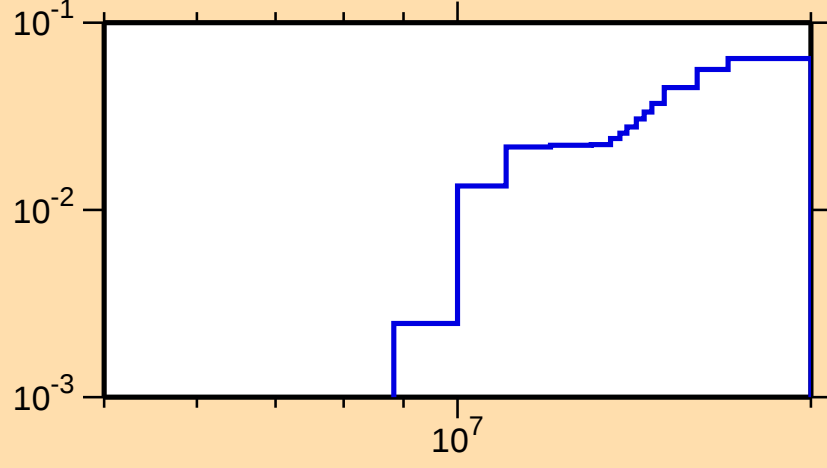
\sigma vs. E for ^{113}\text{Te}(n,2n)
