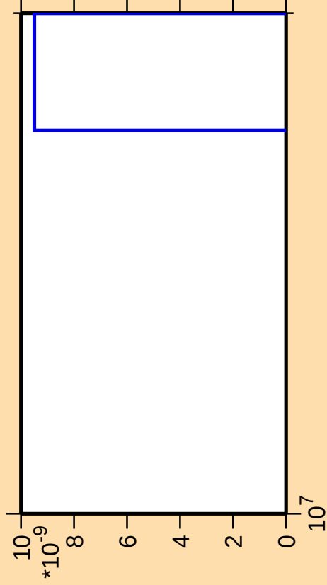
\Delta\sigma/\sigma vs. E for ^{113}\text{Te}(n,3n\alpha)
