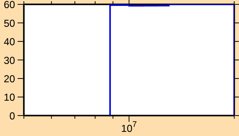
\Delta\sigma/\sigma vs. E for ^{113}\text{Te}(n,\text{inel.})
