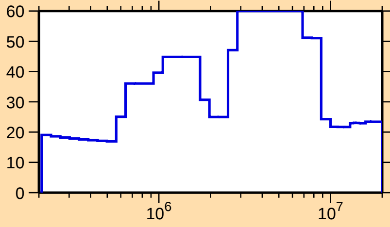
\Delta\sigma/\sigma vs. E for ^{113}\text{Te}(\text{n,el.})
