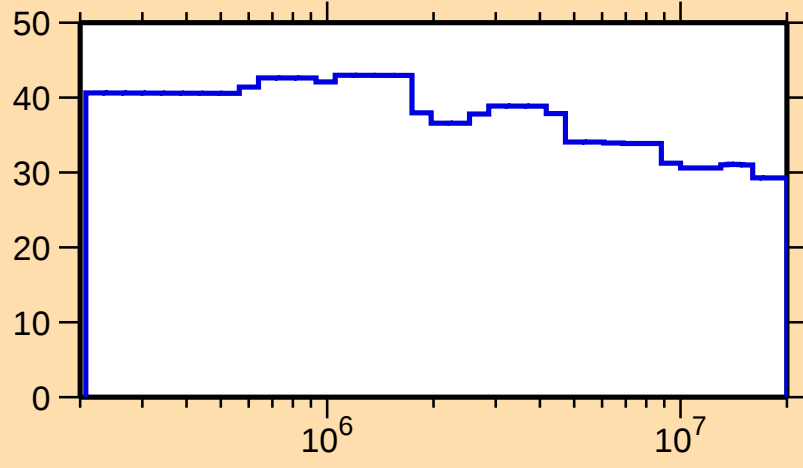
\Delta\sigma/\sigma vs. E for ^{113}\text{Te}(n,n\text{onel.})
