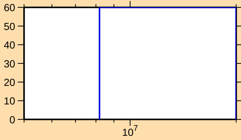
\Delta\sigma/\sigma vs. E for ^{113}\text{Te}(n,\text{inel.})
