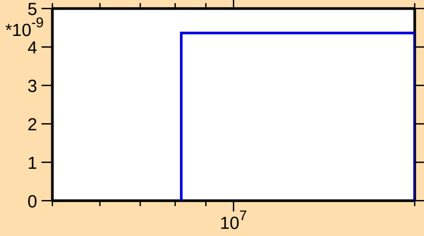
\sigma vs. E for ^{113}\text{Te}(\text{mt } 34)
