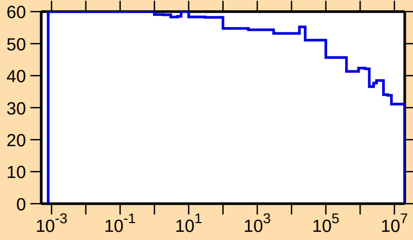
\Delta\sigma/\sigma vs. E for ^{113}\text{Te}(n,\text{nonel.})
