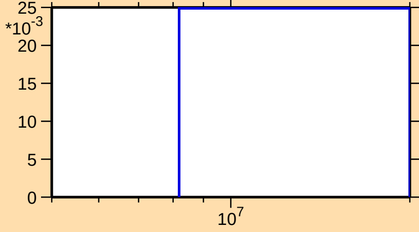
\sigma vs. E for ^{113}\text{Te}(n,2n)
