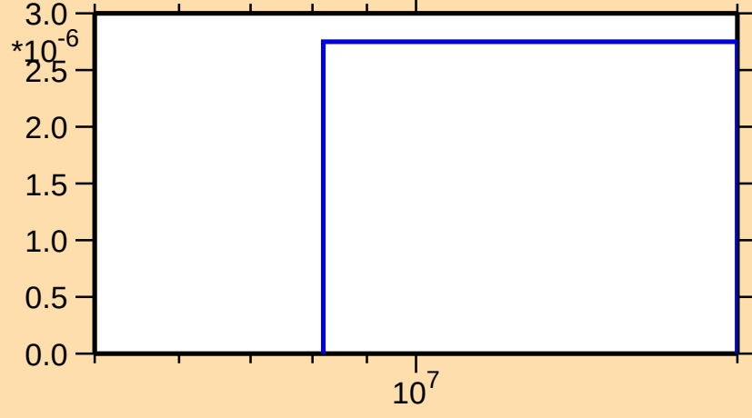
\sigma vs. E for ^{113}\text{Te}(n,\text{pt})
