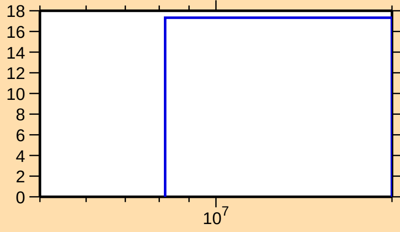
\Delta\sigma/\sigma vs. E for ^{113}\text{Te}(n,\text{tot.})
