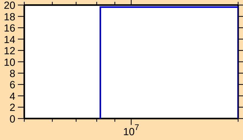
\Delta\sigma/\sigma vs. E for ^{113}\text{Te}(n,\text{el.})
