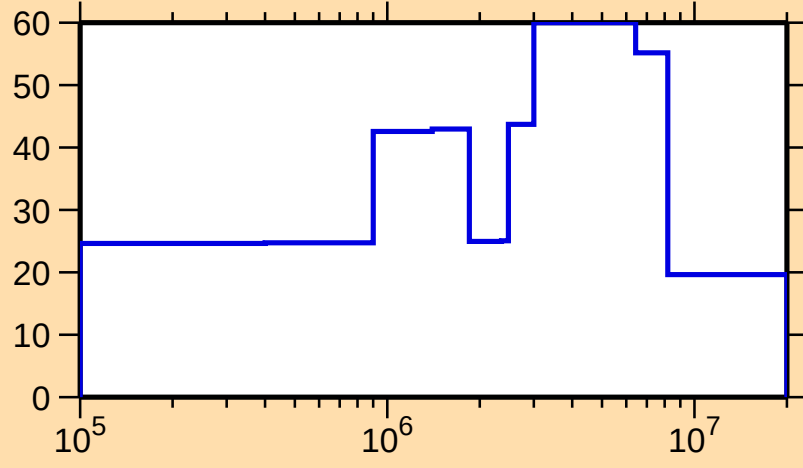
\Delta\sigma/\sigma vs. E for ^{113}\text{Te}(n,\text{el.})
