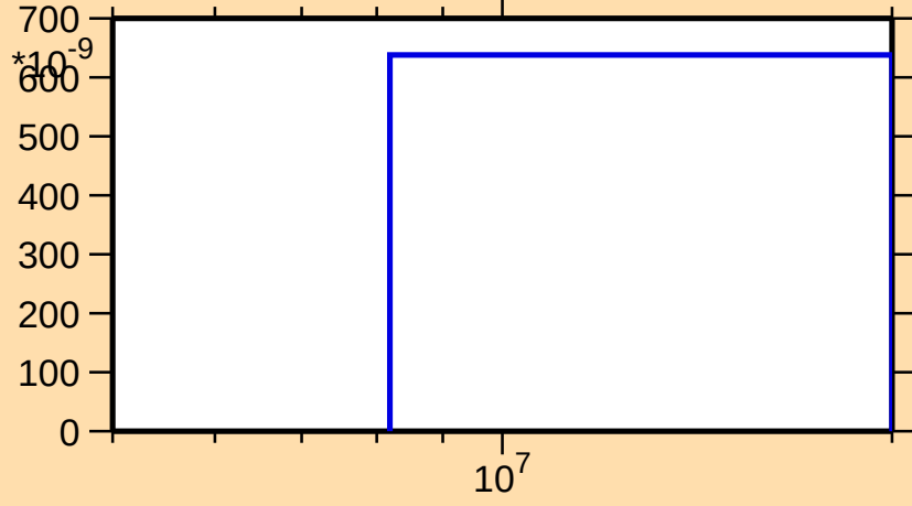
\sigma vs. E for ^{113}\text{Te}(\text{mt } 45)
