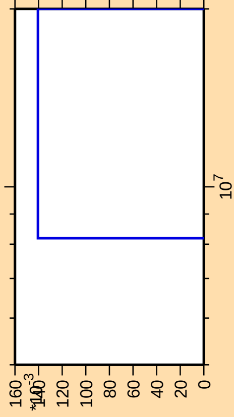
\Delta\sigma/\sigma vs. E for ^{113}\text{Te}(n,nt)
