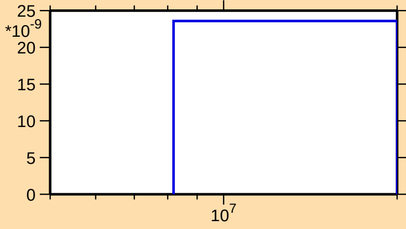
\sigma vs. E for ^{113}\text{Te}(\text{mt117})
