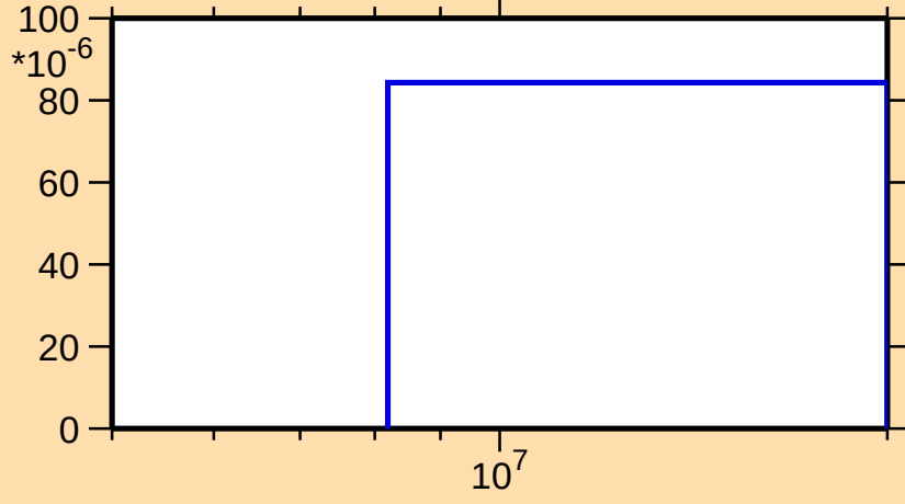
\sigma vs. E for ^{113}\text{Te}(n,2np)
