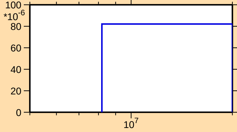
\sigma vs. E for ^{113}\text{Te}(n,\text{pd})
