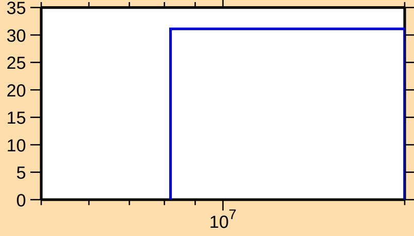
\Delta\sigma/\sigma vs. E for ^{113}\text{Te}(n,\text{nonel.})
