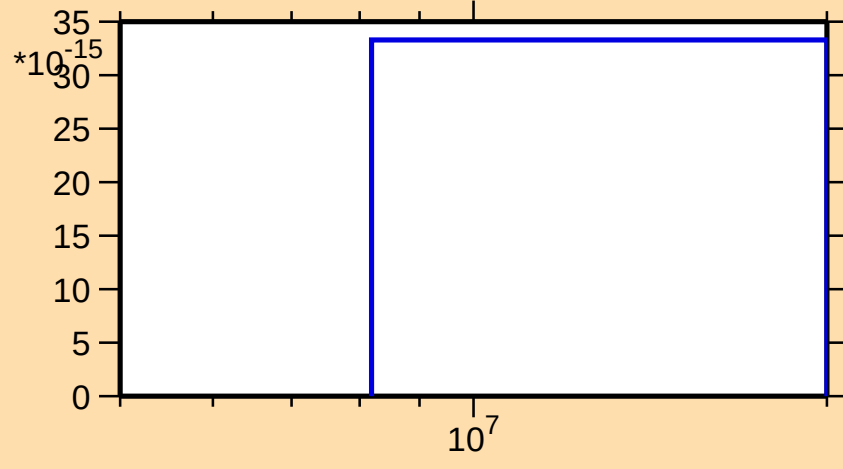
\sigma vs. E for ^{113}\text{Te}(n,nt)
