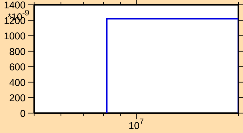
\sigma vs. E for ^{113}\text{Te}(n,\text{nd})
