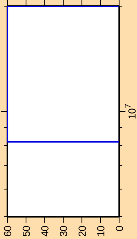
\Delta\sigma/\sigma vs. E for ^{113}\text{Te}(n,n\text{cont.})
