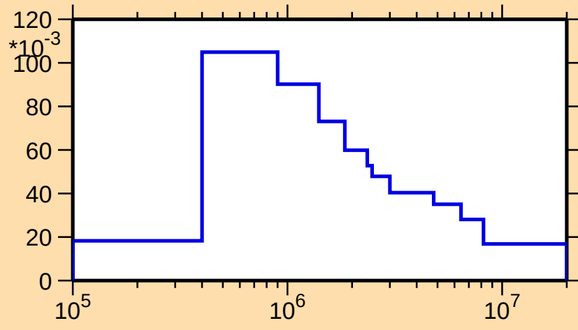
\sigma vs. E for ^{113}\text{Te}(n,n_1)
