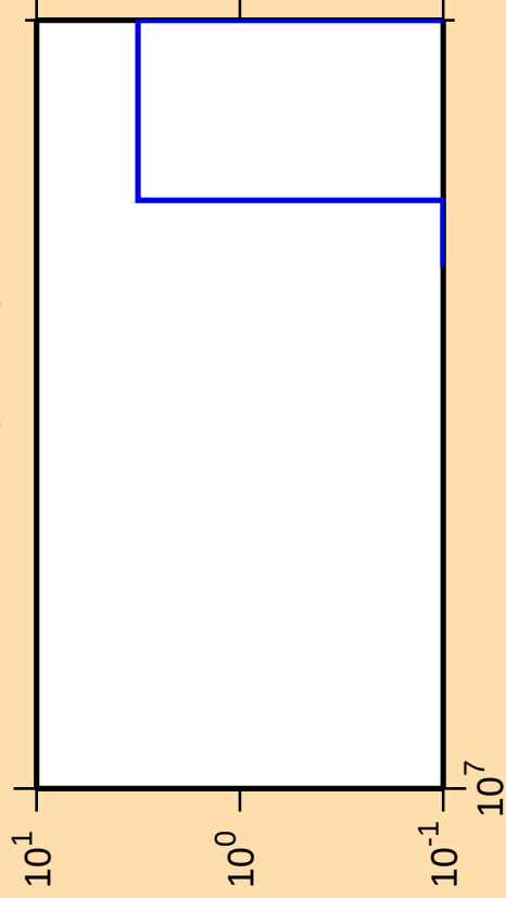
\Delta\sigma/\sigma vs. E for ^{119}\text{Te}(\text{mt 45})
