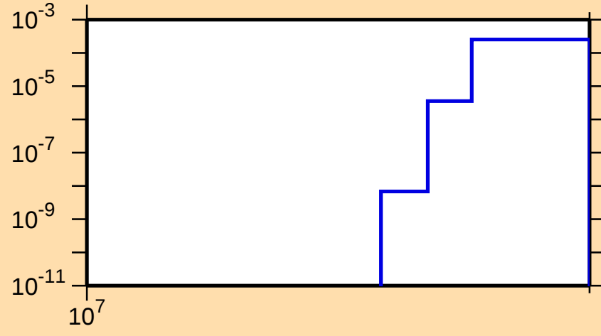
\sigma vs. E for ^{119}\text{Te}(n,2np)
