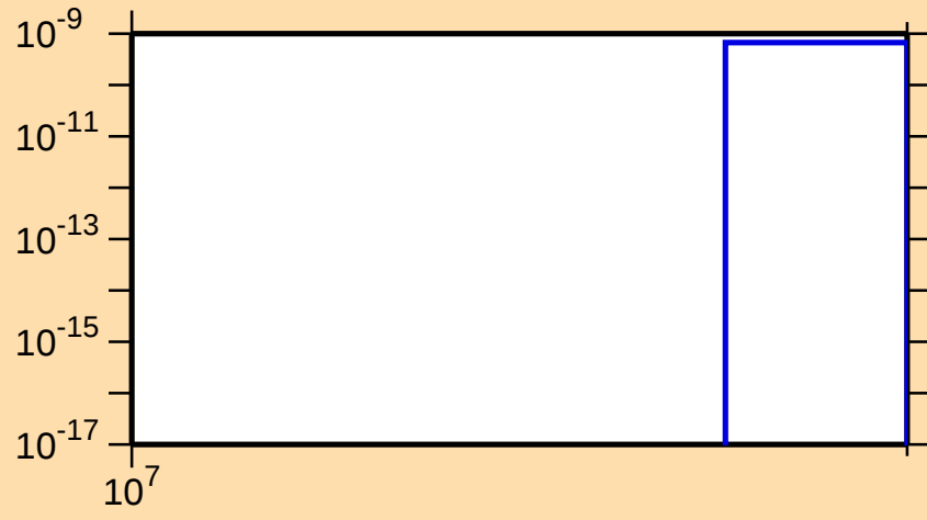
\sigma vs. E for ^{119}\text{Te}(n,nt)
