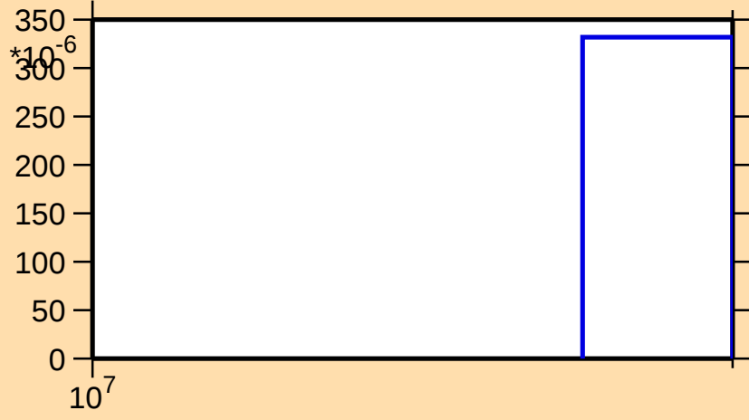
\sigma vs. E for ^{119}\text{Te}(n,3n)
