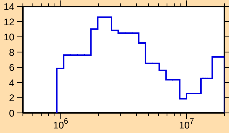
\Delta\sigma/\sigma vs. E for ^{119}\text{Te}(n,\text{tot.})
