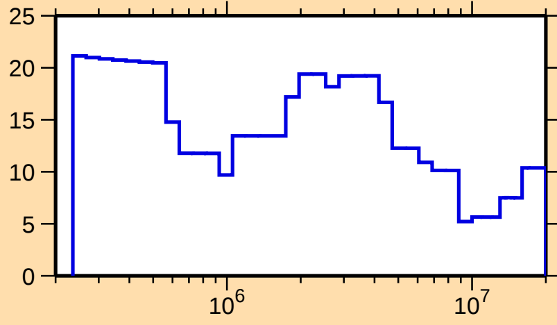
\Delta\sigma/\sigma vs. E for ^{119}\text{Te}(\text{n,el.})
