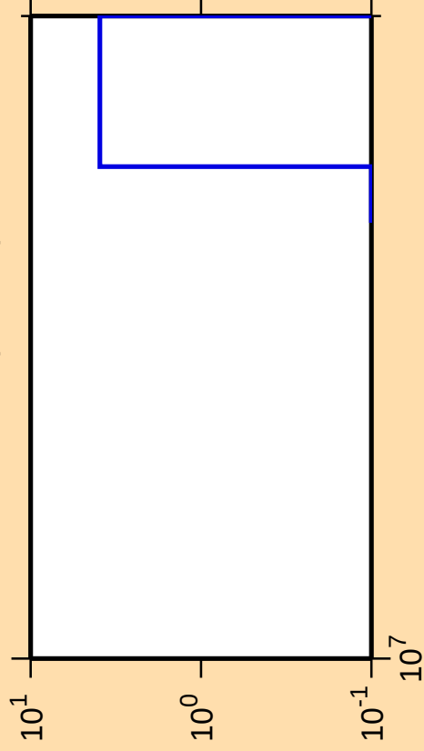
\Delta\sigma/\sigma vs. E for ^{119}\text{Te}(\text{mt117})
