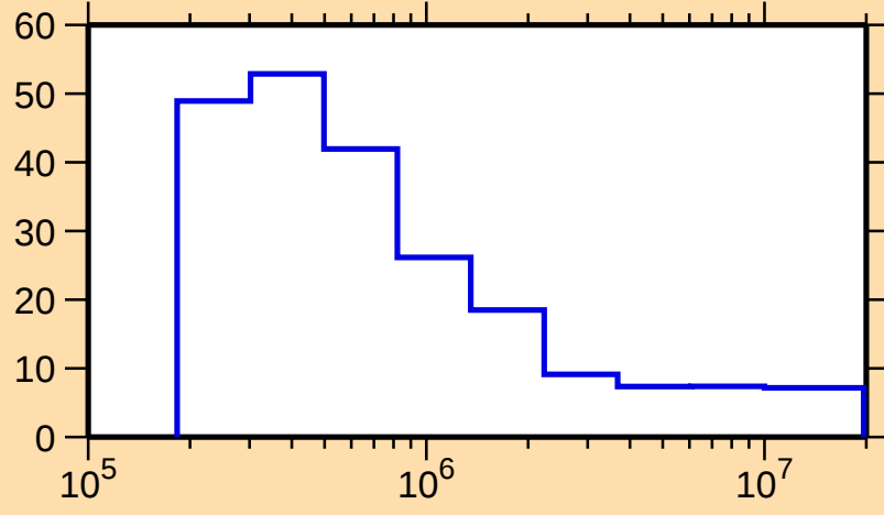
\Delta\sigma/\sigma vs. E for ^{119}\text{Te}(\text{n,inel.})
