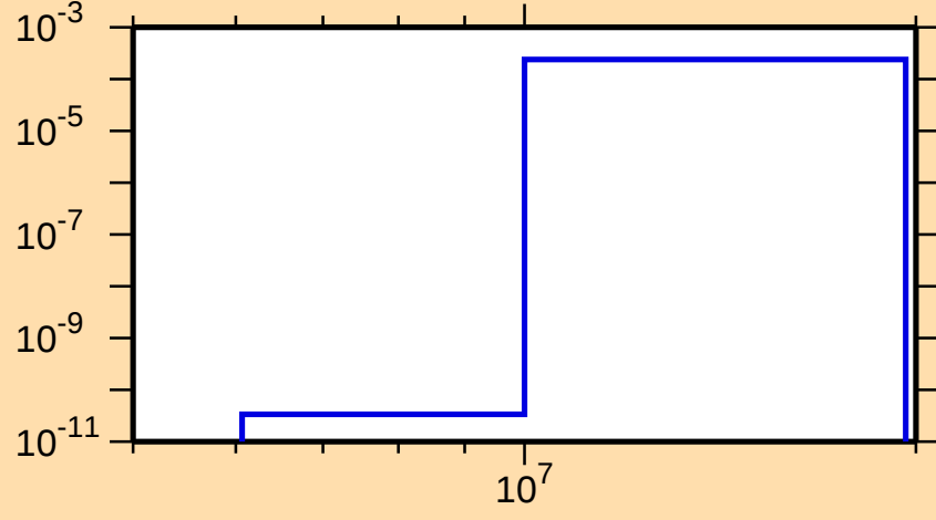
\sigma vs. E for ^{119}\text{Te}(n,t)
