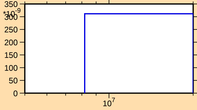
\sigma vs. E for ^{119}\text{Te}(n,\text{nd})
