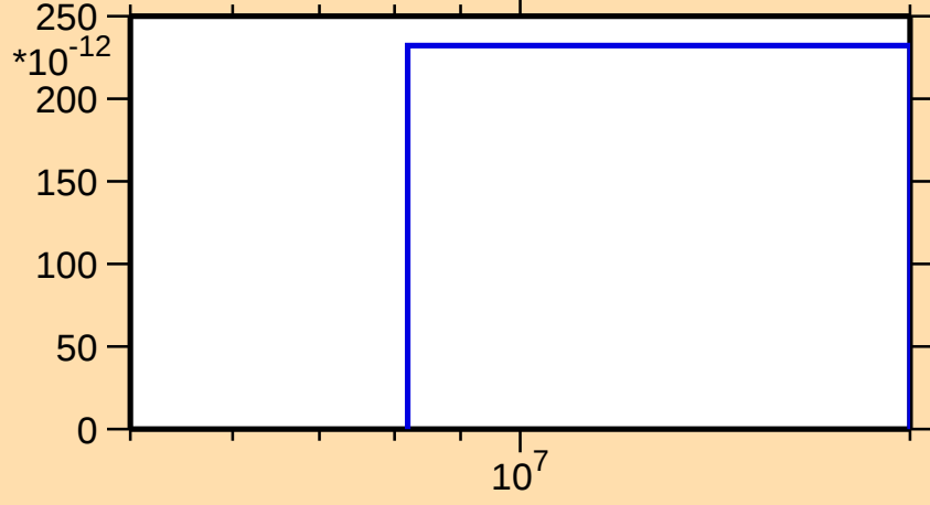
\sigma vs. E for ^{119}\text{Te}(n,\text{pd})
