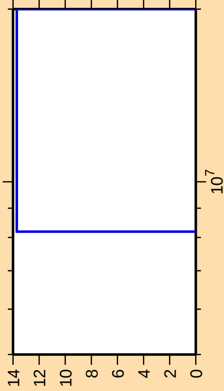
\Delta\sigma/\sigma vs. E for ^{119}\text{Te}(\text{mt } 34)
