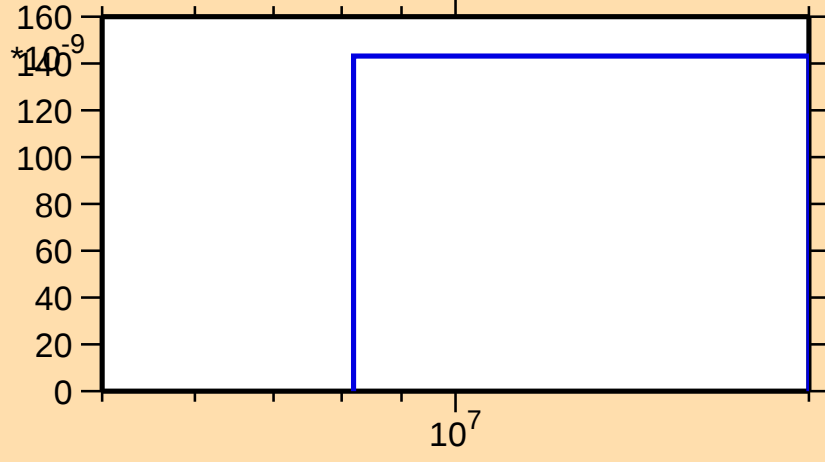
\sigma vs. E for ^{119}\text{Te}(n,\text{He3})
