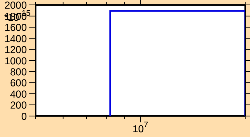
\sigma vs. E for ^{119}\text{Te}(\text{mt } 34)
