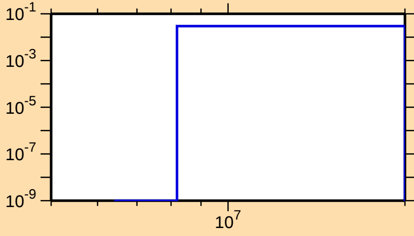
\sigma vs. E for ^{119}\text{Te}(n,np)
