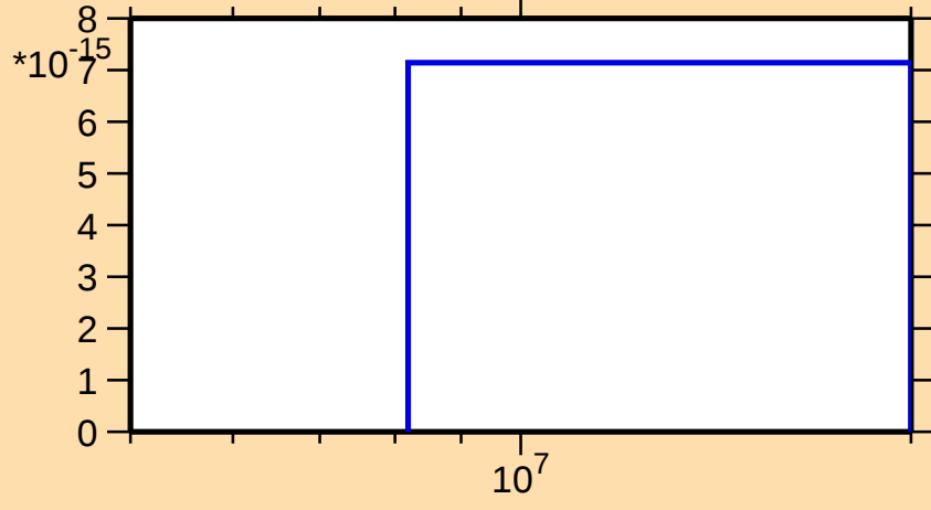
\sigma vs. E for ^{119}\text{Te}(\text{mt } 45)
