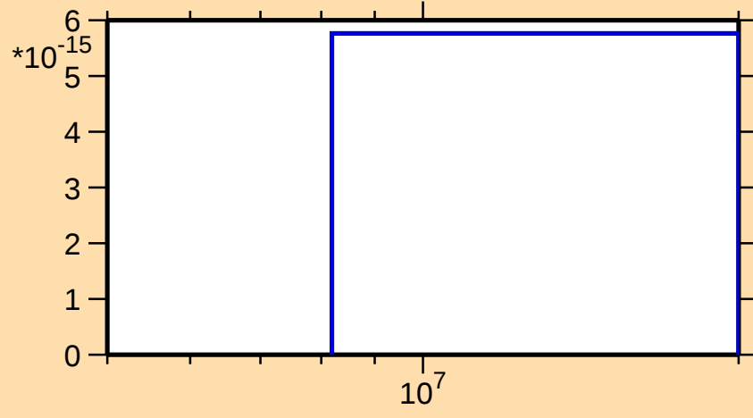
\sigma vs. E for ^{119}\text{Te}(\text{mt117})
