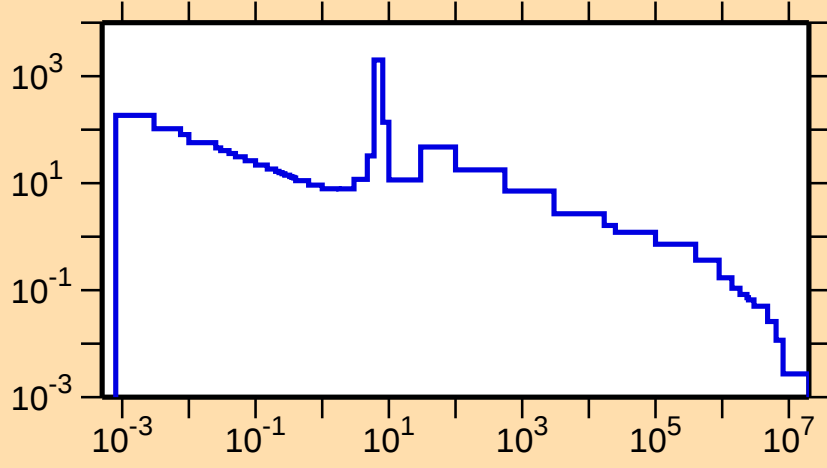
\sigma vs. E for ^{119}\text{Te}(n,\gamma)
