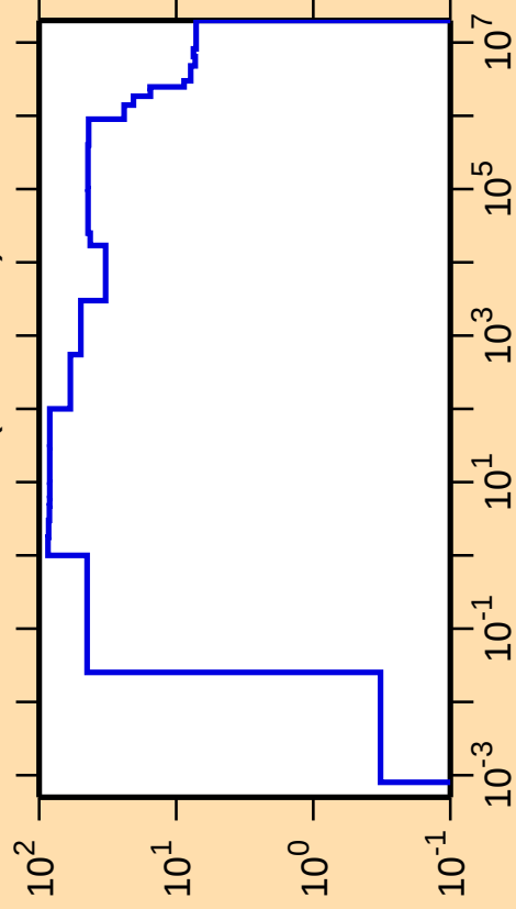
\Delta\sigma/\sigma vs. E for ^{119}\text{Te}(n,\text{nonel.})
