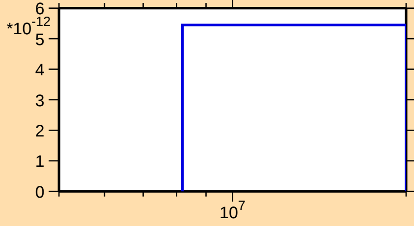
\sigma vs. E for ^{119}\text{Te}(n,nt)
