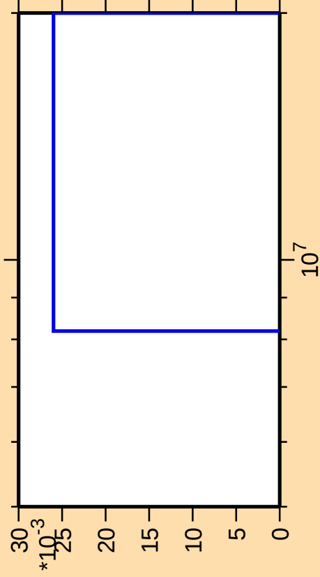
\Delta\sigma/\sigma vs. E for ^{119}\text{Te}(\text{mt } 45)
