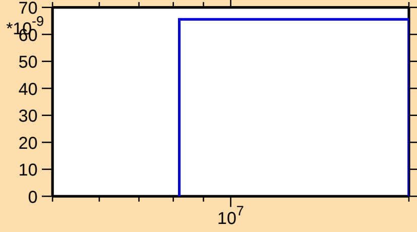
\sigma vs. E for ^{119}\text{Te}(n,p\alpha)
