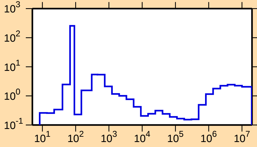
\sigma vs. E for ^{122}\text{Te}(n,\text{nonel.})
