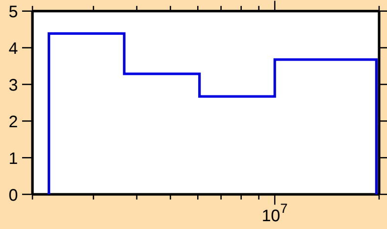
\Delta\sigma/\sigma vs. E for ^{122}\text{Te}(\text{n},\text{tot.})
