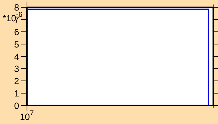
\sigma vs. E for ^{122}\text{Te}(n,t)
