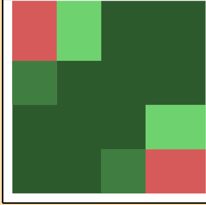
\sigma vs. E for ^{122}\text{Te}(n,n\text{cont.})
