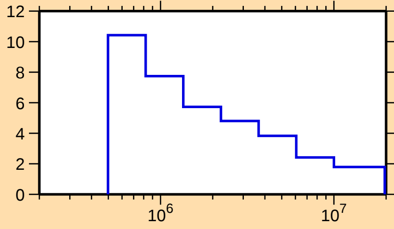
\Delta\sigma/\sigma vs. E for ^{122}\text{Te}(\text{n,nonel.})
