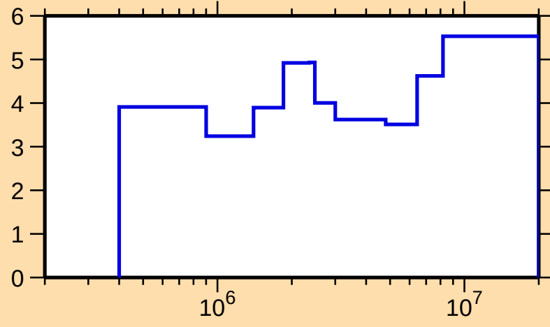
\Delta\sigma/\sigma vs. E for ^{122}\text{Te}(\text{n,el.})
