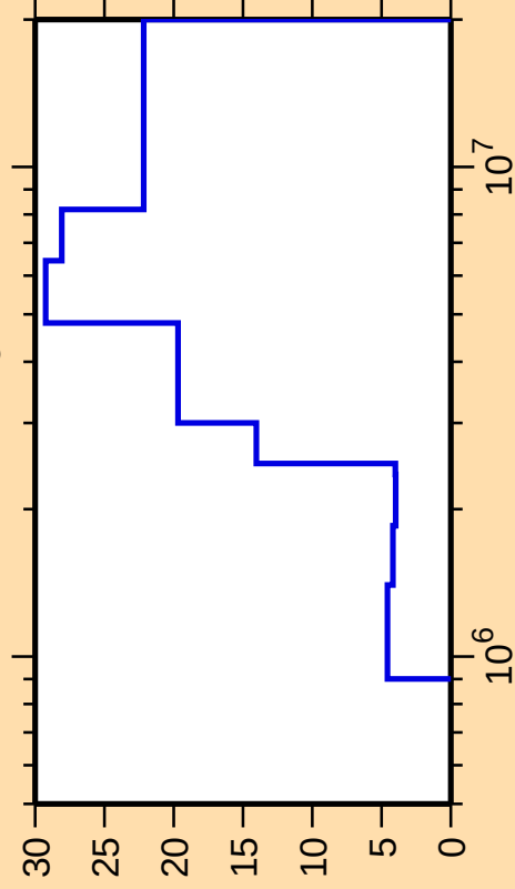
\Delta\sigma/\sigma vs. E for ^{122}\text{Te}(n,n_3)
