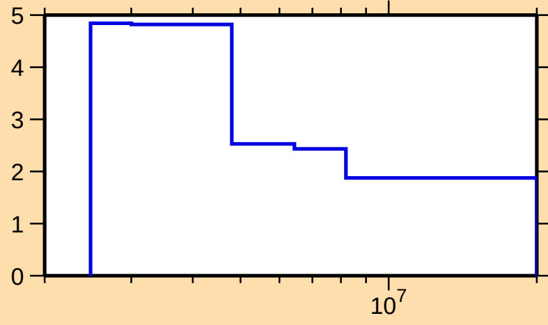
\Delta\sigma/\sigma vs. E for ^{122}\text{Te}(\text{n},\text{nonel.})
