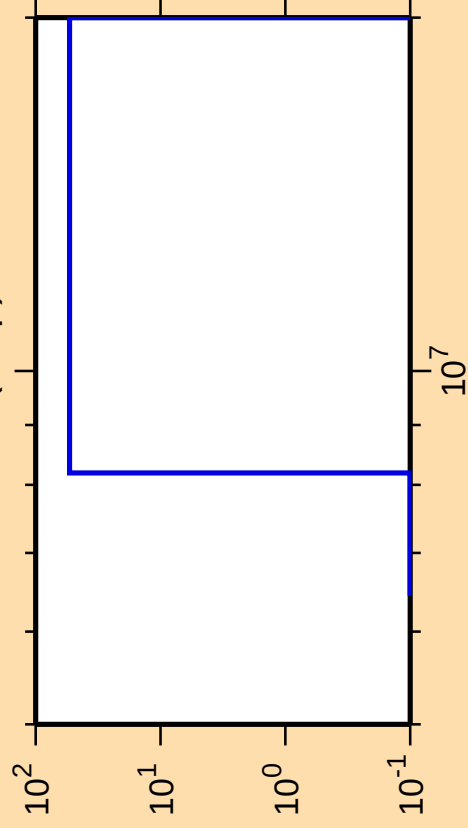
\Delta\sigma/\sigma vs. E for ^{122}\text{Te}(n,np)
