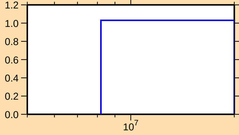
\sigma vs. E for ^{122}\text{Te}(n,2n)
