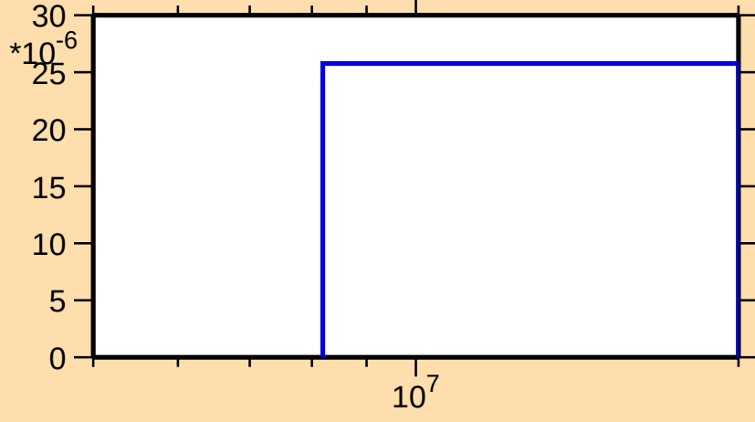
\sigma vs. E for ^{122}\text{Te}(n,3n)
