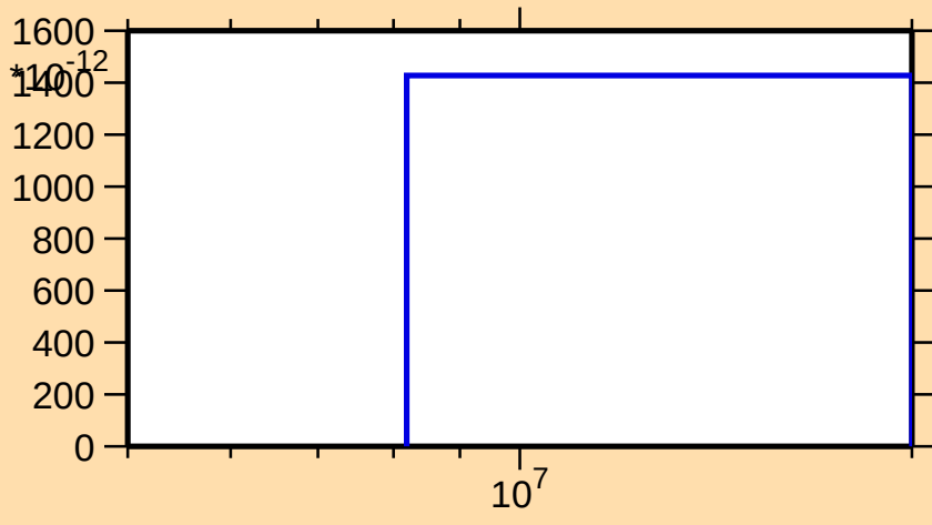
\sigma vs. E for ^{122}\text{Te}(n,\text{He}3)
