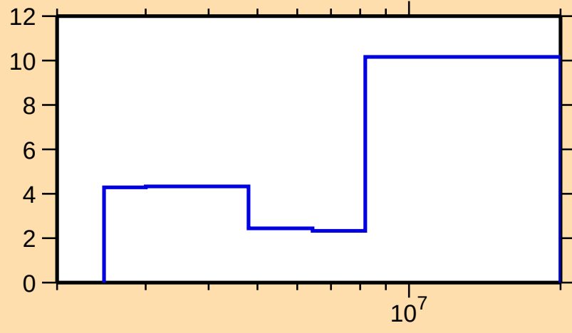
\Delta\sigma/\sigma vs. E for ^{122}\text{Te}(\text{n},\text{inel.})
