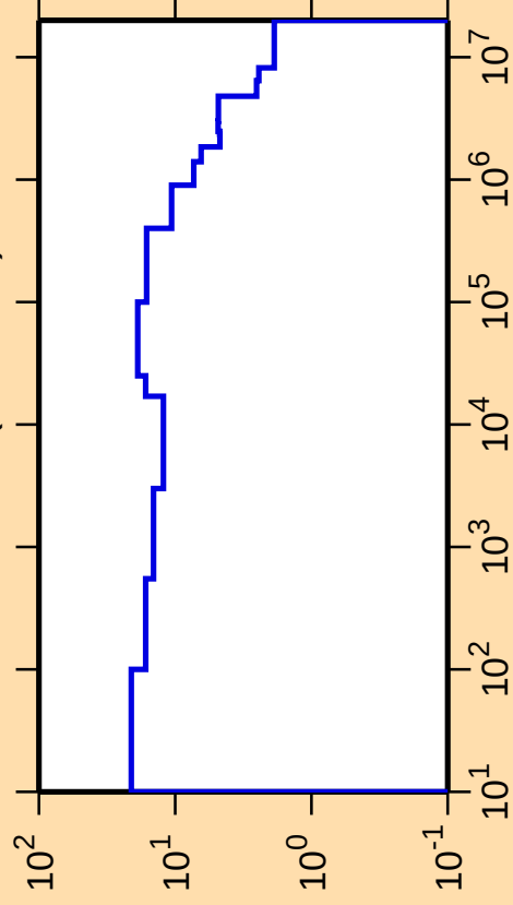
\Delta\sigma/\sigma vs. E for ^{122}\text{Te}(n,\text{nonel.})
