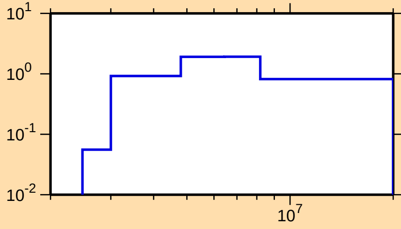
\sigma vs. E for ^{122}\text{Te}(\text{n},\text{ncont.})
