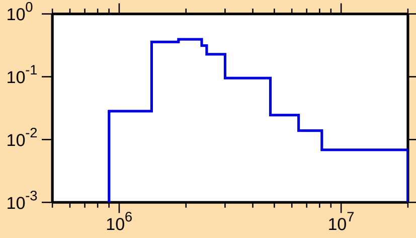
\sigma vs. E for ^{122}\text{Te}(n,n_3)
