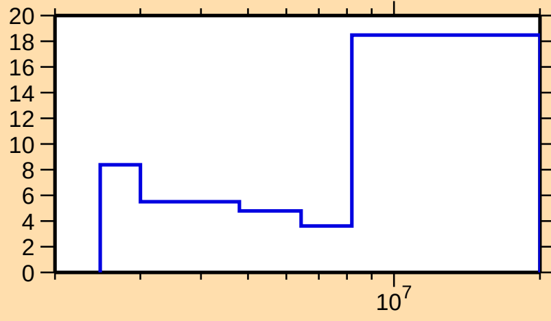
\Delta\sigma/\sigma vs. E for ^{122}\text{Te}(n,n\text{cont.})
