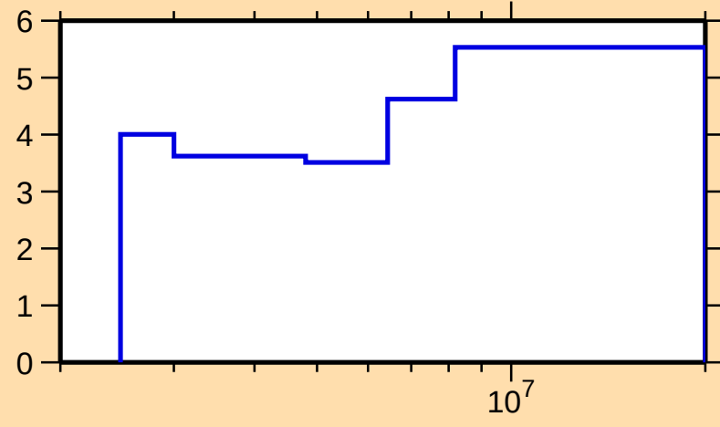
\Delta\sigma/\sigma vs. E for ^{122}\text{Te}(\text{n},\text{el.})
