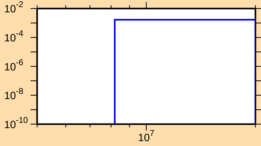
\sigma vs. E for ^{122}\text{Te}(n,np)
