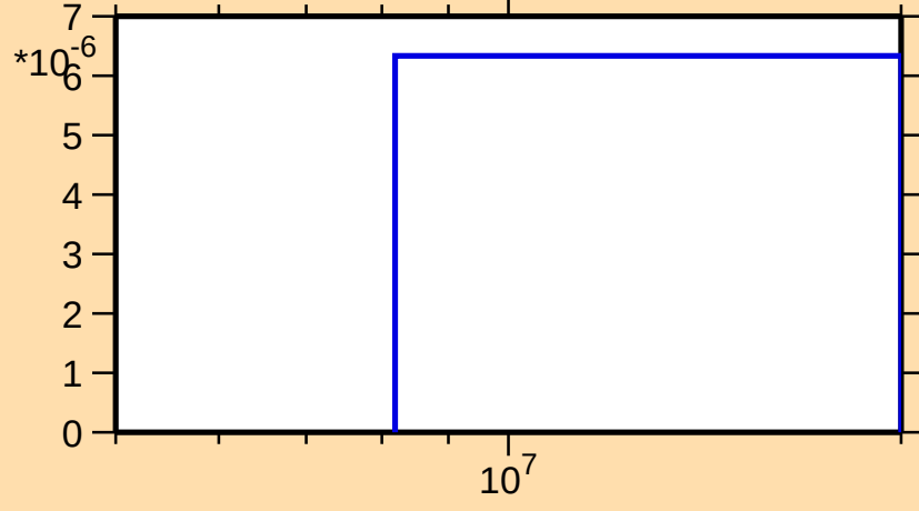
\sigma vs. E for ^{122}\text{Te}(n,t)
