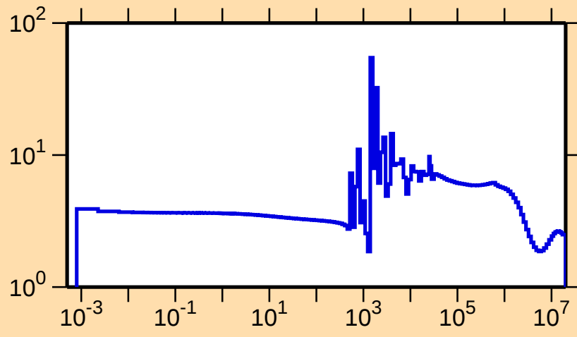
\sigma vs. E for ^{124}\text{Te}(\text{n},\text{el.})
