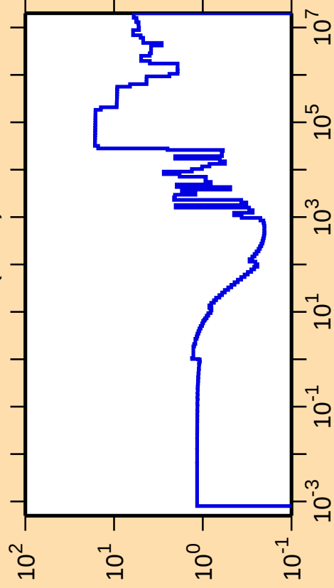
\Delta\sigma/\sigma vs. E for ^{124}\text{Te}(\text{n},\text{el.})
