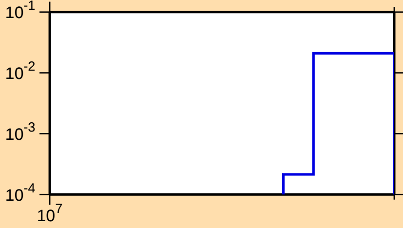
\sigma vs. E for ^{124}\text{Te}(n,3n)
