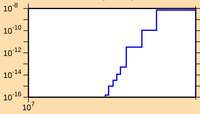
\sigma vs. E for ^{124}\text{Te}(n,\text{He3})
