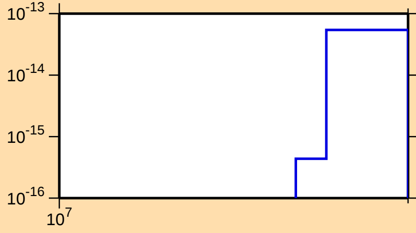
\sigma vs. E for ^{124}\text{Te}(n,p\alpha)
