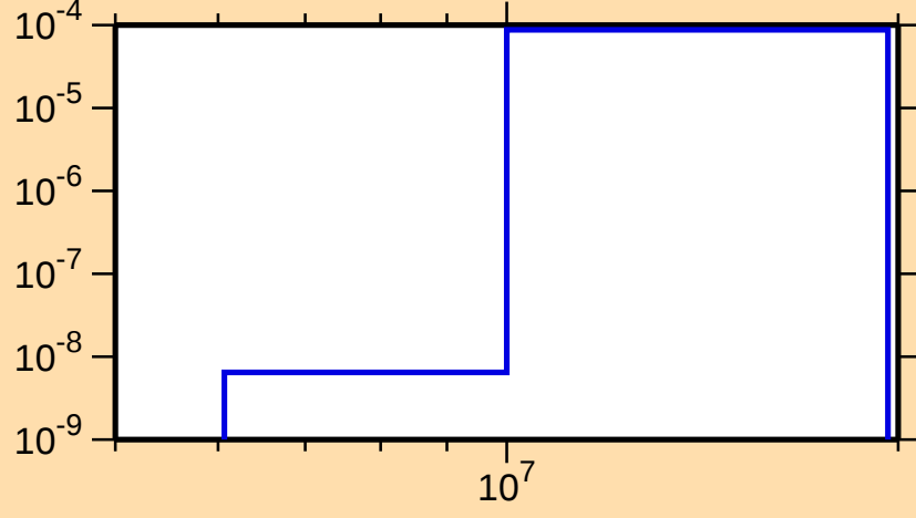
\sigma vs. E for ^{124}\text{Te}(n,n\alpha)
