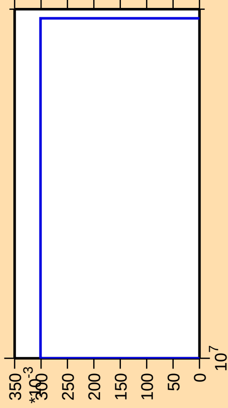
\Delta\sigma/\sigma vs. E for ^{124}\text{Te}(n,nt)
