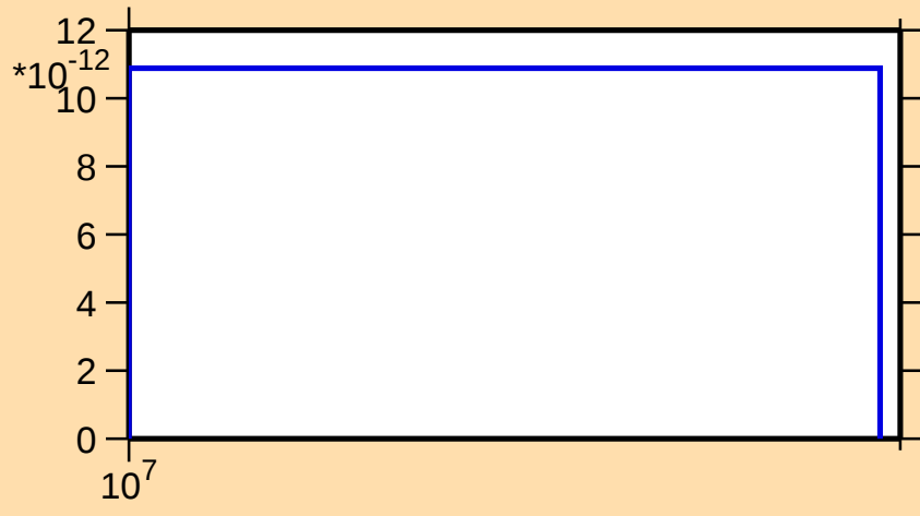
\sigma vs. E for ^{124}\text{Te}(n,2n\alpha)
