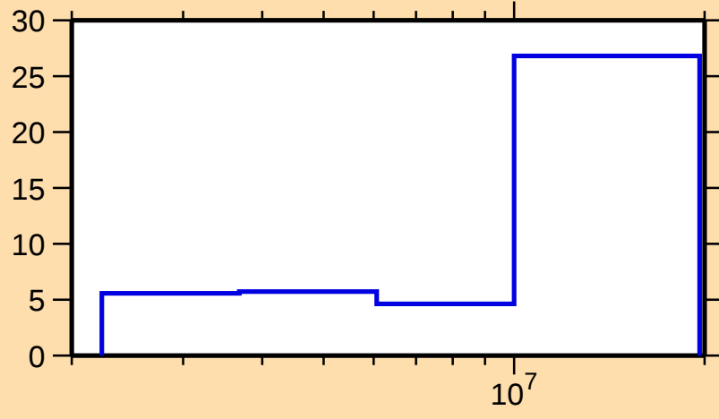
\Delta\sigma/\sigma vs. E for ^{124}\text{Te}(\text{n},\text{inel.})
