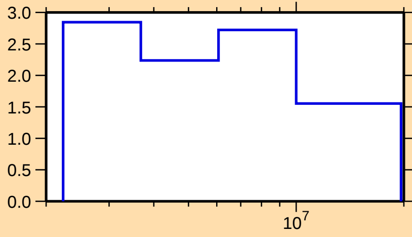
\Delta\sigma/\sigma vs. E for ^{124}\text{Te}(\text{n},\text{tot.})
