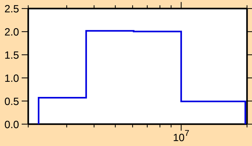
\sigma vs. E for ^{124}\text{Te}(\text{n},\text{ncont.})
