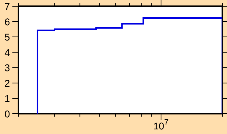
\Delta\sigma/\sigma vs. E for ^{124}\text{Te}(\text{n},\text{nonel.})
