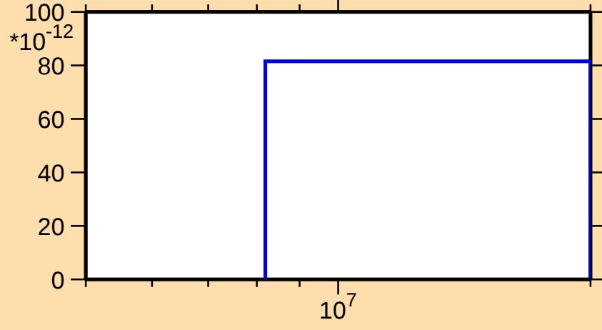
\sigma vs. E for ^{124}\text{Te}(\text{n},\text{nd})
