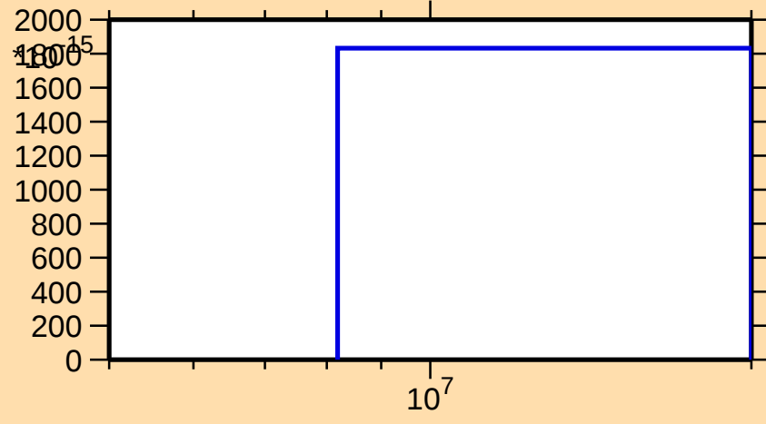
\sigma vs. E for ^{124}\text{Te}(n,nt)
