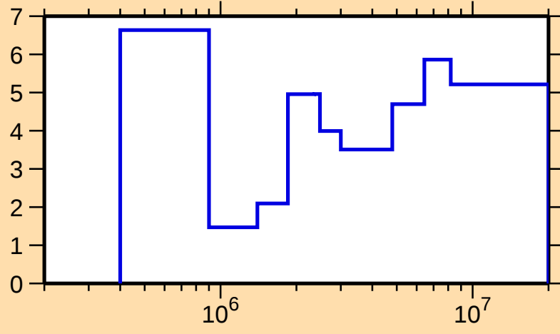
\Delta\sigma/\sigma vs. E for ^{124}\text{Te}(\text{n,el.})
