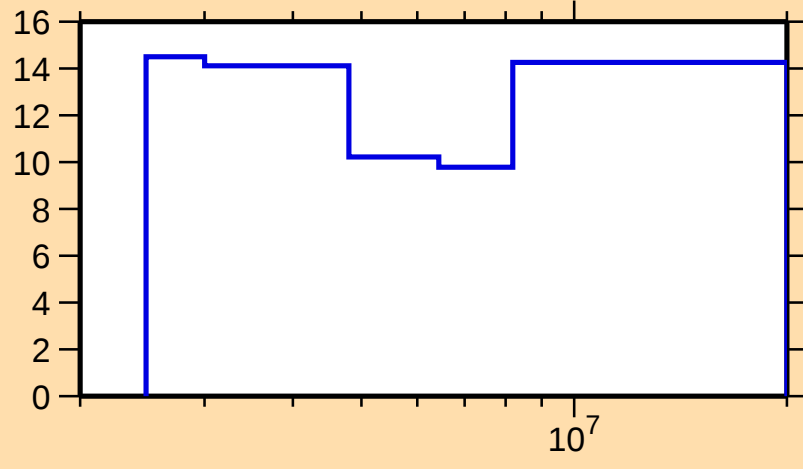
\Delta\sigma/\sigma vs. E for ^{124}\text{Te}(n,n\text{cont.})
