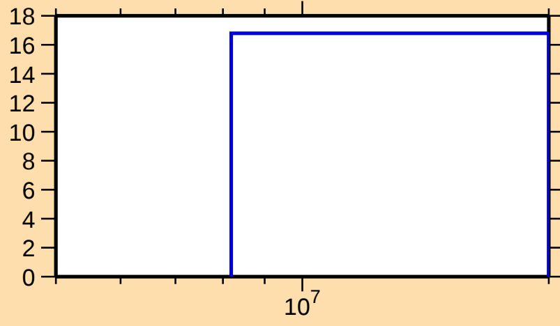
\Delta\sigma/\sigma vs. E for ^{124}\text{Te}(n,\text{inel.})
