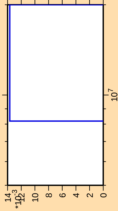
\Delta\sigma/\sigma vs. E for ^{124}\text{Te}(n,\text{pd})
