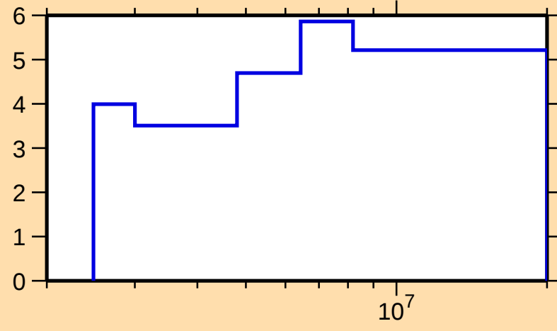
\Delta\sigma/\sigma vs. E for ^{124}\text{Te}(\text{n},\text{el.})
