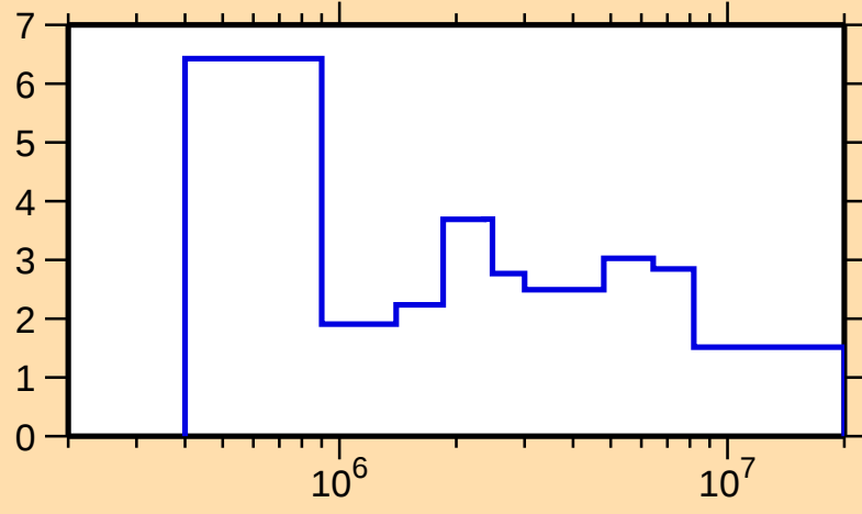
\Delta\sigma/\sigma vs. E for ^{124}\text{Te}(\text{n,tot.})
