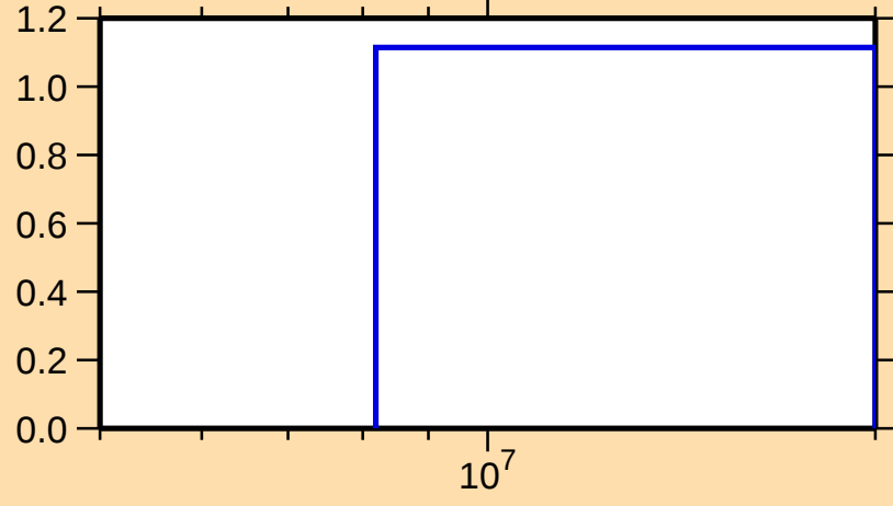
\sigma vs. E for ^{124}\text{Te}(n,2n)
