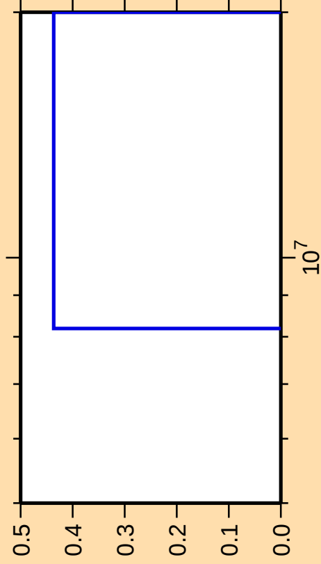
\Delta\sigma/\sigma vs. E for ^{124}\text{Te}(n,nt)
