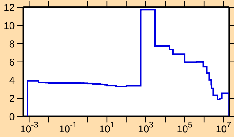
\sigma vs. E for ^{124}\text{Te}(n,\text{el.})
