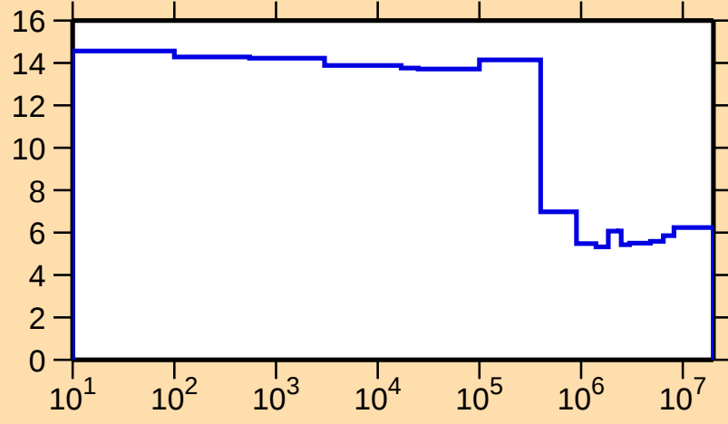
\Delta\sigma/\sigma vs. E for ^{124}\text{Te}(n,\text{nonel.})
