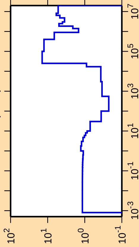
\Delta\sigma/\sigma vs. E for ^{124}\text{Te}(n,\text{el.})
