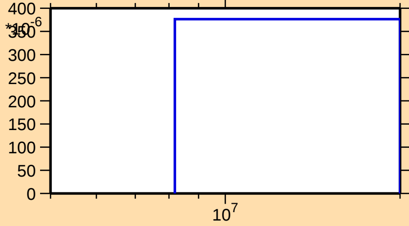
\sigma vs. E for ^{124}\text{Te}(n,np)
