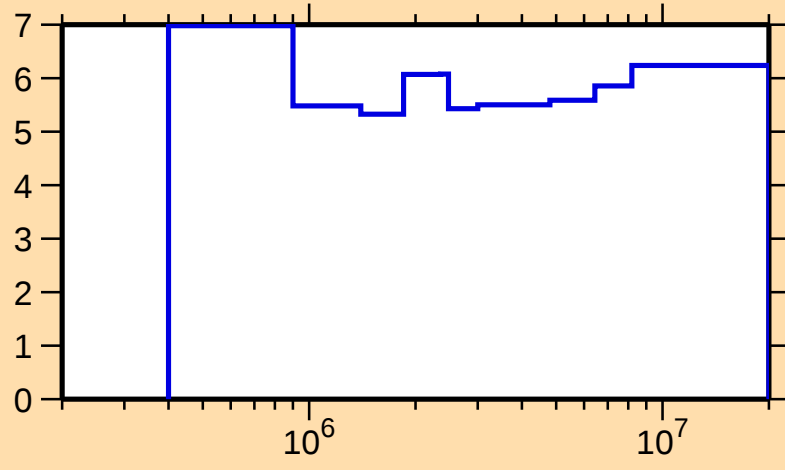
\Delta\sigma/\sigma vs. E for ^{124}\text{Te}(\text{n,nonel.})
