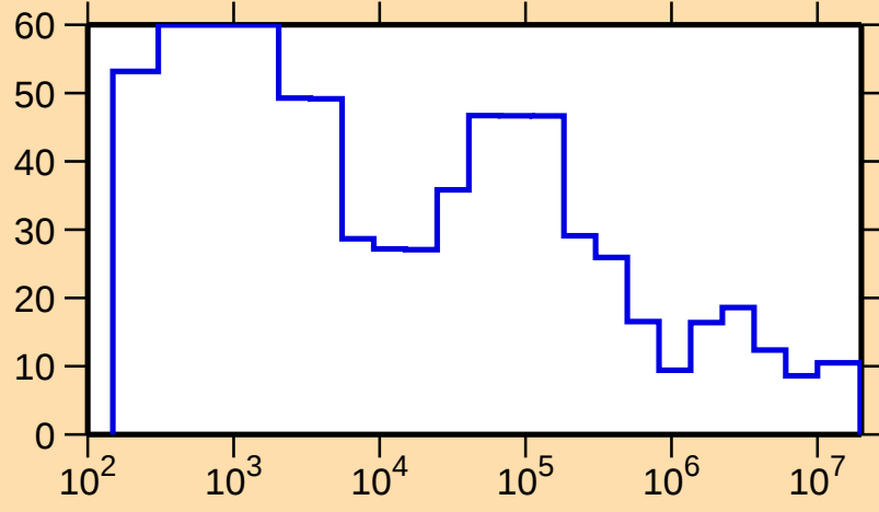
\Delta\sigma/\sigma vs. E for ^{125}\text{Te}(\text{n,el.})
