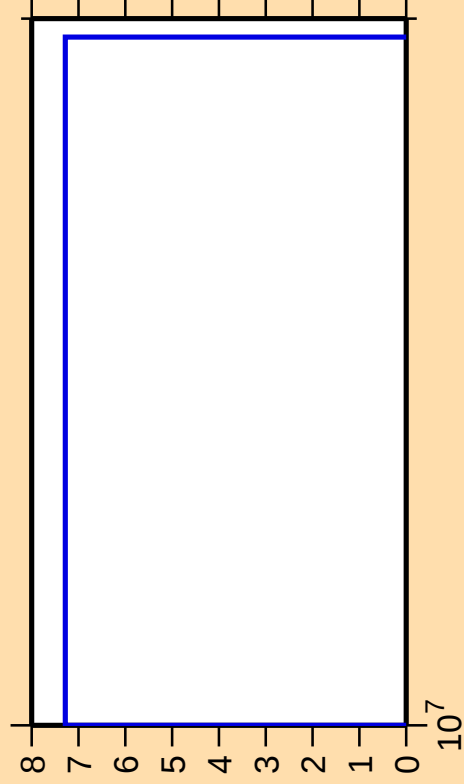
\Delta\sigma/\sigma vs. E for ^{125}\text{Te}(n,\text{nt})
