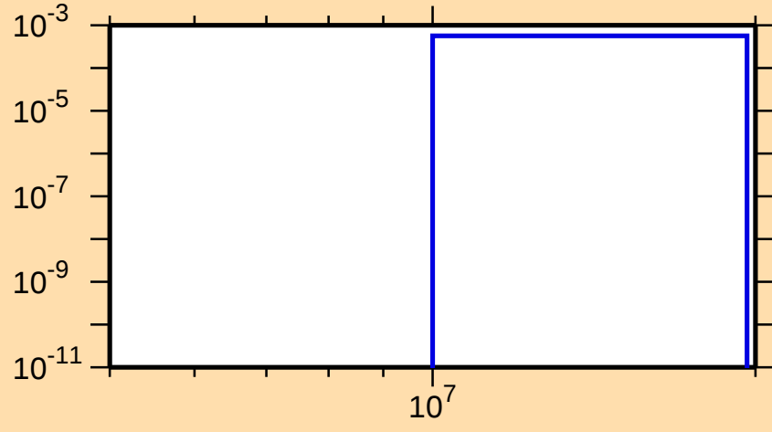
\sigma vs. E for ^{125}\text{Te}(n,np)
