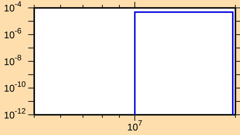
\sigma vs. E for ^{125}\text{Te}(n,t)
