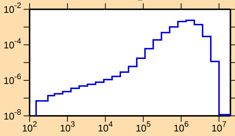
\sigma vs. E for ^{125}\text{Te}(n,n_1)
