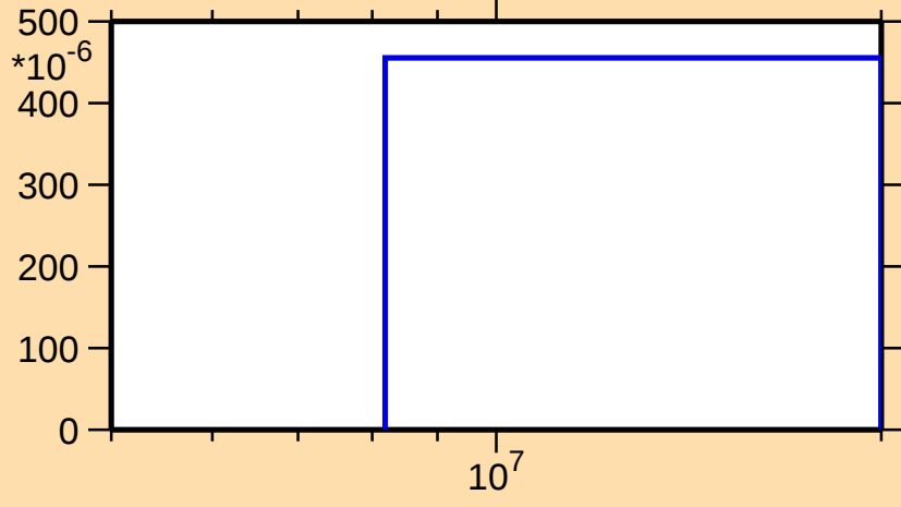
\sigma vs. E for ^{125}\text{Te}(n,np)
