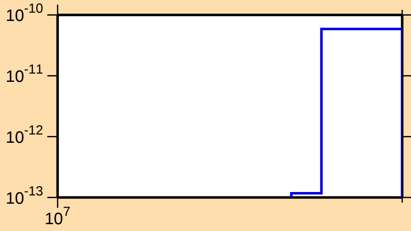
\sigma vs. E for ^{127}\text{Te}(n,\text{He3})
