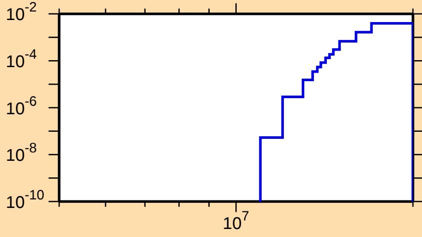
\sigma vs. E for ^{127}\text{Te}(n,np)
