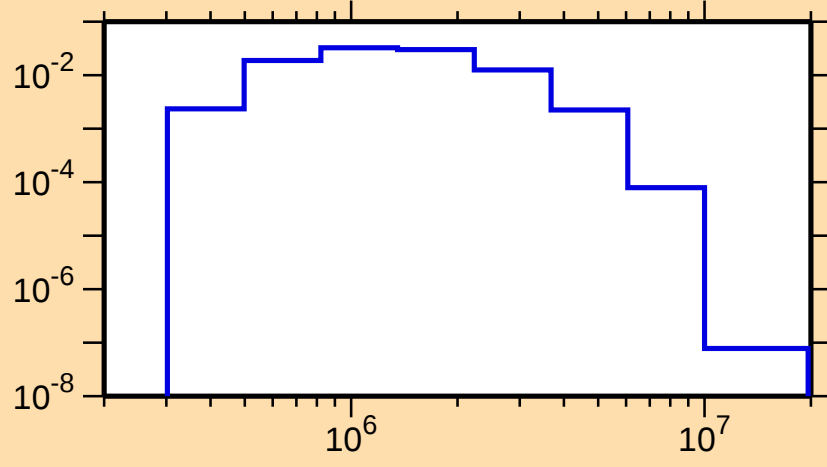
\sigma vs. E for ^{127}\text{Te}(n,n_4)
