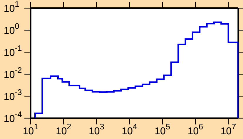
\sigma vs. E for ^{127}\text{Te}(n,\text{inel.})
