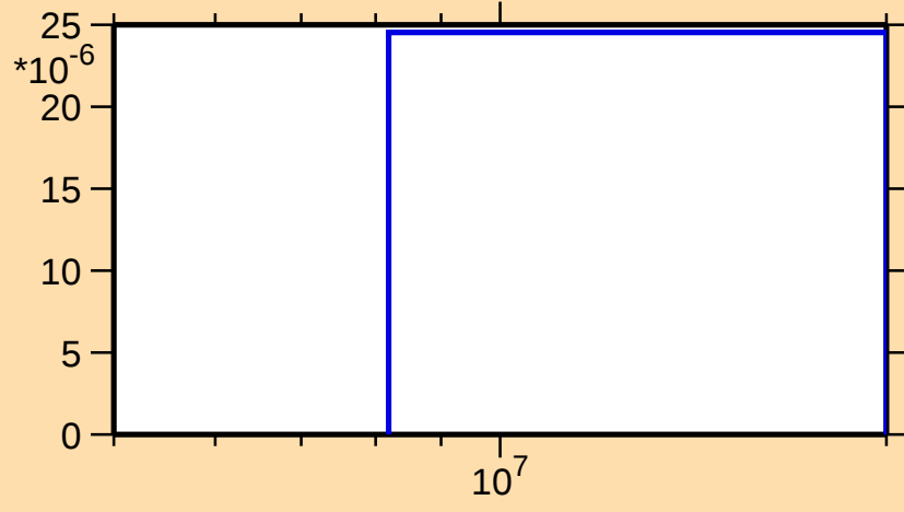
\sigma vs. E for ^{127}\text{Te}(n,t)
