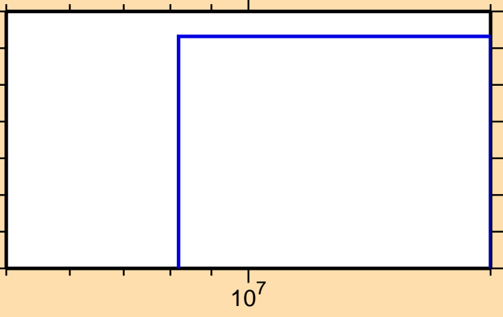
\sigma vs. E for ^{131}\text{Te}(n,\text{nd})
