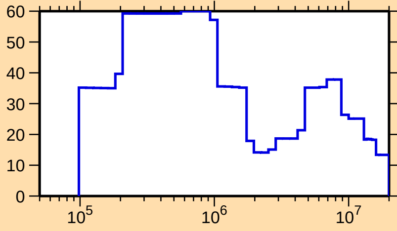
\Delta\sigma/\sigma vs. E for ^{224}\text{Th}(n,\text{el.})
