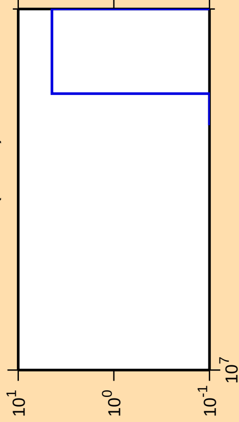
\Delta\sigma/\sigma vs. E for ^{224}\text{Th}(\text{mt } 34)
