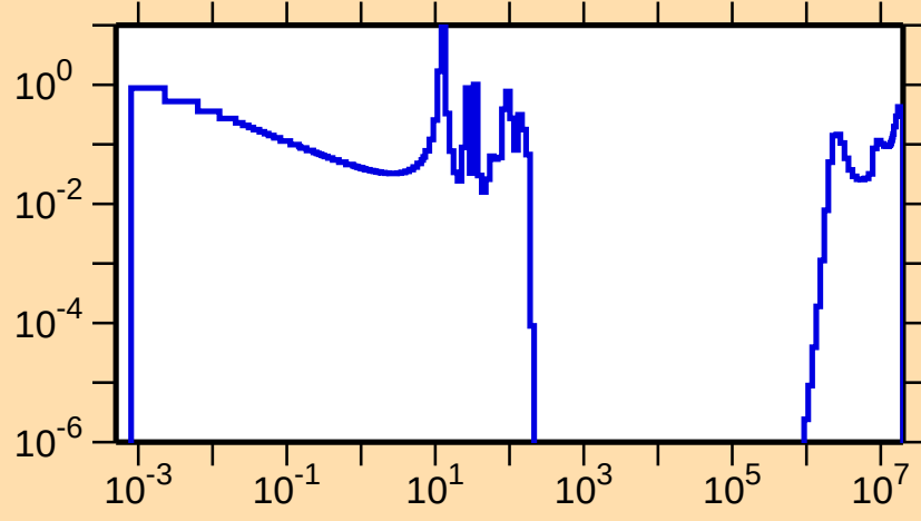
\sigma vs. E for ^{224}\text{Th}(n,f)
