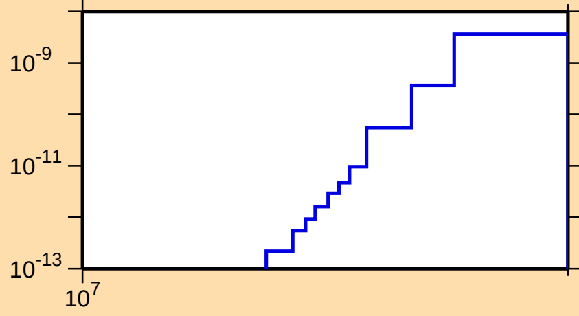
\sigma vs. E for ^{224}\text{Th}(n,\text{He3})
