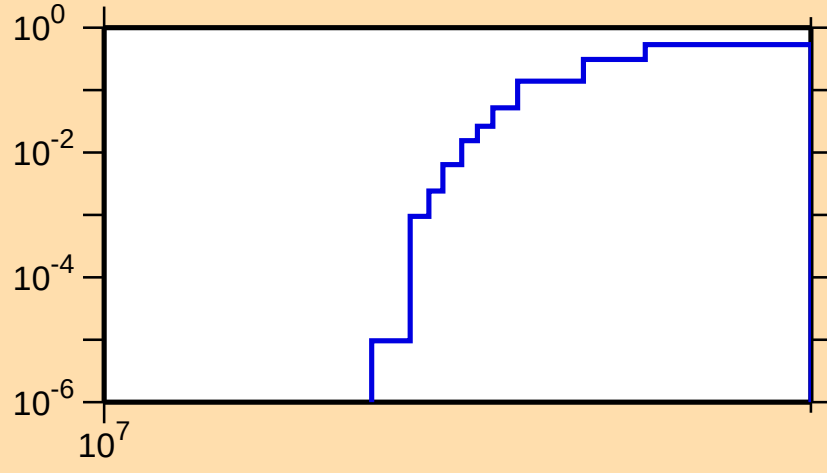
\sigma vs. E for ^{224}\text{Th}(n,3n)
