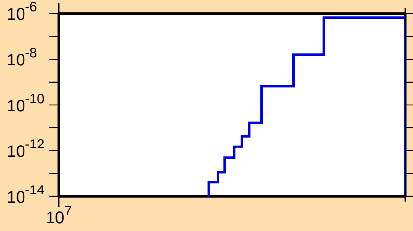
\sigma vs. E for ^{224}\text{Th}(n,\text{nt})
