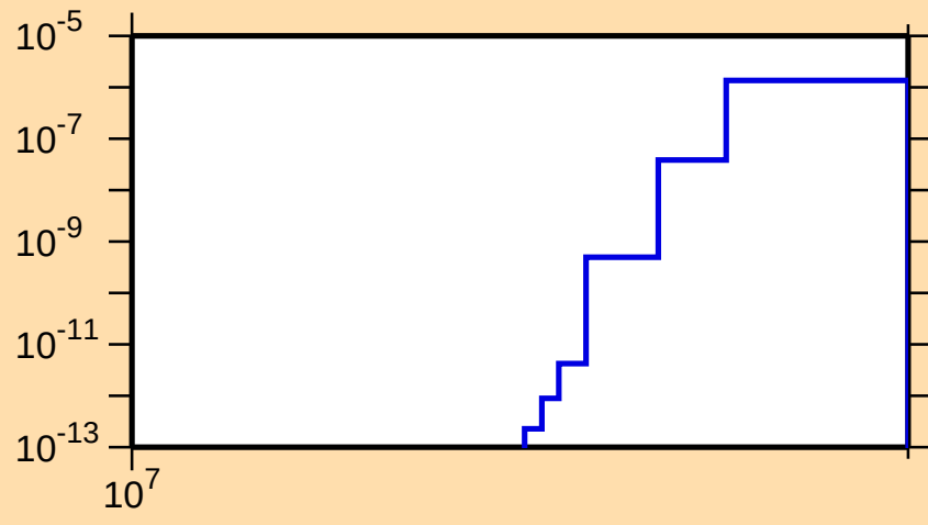
\sigma vs. E for ^{224}\text{Th}(n,2np)
