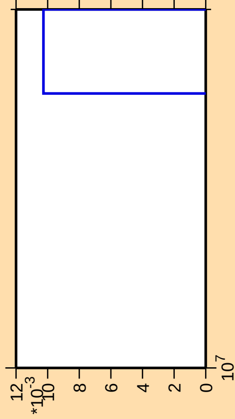
\Delta\sigma/\sigma vs. E for ^{224}\text{Th}(\text{mt } 42)
