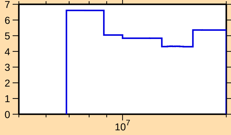
\Delta\sigma/\sigma vs. E for ^{224}\text{Th}(n,\text{nonel.})
