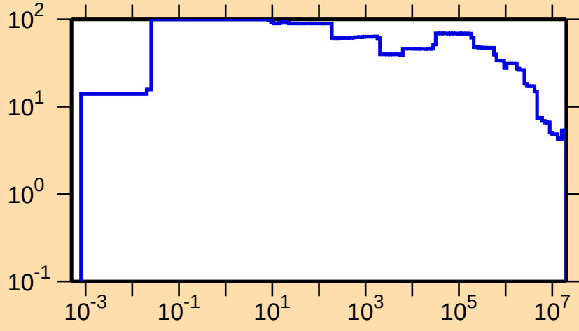
\Delta\sigma/\sigma vs. E for ^{224}\text{Th}(n,\text{nonel.})
