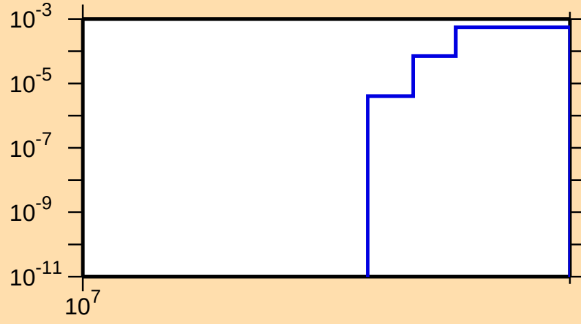
\sigma vs. E for ^{224}\text{Th}(n,3n\alpha)
