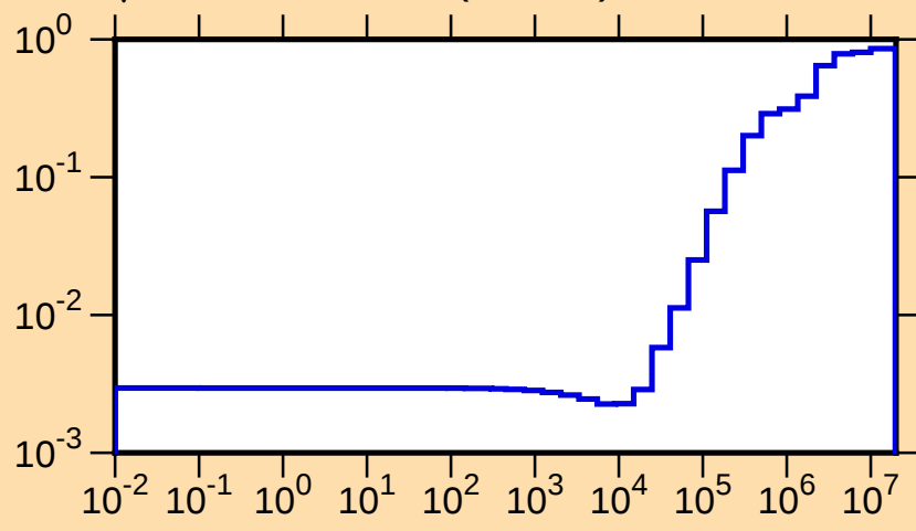
\mu vs. E for ^{224}\text{Th}(\text{mt251})
