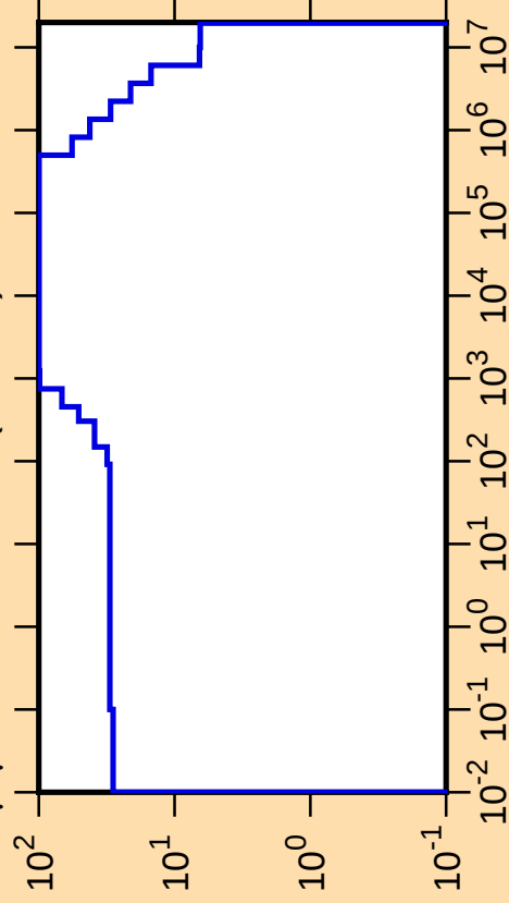
\Delta\mu/\mu vs. E for ^{224}\text{Th}(\text{mt251})
