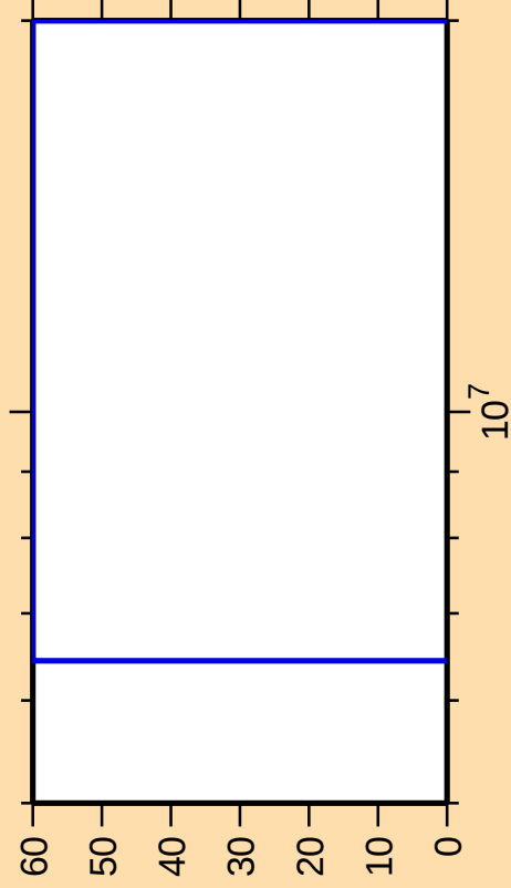
\Delta\sigma/\sigma vs. E for ^{224}\text{Th}(n,f)
