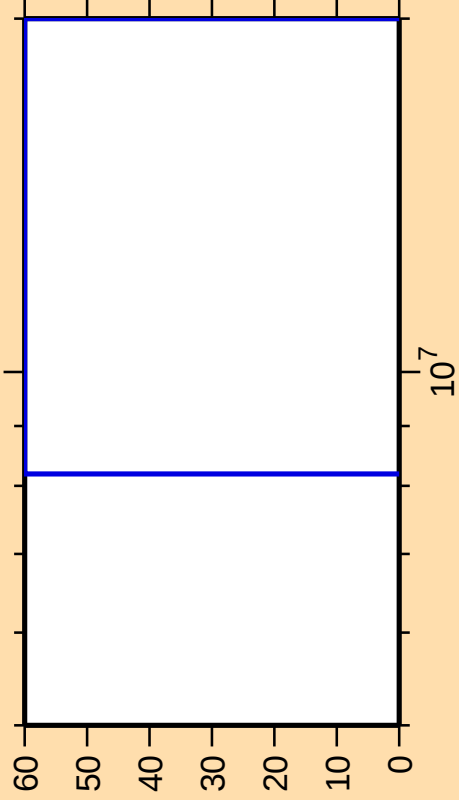
\Delta\sigma/\sigma vs. E for ^{224}\text{Th}(n,p\alpha)
