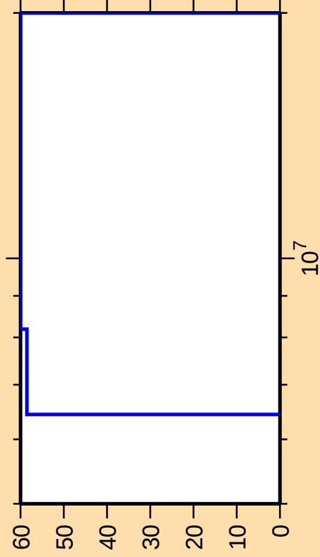
\Delta\sigma/\sigma vs. E for ^{224}\text{Th}(n,n\text{cont.})
