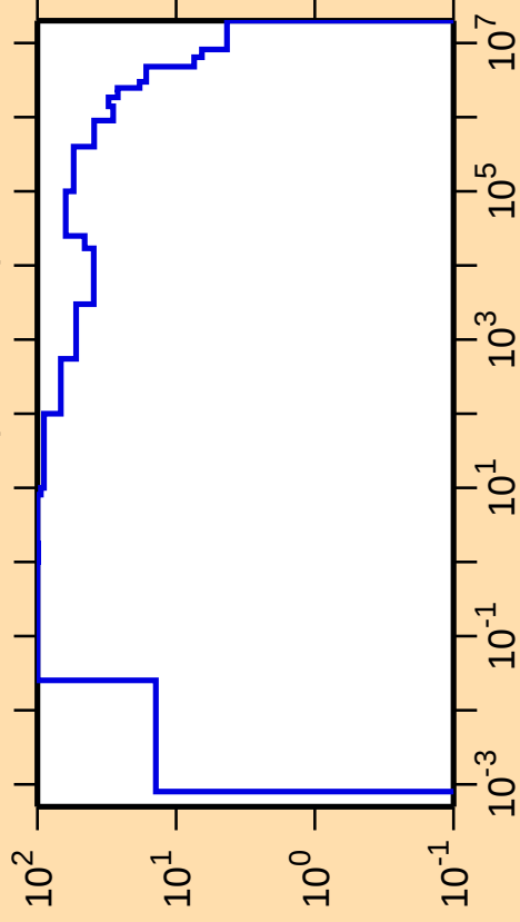
\Delta\sigma/\sigma vs. E for ^{224}\text{Th}(n,\text{nonel.})
