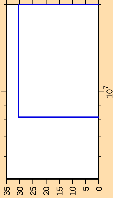
\Delta\sigma/\sigma vs. E for ^{224}\text{Th}(\text{mt } 45)
