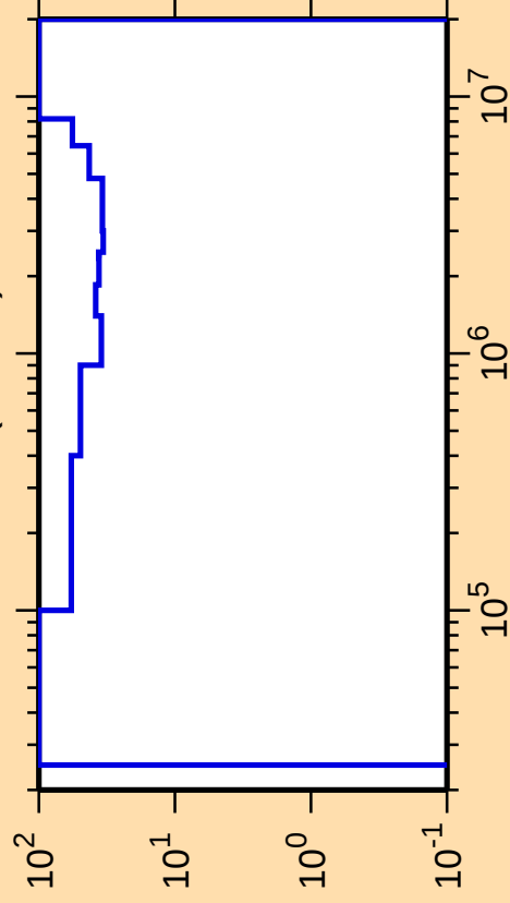
\Delta\sigma/\sigma vs. E for ^{224}\text{Th}(n,\text{inel.})
