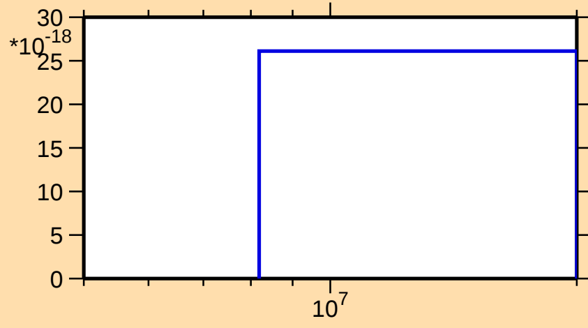
\sigma vs. E for ^{224}\text{Th}(\text{mt } 42)
