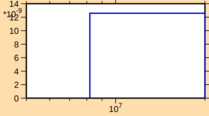
\sigma vs. E for ^{224}\text{Th}(n,2np)
