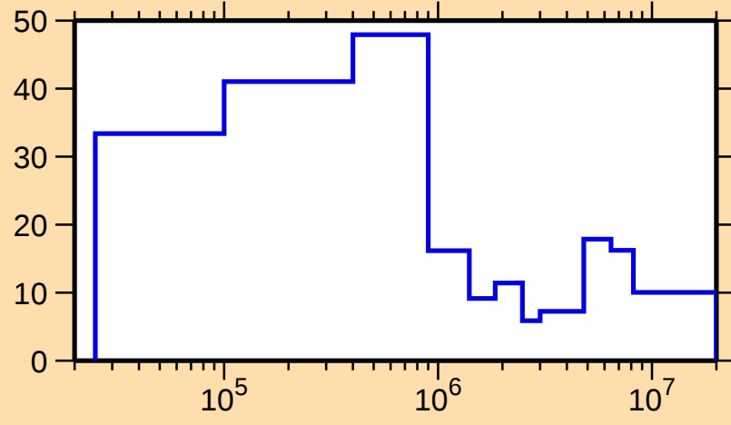
\Delta\sigma/\sigma vs. E for ^{224}\text{Th}(n,\text{tot.})
