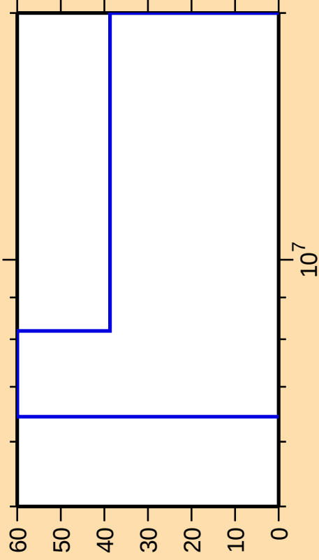
\Delta\sigma/\sigma vs. E for ^{224}\text{Th}(n,p)
