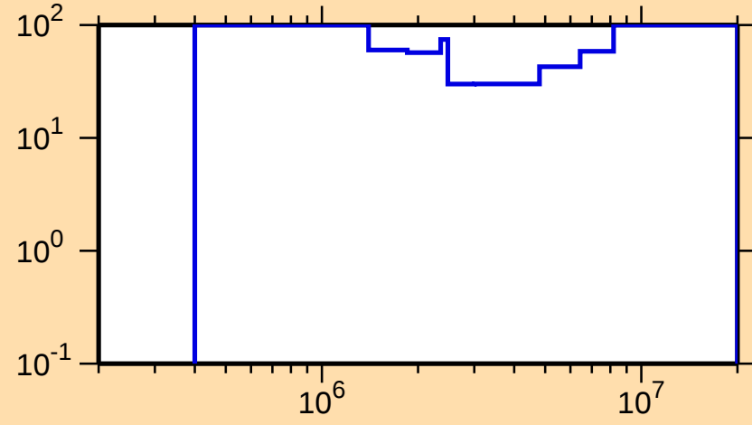
\Delta\sigma/\sigma vs. E for ^{224}\text{Th}(n,n\text{cont.})
