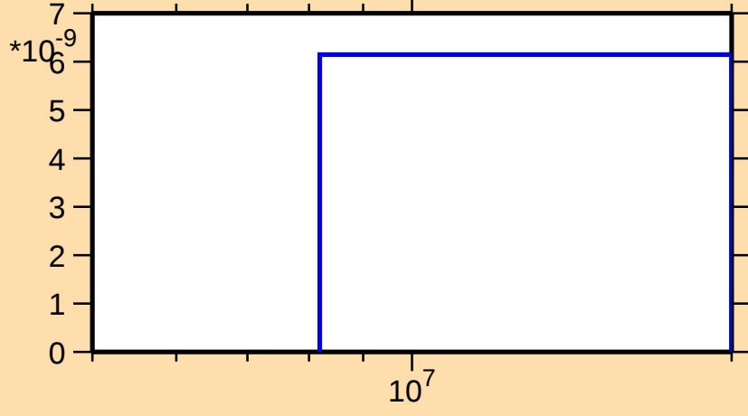
\sigma vs. E for ^{224}\text{Th}(n,\text{nt})
