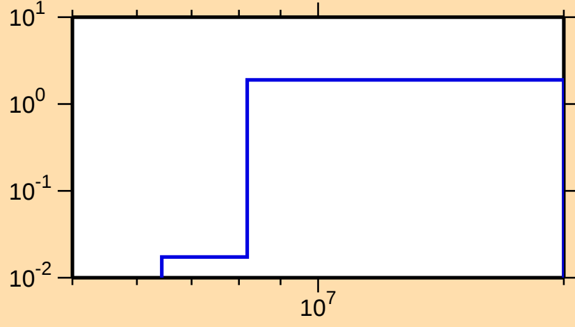
\sigma vs. E for ^{224}\text{Th}(n,2n)
