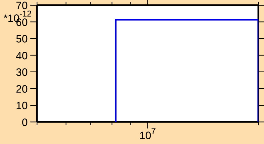
\sigma vs. E for ^{224}\text{Th}(n,p\alpha)
