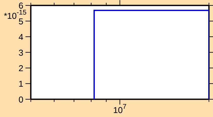
\sigma vs. E for ^{224}\text{Th}(\text{mt } 34)
