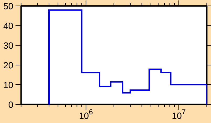
\Delta\sigma/\sigma vs. E for ^{224}\text{Th}(n,\text{tot.})
