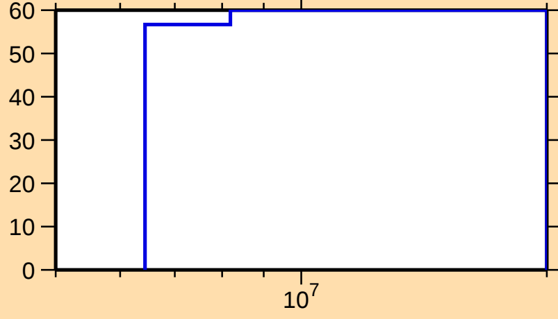
\Delta\sigma/\sigma vs. E for ^{224}\text{Th}(n,\text{inel.})
