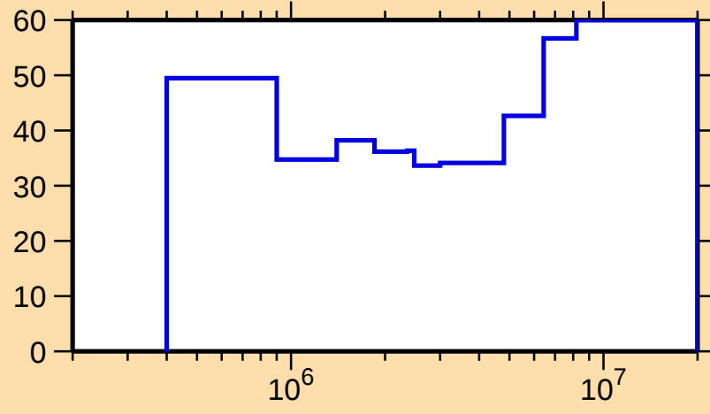
\Delta\sigma/\sigma vs. E for ^{224}\text{Th}(n,\text{inel.})
