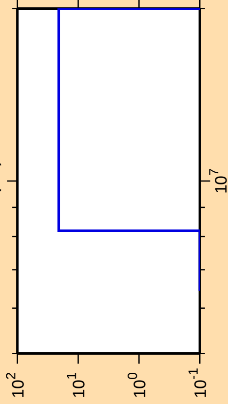
\Delta\sigma/\sigma vs. E for ^{224}\text{Th}(n,t)
