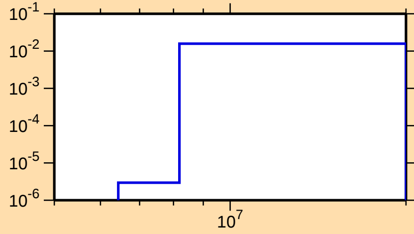
\sigma vs. E for ^{224}\text{Th}(n,2n\alpha)
