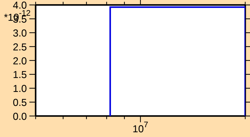
\sigma vs. E for ^{224}\text{Th}(\text{mt } 45)
