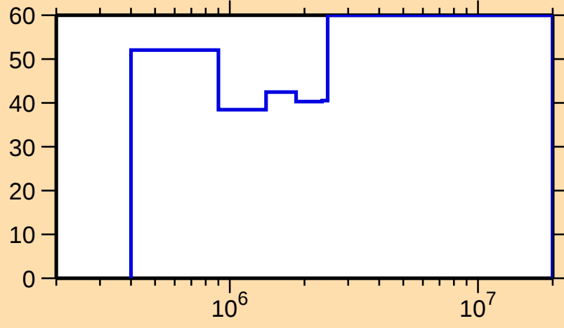
\Delta\sigma/\sigma vs. E for ^{224}\text{Th}(n,n_1)
