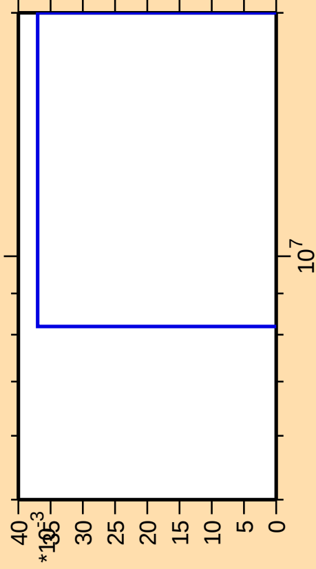
\Delta\sigma/\sigma vs. E for ^{224}\text{Th}(\text{mt } 34)
