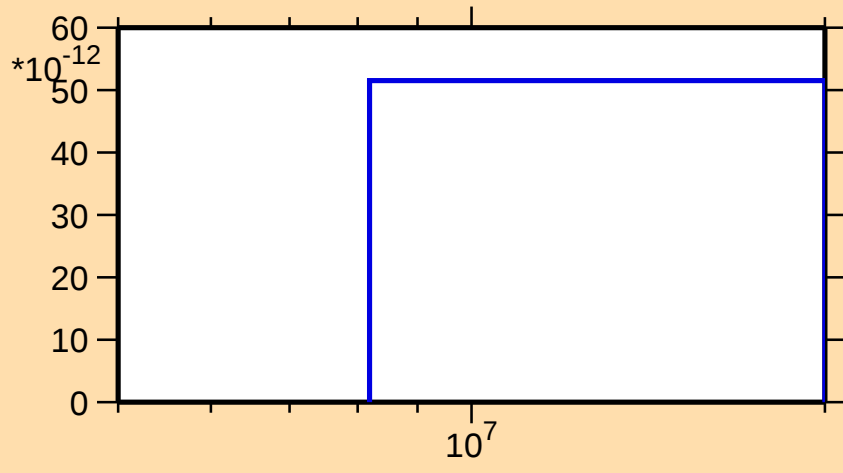
\sigma vs. E for ^{224}\text{Th}(n,\text{He}3)
