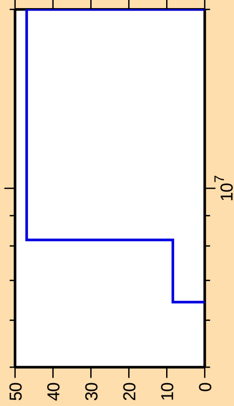
\Delta\sigma/\sigma vs. E for ^{224}\text{Th}(n,np)
