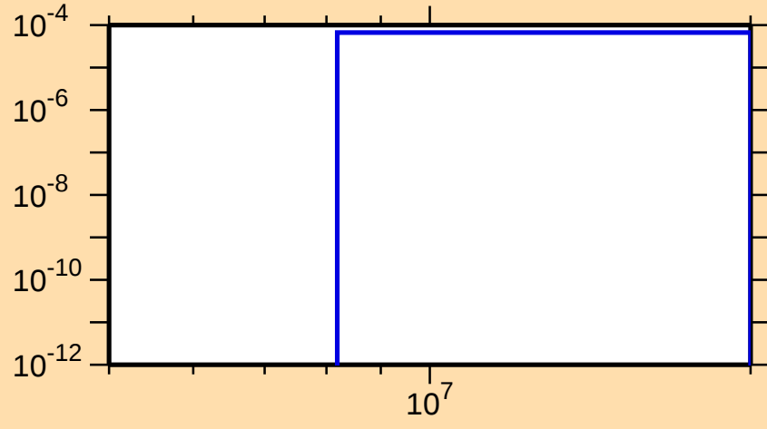
\sigma vs. E for ^{224}\text{Th}(n,t)
