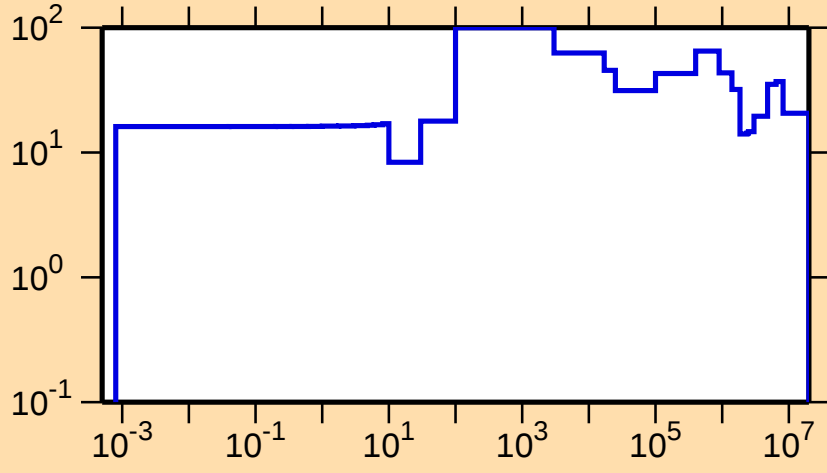
\Delta\sigma/\sigma vs. E for ^{224}\text{Th}(n,\text{el.})
