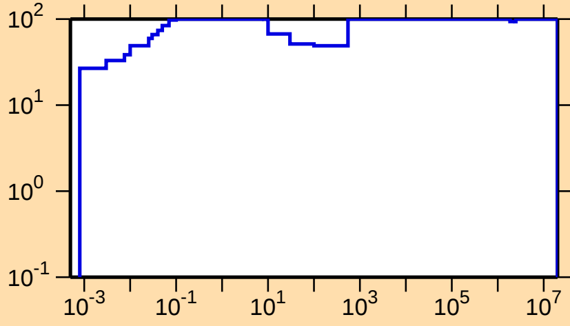
\Delta\sigma/\sigma vs. E for ^{224}\text{Th}(n,f)
