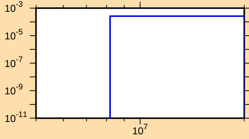
\sigma vs. E for ^{224}\text{Th}(n,np)
