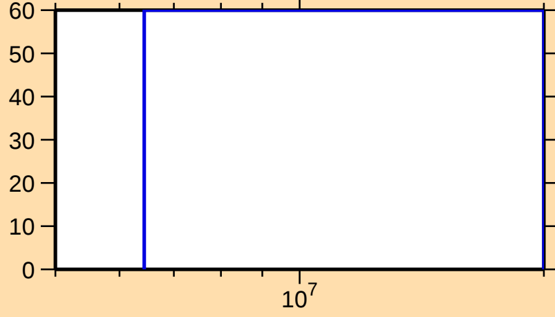
\Delta\sigma/\sigma vs. E for ^{224}\text{Th}(n,2n)
