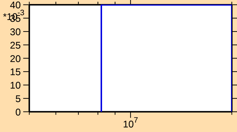
\sigma vs. E for ^{224}\text{Th}(n,3n)
