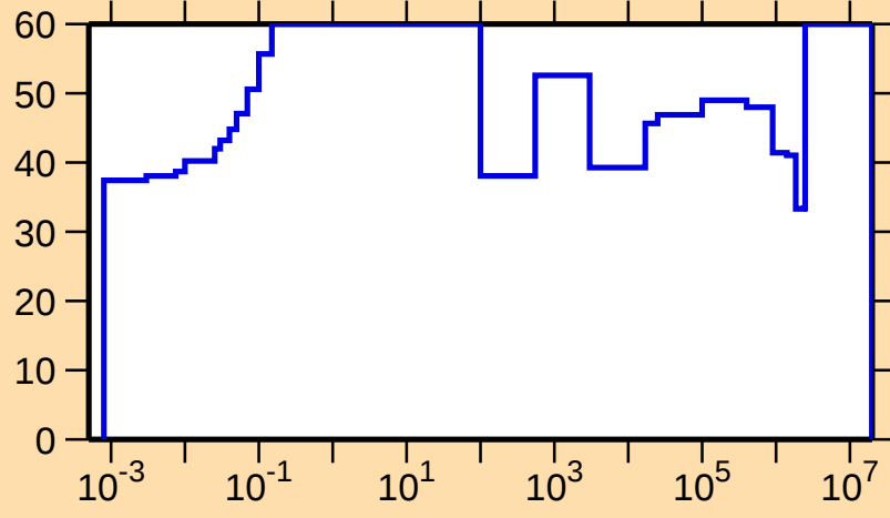
\Delta\sigma/\sigma vs. E for ^{224}\text{Th}(n,\gamma)
