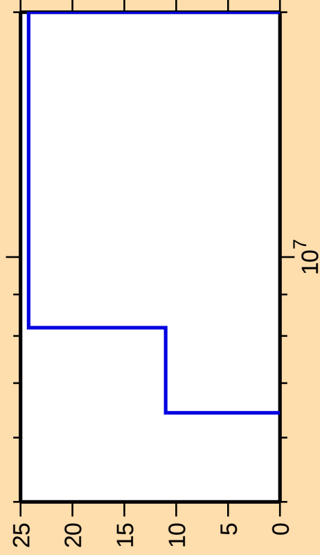
\Delta\sigma/\sigma vs. E for ^{224}\text{Th}(n,d)
