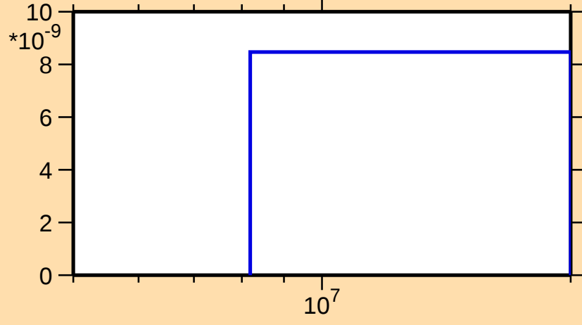
\sigma vs. E for ^{224}\text{Th}(n,\text{nd})
