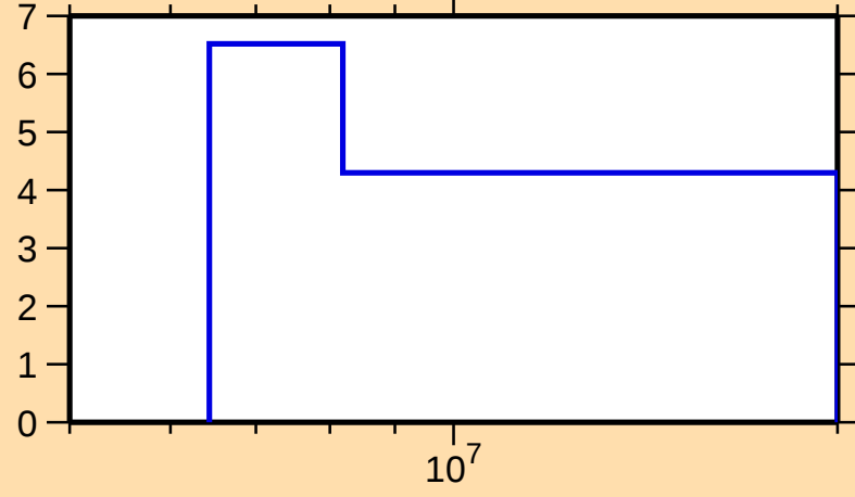
\Delta\sigma/\sigma vs. E for ^{224}\text{Th}(n,\text{nonel.})
