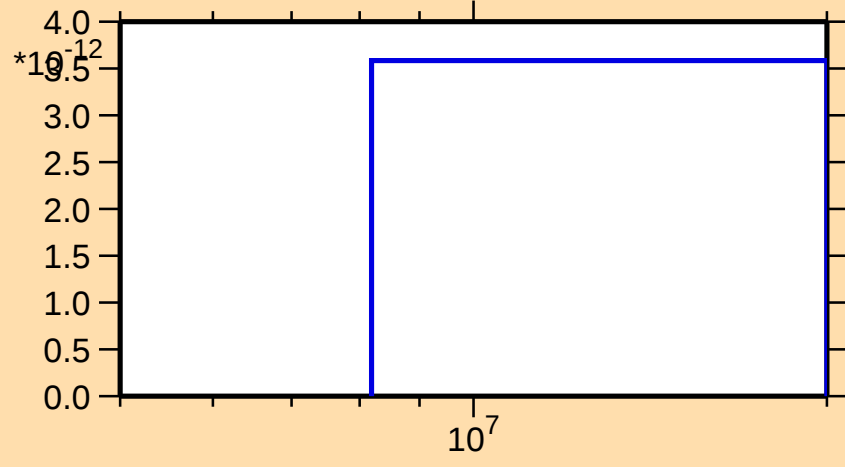
\sigma vs. E for ^{224}\text{Th}(\text{mt117})
