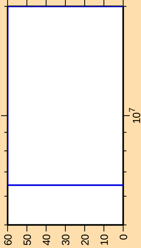
\Delta\sigma/\sigma vs. E for ^{224}\text{Th}(n,n_1)
