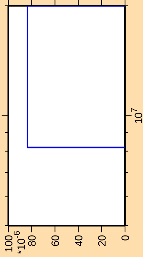
\Delta\sigma/\sigma vs. E for ^{224}\text{Th}(\text{mt } 42)
