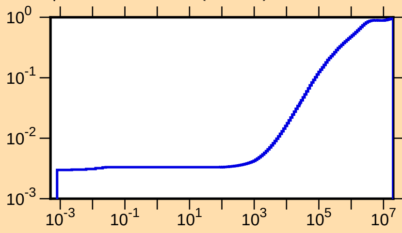
\mu vs. E for ^{227}\text{Th}(\text{mt251})
