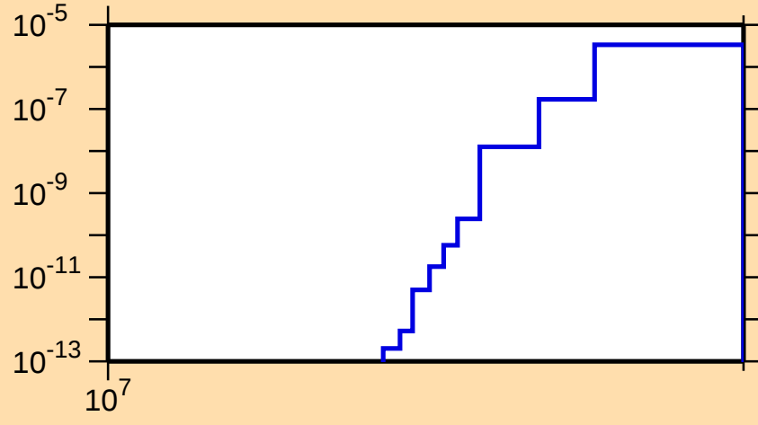
\sigma vs. E for ^{227}\text{Th}(n,2np)
