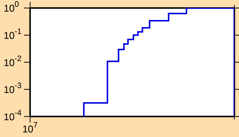
\sigma vs. E for ^{227}\text{Th}(n,3n)
