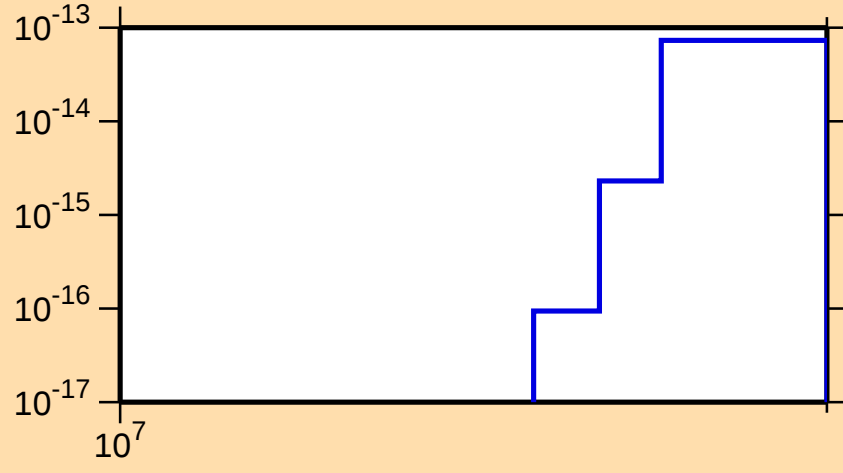
\sigma vs. E for ^{227}\text{Th}(\text{mt } 11)
