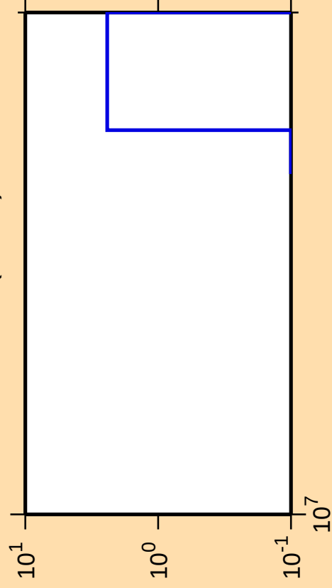
\Delta\sigma/\sigma vs. E for ^{227}\text{Th}(\text{mt } 34)
