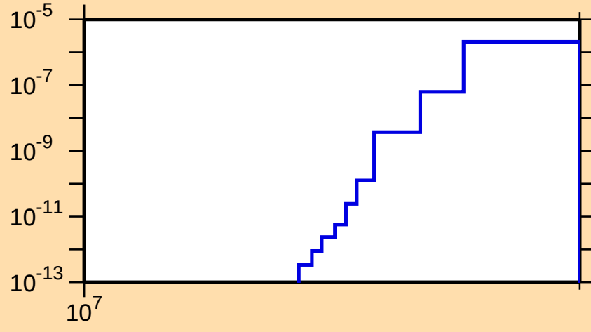
\sigma vs. E for ^{227}\text{Th}(n,\text{nt})
