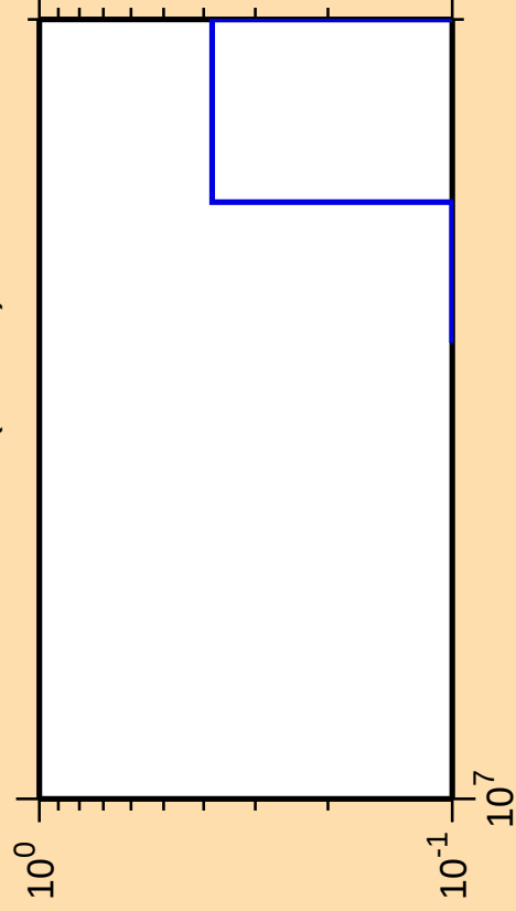
\Delta\sigma/\sigma vs. E for ^{227}\text{Th}(\text{mt } 11)
