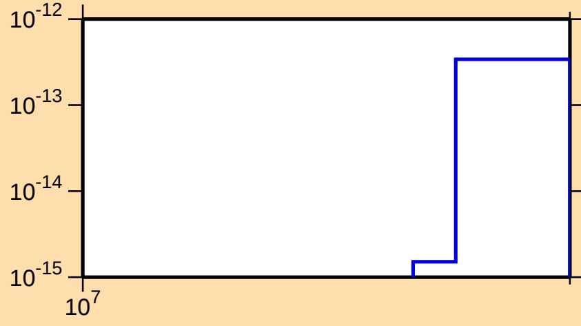
\sigma vs. E for ^{227}\text{Th}(\text{mt } 34)
