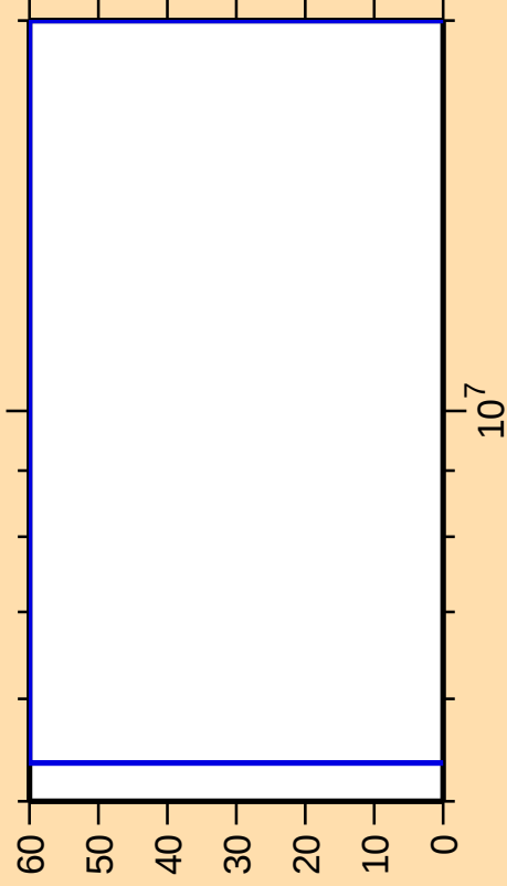
\Delta\sigma/\sigma vs. E for ^{227}\text{Th}(n,\gamma)
