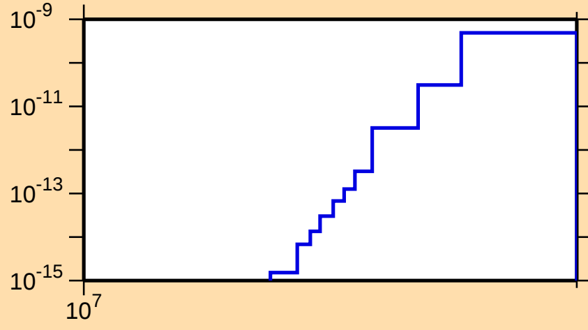
\sigma vs. E for ^{227}\text{Th}(n,\text{He3})
