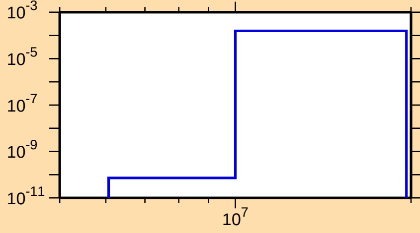
\sigma vs. E for ^{227}\text{Th}(n,np)
