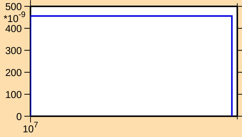
\sigma vs. E for ^{227}\text{Th}(n,3n\alpha)
