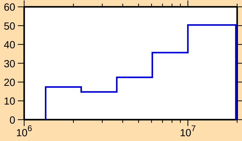
\Delta\sigma/\sigma vs. E for ^{227}\text{Th}(n,\text{inel.})
