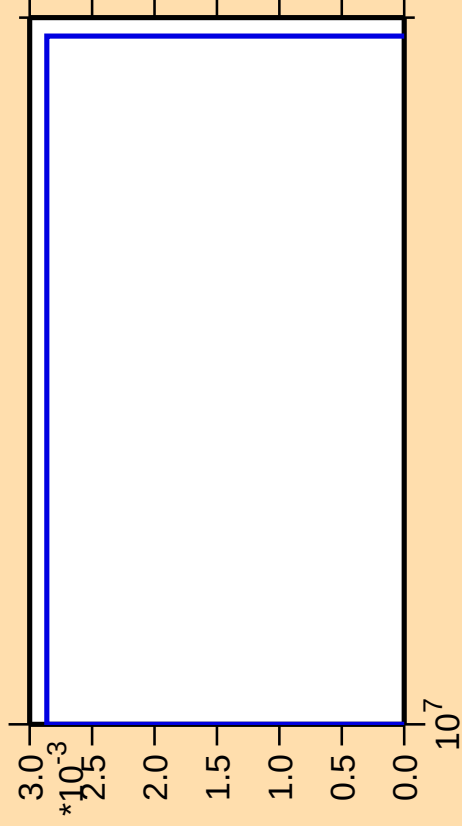
\Delta\sigma/\sigma vs. E for ^{227}\text{Th}(\text{mt } 11)
