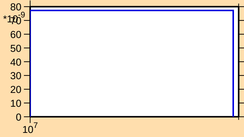
\sigma vs. E for ^{227}\text{Th}(n,\text{nd})
