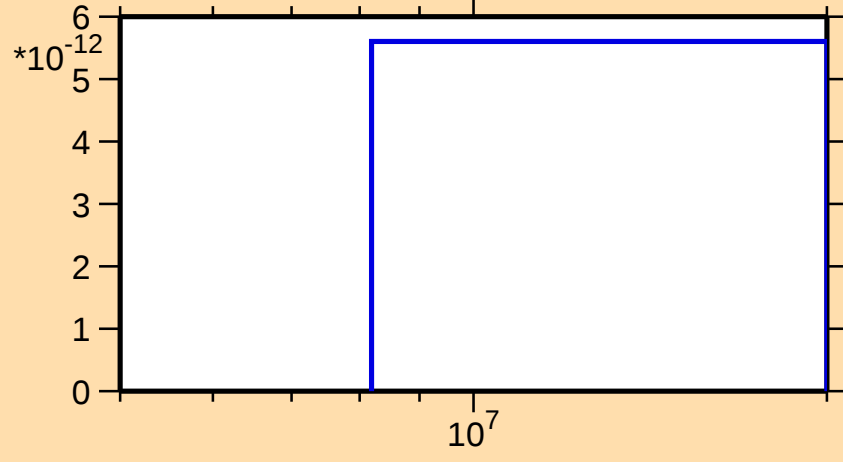
\sigma vs. E for ^{227}\text{Th}(n,\text{He}3)
