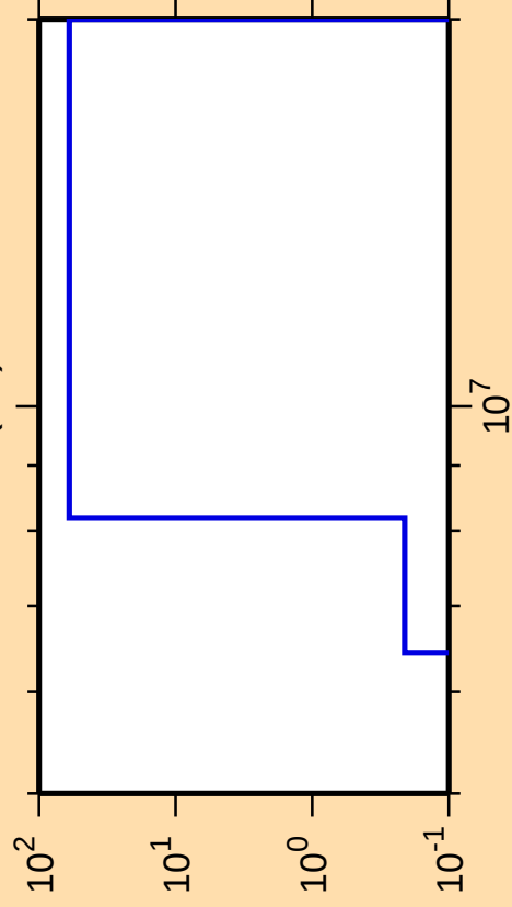
\Delta\sigma/\sigma vs. E for ^{227}\text{Th}(n,t)
