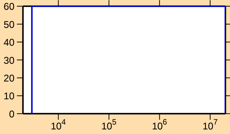
\Delta\sigma/\sigma vs. E for ^{227}\text{Th}(n,n_1)
