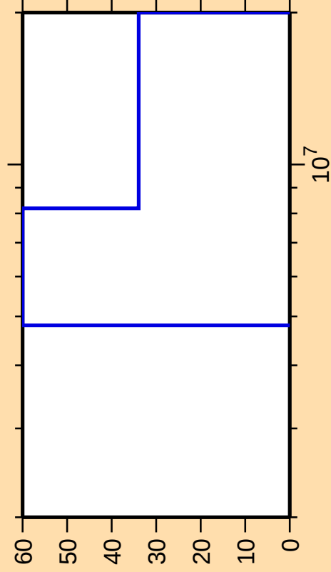
\Delta\sigma/\sigma vs. E for ^{227}\text{Th}(n,2n)
