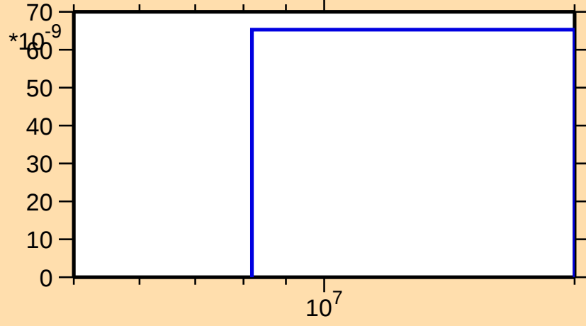
\sigma vs. E for ^{227}\text{Th}(n,\text{nd})
