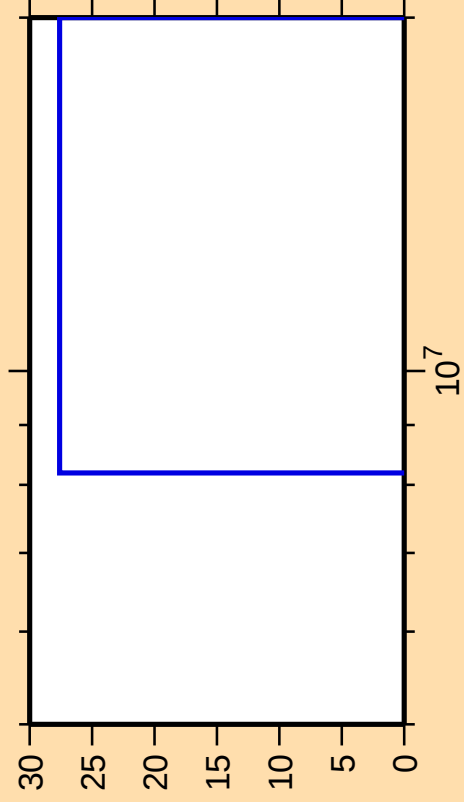
\Delta\sigma/\sigma vs. E for ^{227}\text{Th}(n,\text{He}3)
