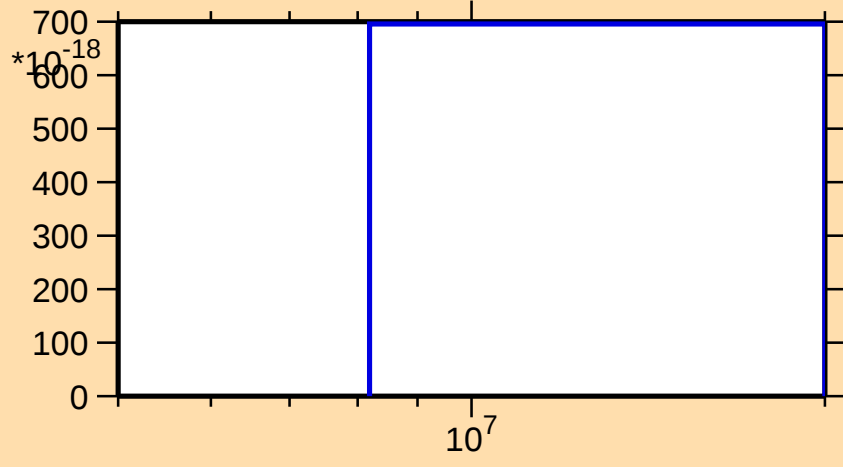
\sigma vs. E for ^{227}\text{Th}(\text{mt } 11)
