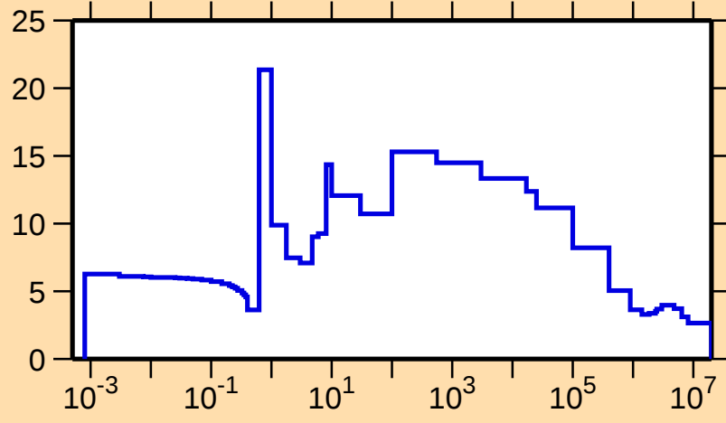
\sigma vs. E for ^{227}\text{Th}(n,\text{el.})
