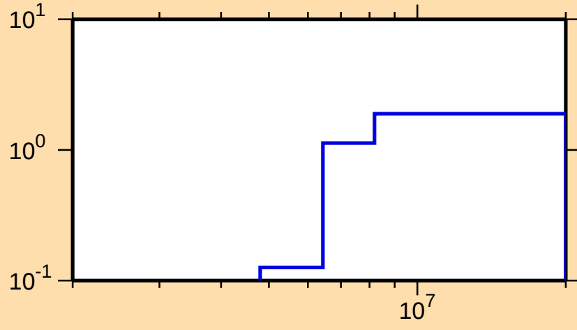
\sigma vs. E for ^{227}\text{Th}(n,2n)
