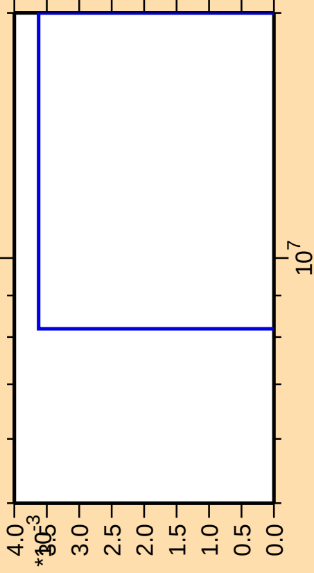
\Delta\sigma/\sigma vs. E for ^{227}\text{Th}(\text{mt } 11)
