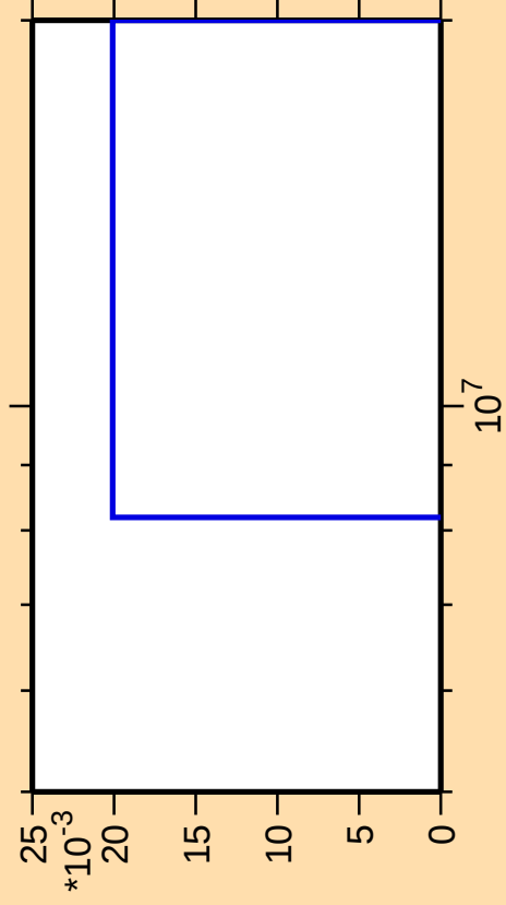
\Delta\sigma/\sigma vs. E for ^{227}\text{Th}(\text{mt } 34)
