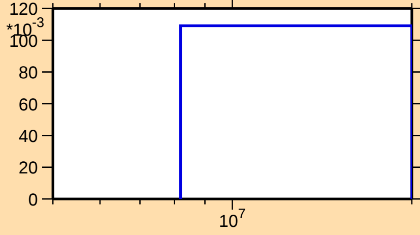
\sigma vs. E for ^{227}\text{Th}(n,3n)
