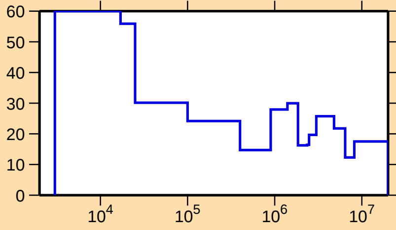
\Delta\sigma/\sigma vs. E for ^{227}\text{Th}(n,\text{el.})
