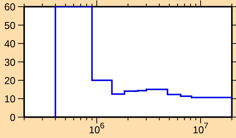
\Delta\sigma/\sigma vs. E for ^{227}\text{Th}(n,\text{nonel.})
