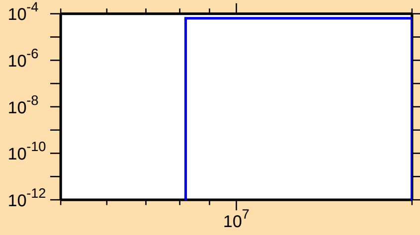
\sigma vs. E for ^{227}\text{Th}(n,t)
