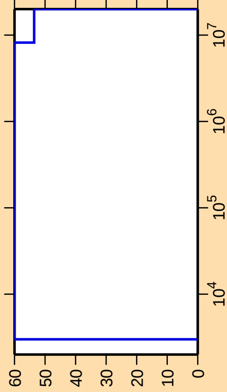
\Delta\sigma/\sigma vs. E for ^{227}\text{Th}(n,\alpha)
