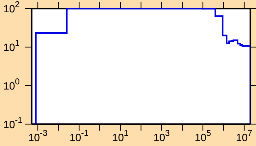
\Delta\sigma/\sigma vs. E for ^{227}\text{Th}(n,\text{nonel.})
