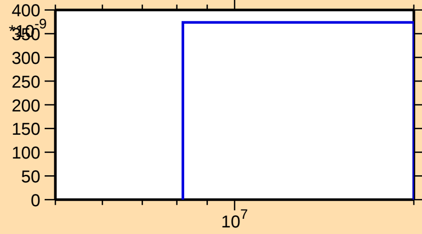
\sigma vs. E for ^{227}\text{Th}(n,3n\alpha)
