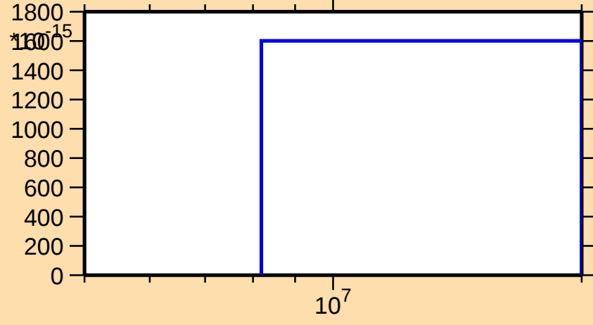
\sigma vs. E for ^{227}\text{Th}(n,p\alpha)
