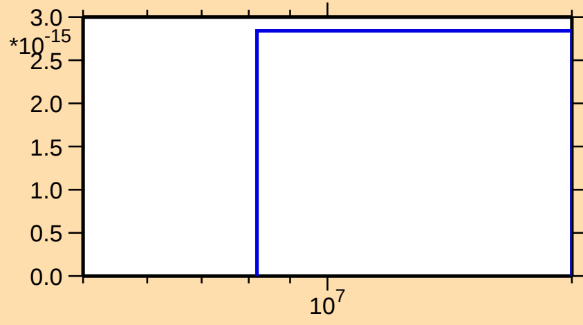
\sigma vs. E for ^{227}\text{Th}(\text{mt } 34)
