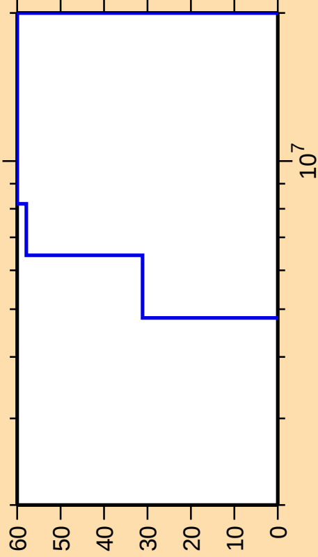
\Delta\sigma/\sigma vs. E for ^{227}\text{Th}(n,n\text{cont.})
