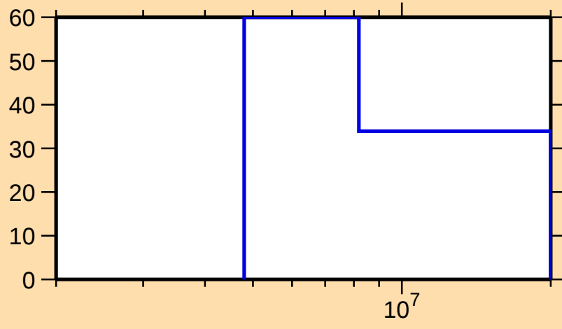
\Delta\sigma/\sigma vs. E for ^{227}\text{Th}(n,2n)
