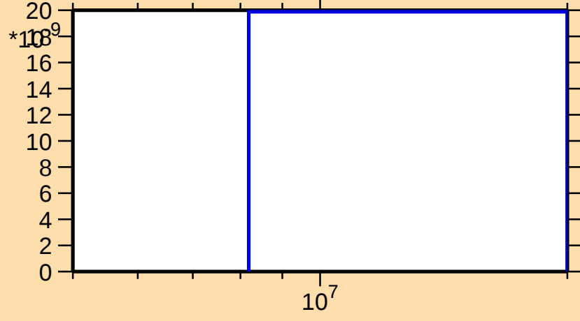
\sigma vs. E for ^{227}\text{Th}(n,\text{nt})
