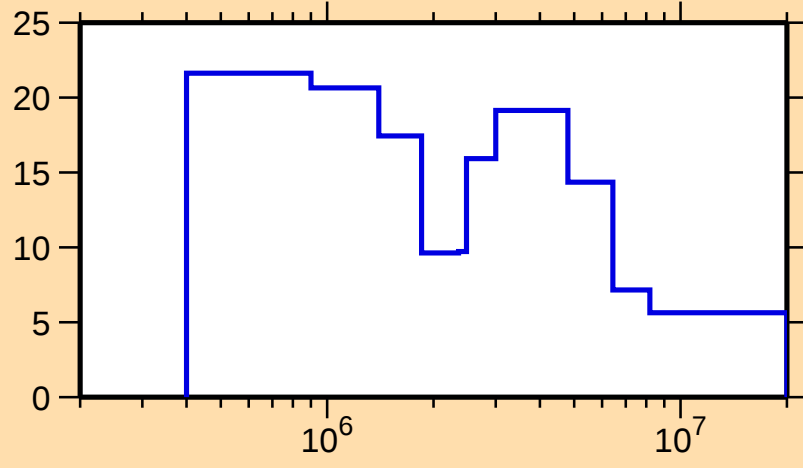
\Delta\sigma/\sigma vs. E for ^{227}\text{Th}(n,\text{tot.})
