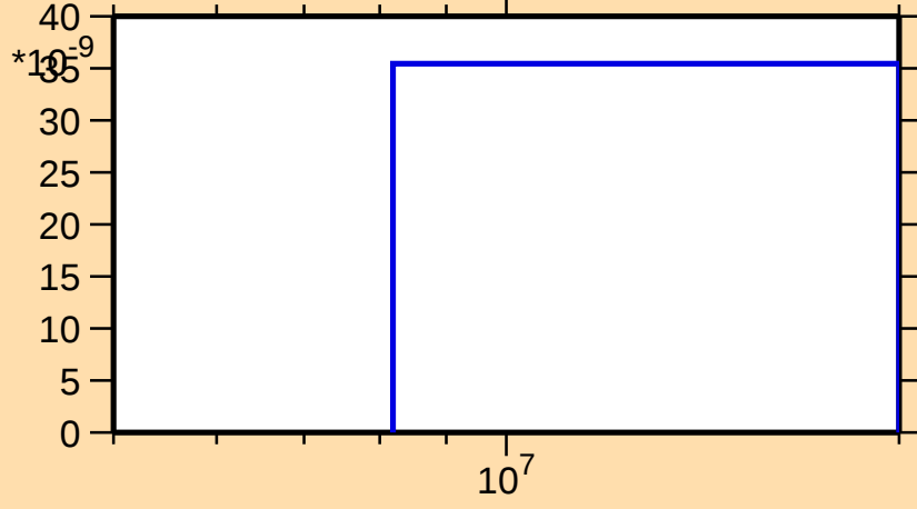
\sigma vs. E for ^{227}\text{Th}(n,2np)
