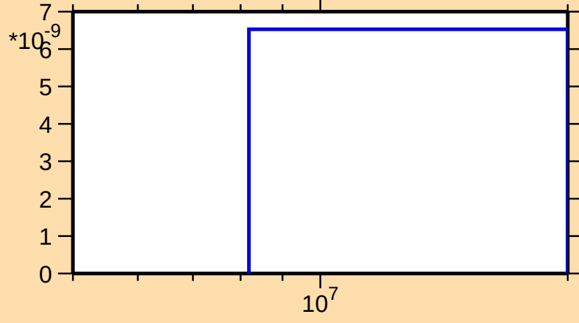
\sigma vs. E for ^{228}\text{Th}(n,nt)
