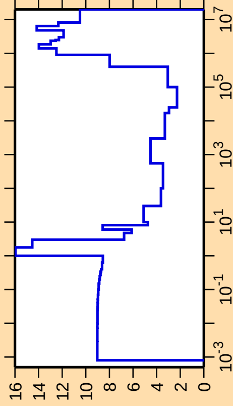
\Delta\sigma/\sigma vs. E for ^{228}\text{Th}(\text{n},\text{el.})
