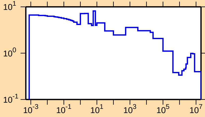
\Delta\sigma/\sigma vs. E for ^{228}\text{Th}(\text{n},\text{tot.})
