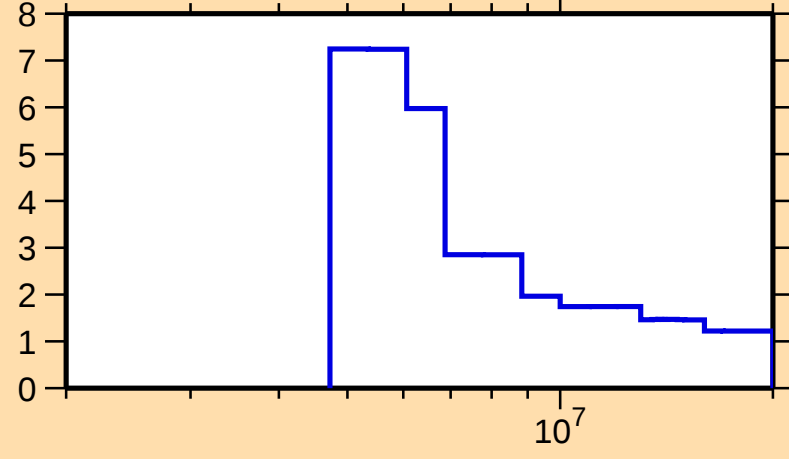
\Delta\sigma/\sigma vs. E for ^{229}\text{Th}(n,\text{nonel.})
