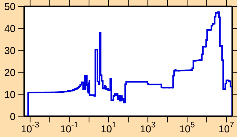
\Delta\sigma/\sigma vs. E for ^{229}\text{Th}(n,\gamma)
