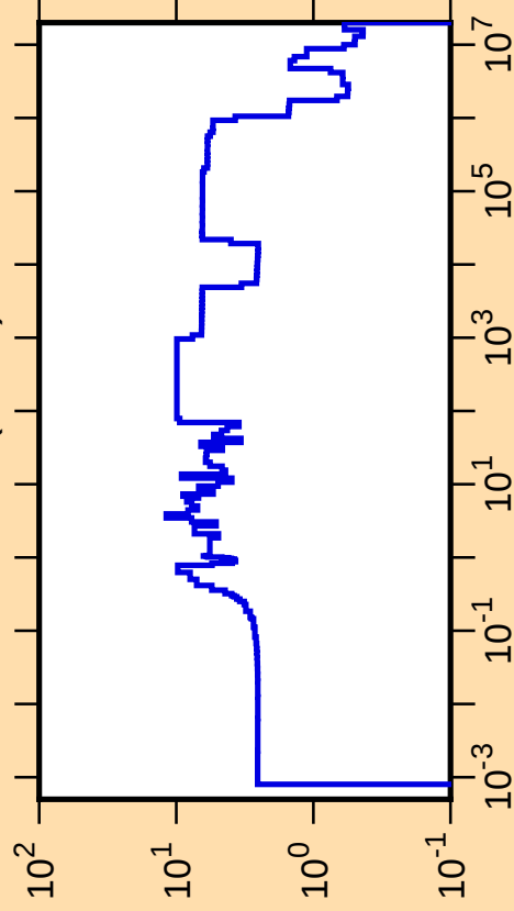
\Delta\sigma/\sigma vs. E for ^{229}\text{Th}(n,\text{tot.})
