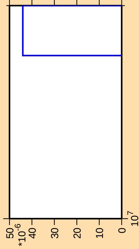
\Delta\sigma/\sigma vs. E for ^{229}\text{Th} (mt 42)
