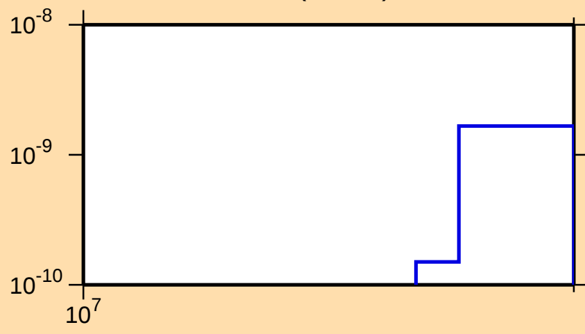
\sigma vs. E for ^{229}\text{Th}(n,3n\alpha)
