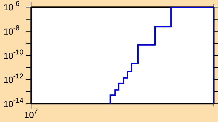
\sigma vs. E for ^{229}\text{Th}(n,nt)
