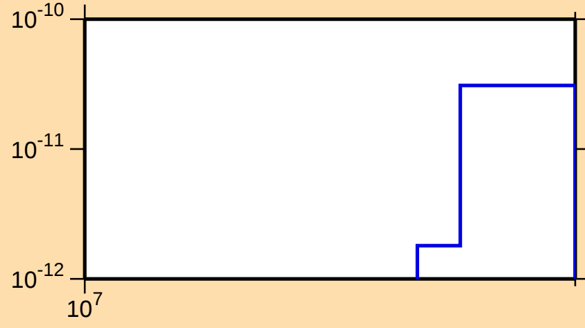
\sigma vs. E for ^{229}\text{Th}(n,\text{He}3)
