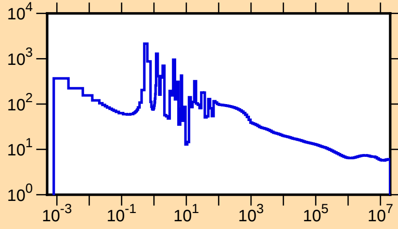
\sigma vs. E for ^{229}\text{Th}(n,\text{tot.})
