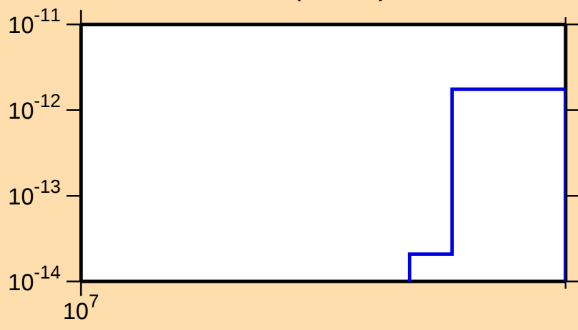
\sigma vs. E for ^{231}\text{Th}(n,\text{He3})
