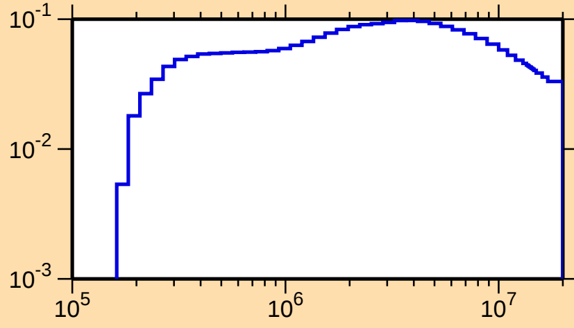
\sigma vs. E for ^{231}\text{Th}(n,n_3)
