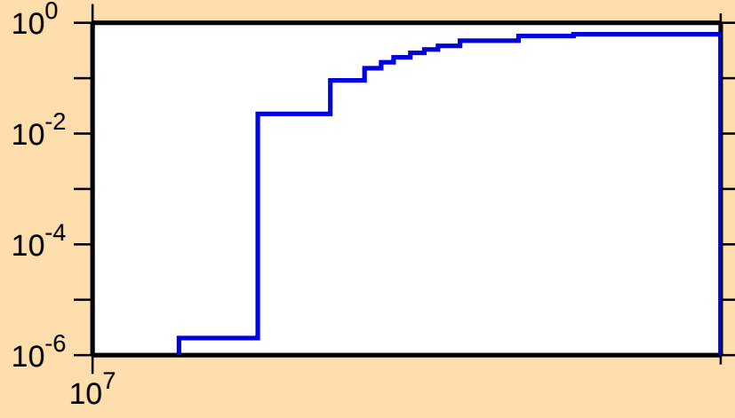
\sigma vs. E for ^{231}\text{Th}(n,3n)
