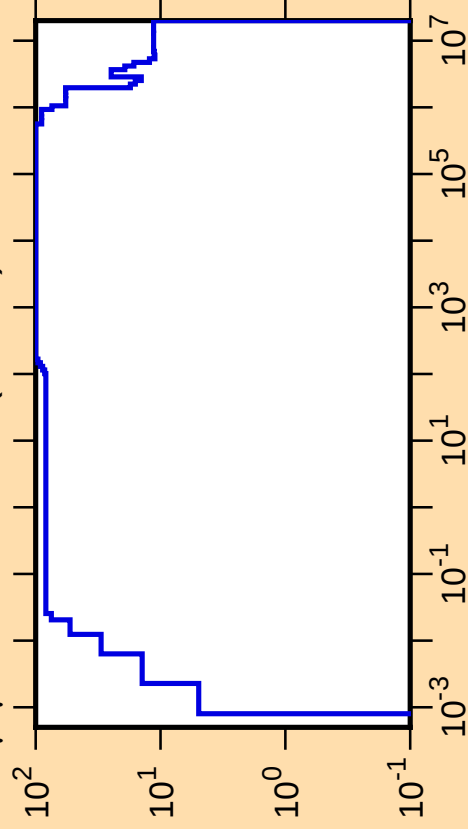
\Delta\mu/\mu vs. E for ^{235}\text{Th}(\text{mt251})
