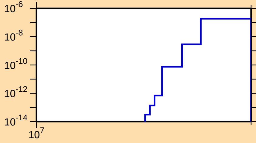
\sigma vs. E for ^{235}\text{Th}(n,\text{nd})
