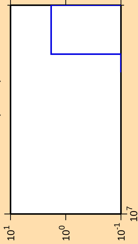
\Delta\sigma/\sigma vs. E for ^{235}\text{Th}(n,3n\alpha)
