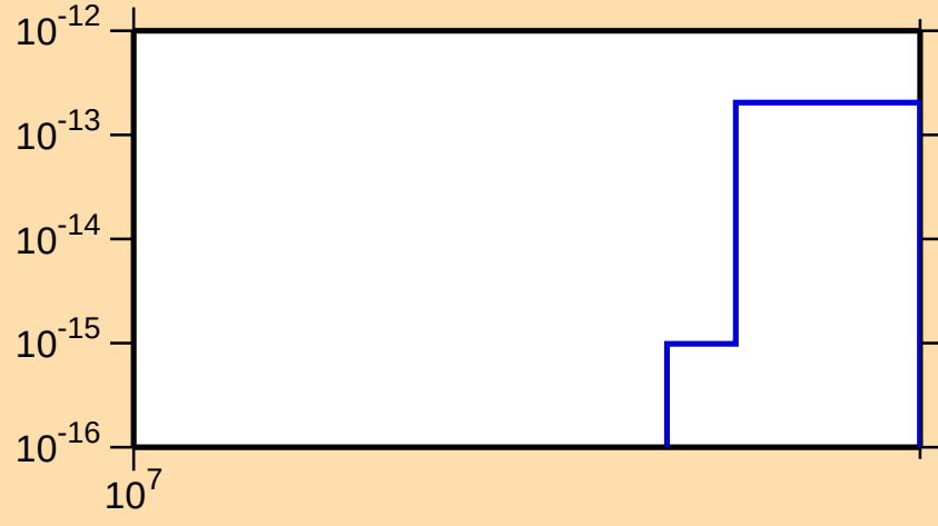
\sigma vs. E for ^{235}\text{Th}(n,3n\alpha)
