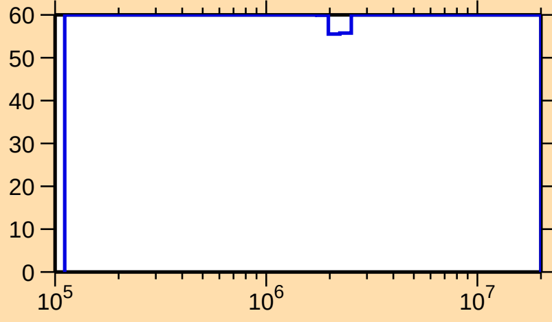
\Delta\sigma/\sigma vs. E for ^{235}\text{Th}(n,n_1)
