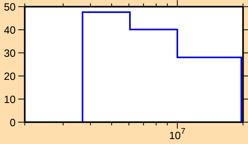
\Delta\sigma/\sigma vs. E for ^{235}\text{Th}(n,2n)
