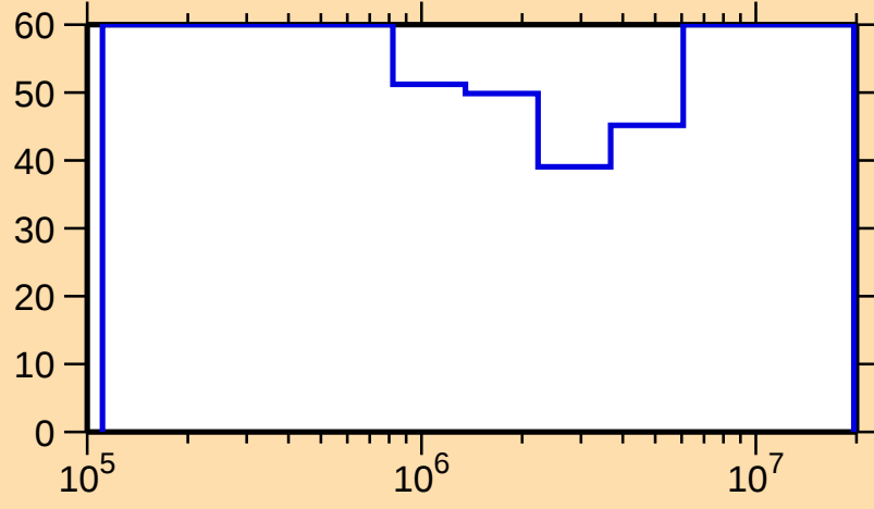
\Delta\sigma/\sigma vs. E for ^{235}\text{Th}(n,\text{inel.})
