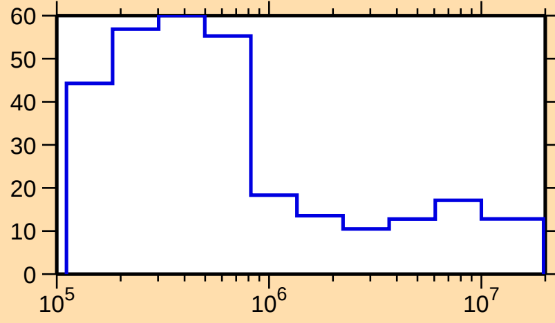
\Delta\sigma/\sigma vs. E for ^{235}\text{Th}(n,\text{tot.})
