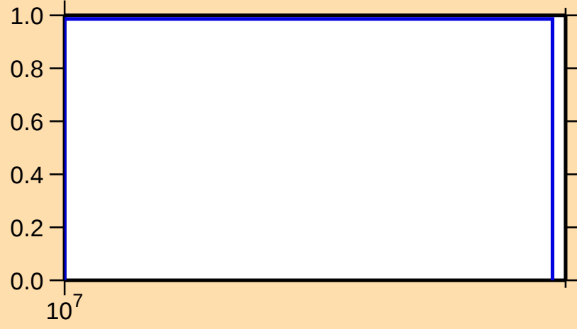
\sigma vs. E for ^{235}\text{Th}(n,3n)
