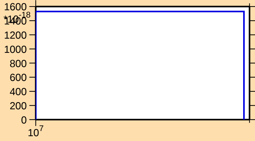
\sigma vs. E for ^{235}\text{Th}(n,3n\alpha)
