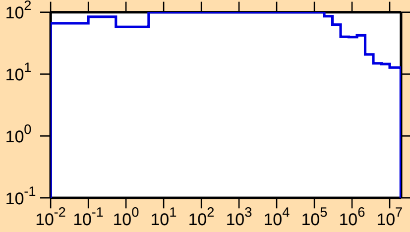
\Delta\sigma/\sigma vs. E for ^{235}\text{Th}(n,\text{nonel.})
