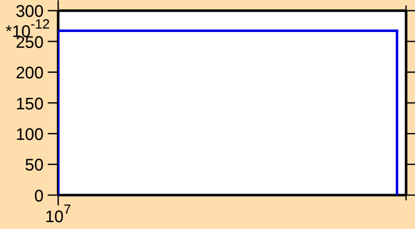
\sigma vs. E for ^{235}\text{Th}(n,2np)
