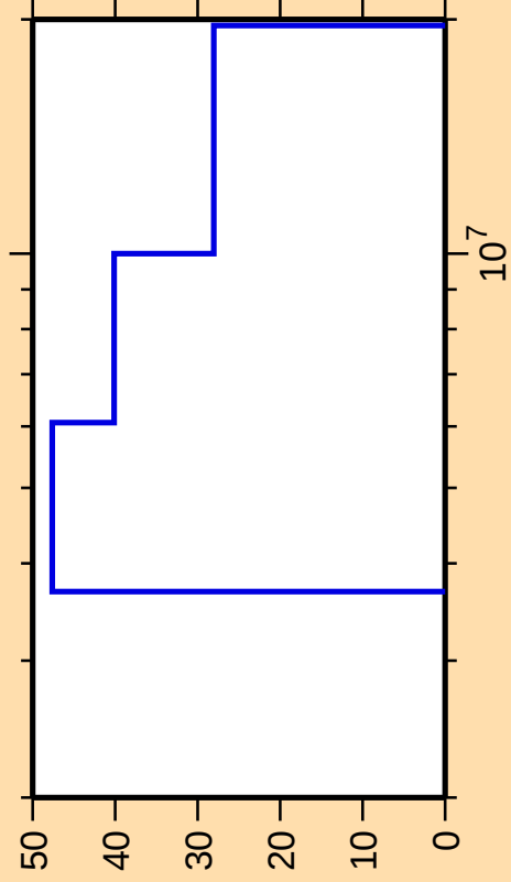
\Delta\sigma/\sigma vs. E for ^{235}\text{Th}(n,2n)
