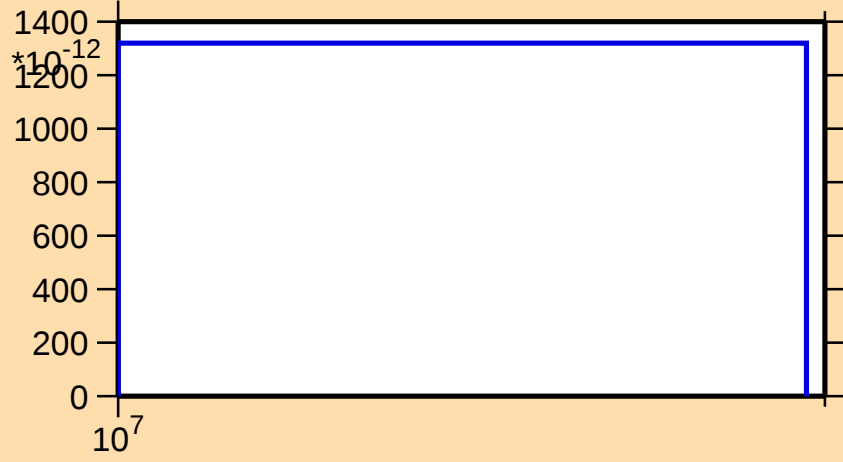
\sigma vs. E for ^{235}\text{Th}(n,\text{nt})
