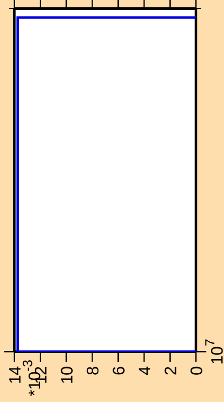
\Delta\sigma/\sigma vs. E for ^{235}\text{Th}(n,3n\alpha)
