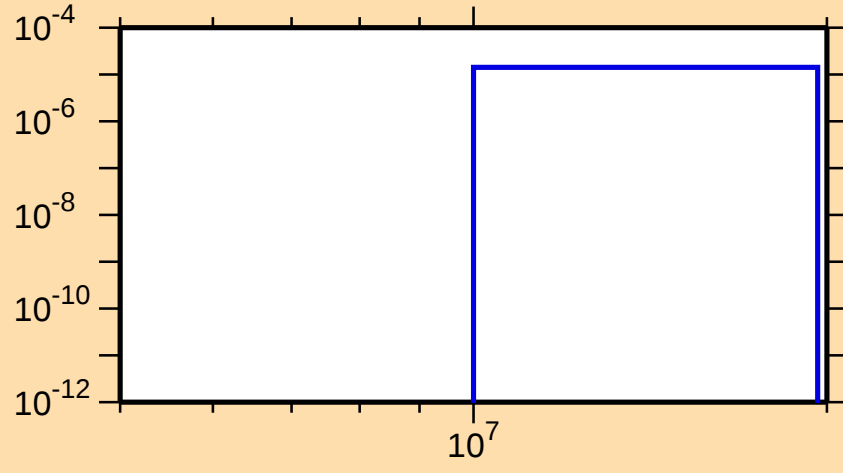
\sigma vs. E for ^{235}\text{Th}(n,d)
