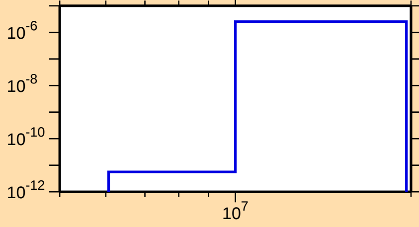
\sigma vs. E for ^{235}\text{Th}(n,\alpha)
