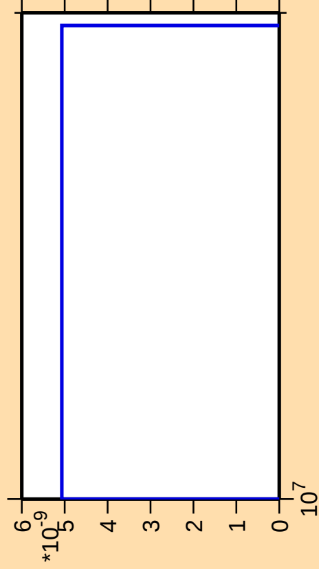
\Delta\sigma/\sigma vs. E for ^{235}\text{Th}(\text{mt } 42)
