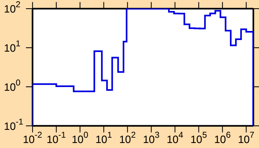
\Delta\sigma/\sigma vs. E for ^{235}\text{Th}(n,\text{el.})
