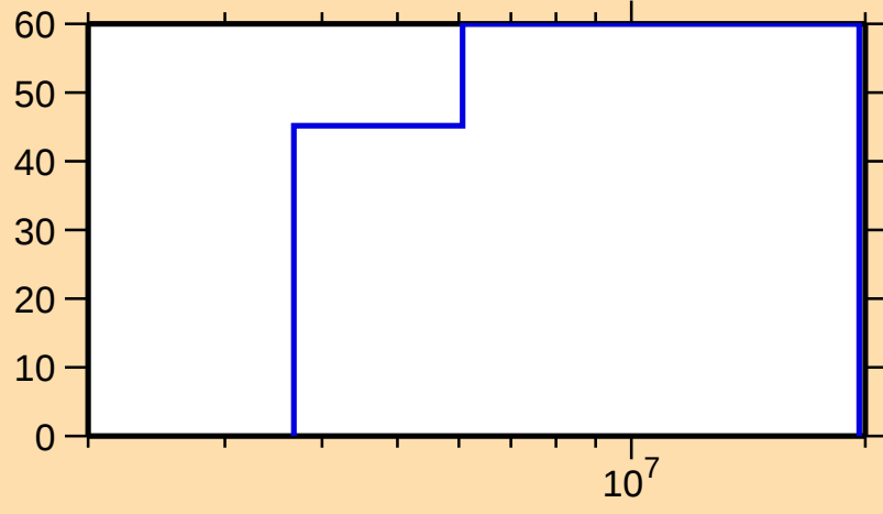
\Delta\sigma/\sigma vs. E for ^{235}\text{Th}(n,\text{inel.})
