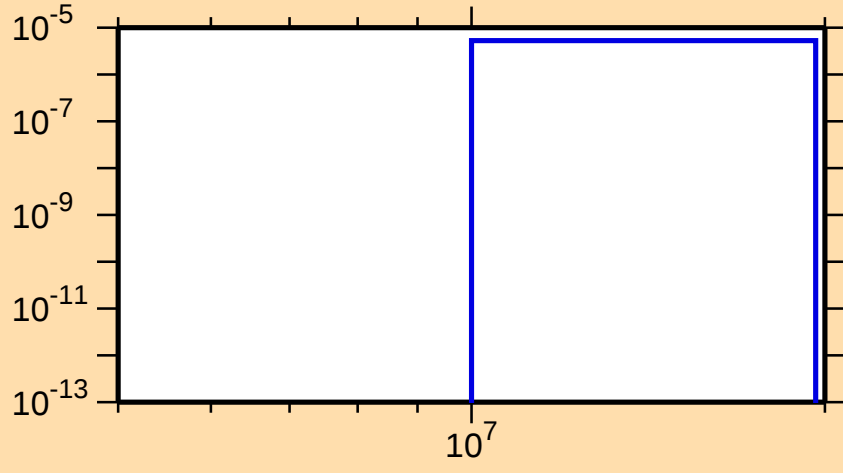
\sigma vs. E for ^{235}\text{Th}(n,np)
