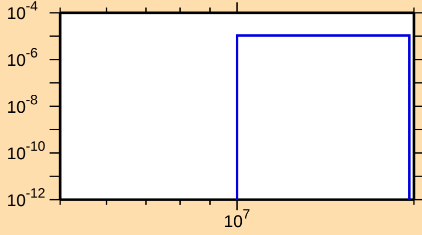
\sigma vs. E for ^{235}\text{Th}(n,t)
