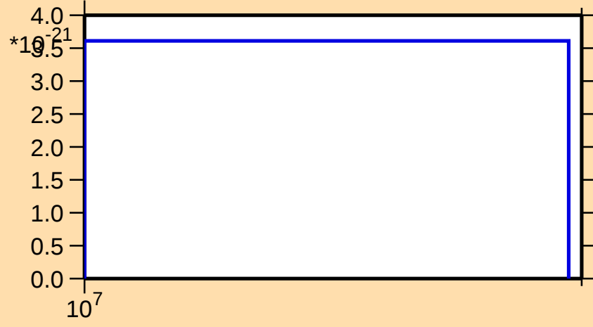
\sigma vs. E for ^{235}\text{Th}(\text{mt } 42)
