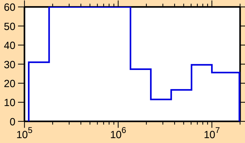
\Delta\sigma/\sigma vs. E for ^{235}\text{Th}(n,\text{el.})
