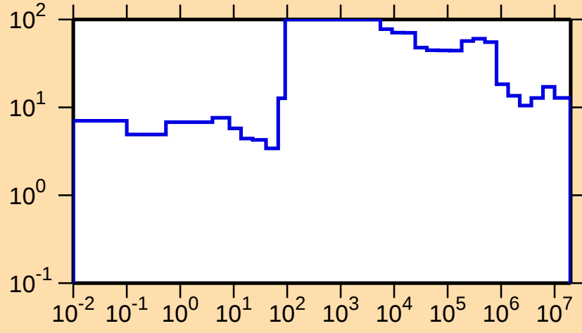
\Delta\sigma/\sigma vs. E for ^{235}\text{Th}(n,\text{tot.})
