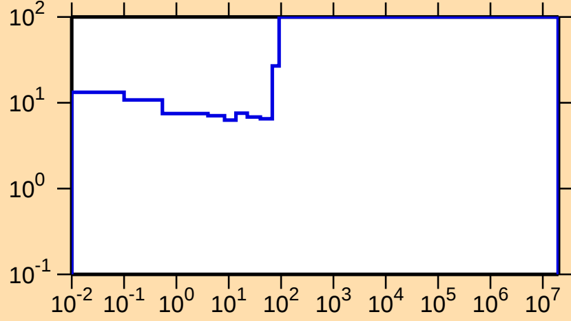
\Delta\sigma/\sigma vs. E for ^{235}\text{Th}(n,f)
