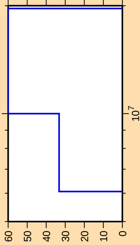
\Delta\sigma/\sigma vs. E for ^{235}\text{Th}(n,\alpha)
