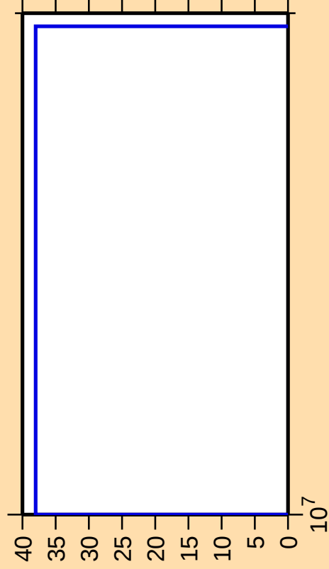
\Delta\sigma/\sigma vs. E for ^{235}\text{Th}(n,3n)
