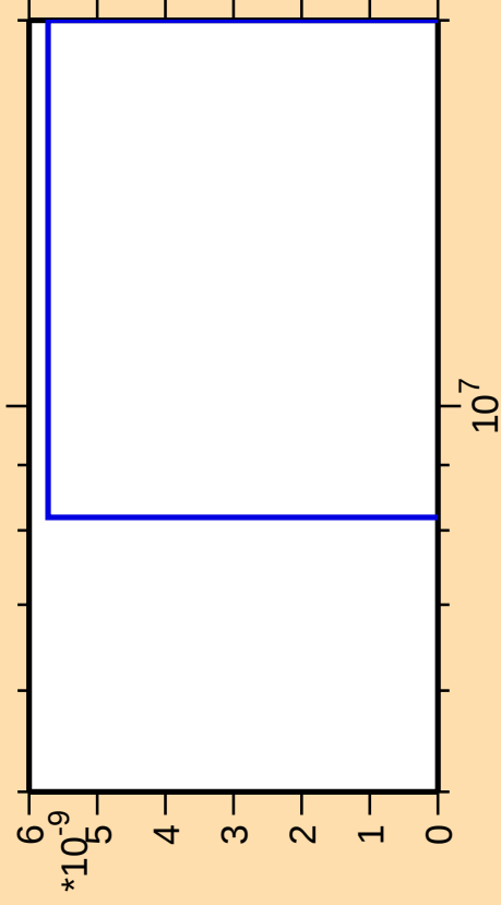
\Delta\sigma/\sigma vs. E for ^{235}\text{Th}(\text{mt } 42)
