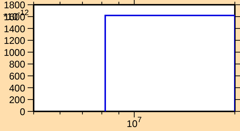
\sigma vs. E for ^{235}\text{Th}(n,\text{nd})
