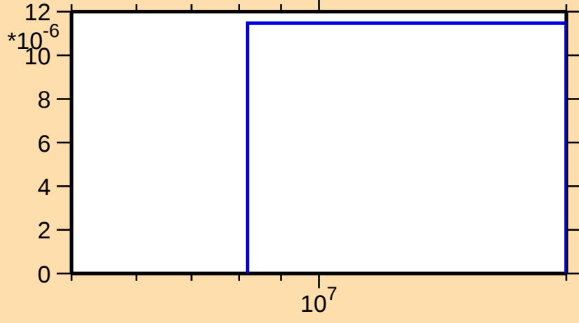
\sigma vs. E for ^{235}\text{Th}(n,d)
