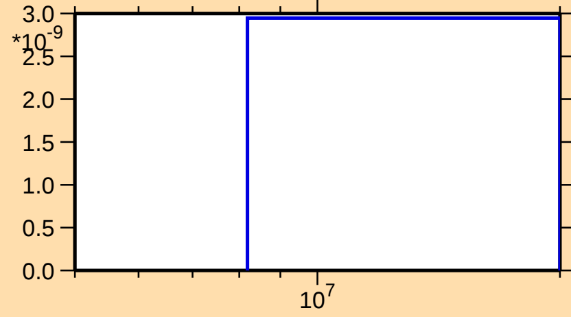
\sigma vs. E for ^{235}\text{Th}(n,2n\alpha)
