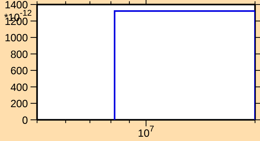
\sigma vs. E for ^{235}\text{Th}(n,nt)
