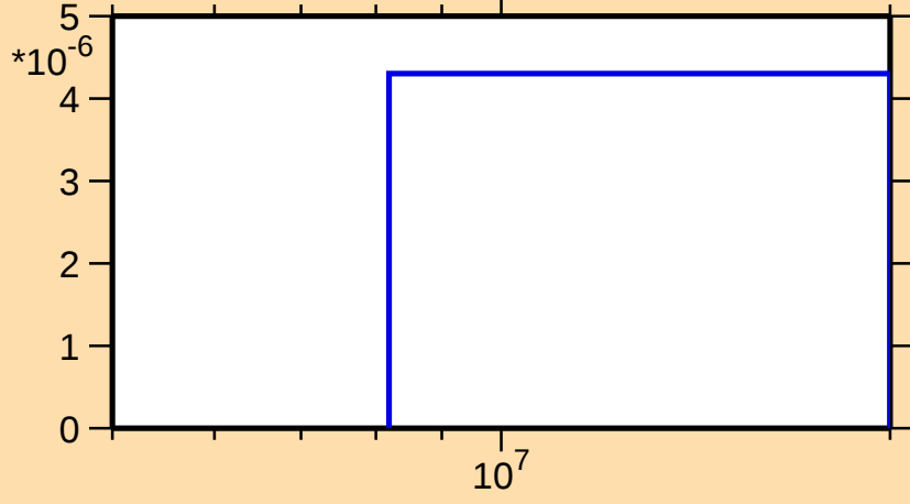
\sigma vs. E for ^{235}\text{Th}(n,np)
