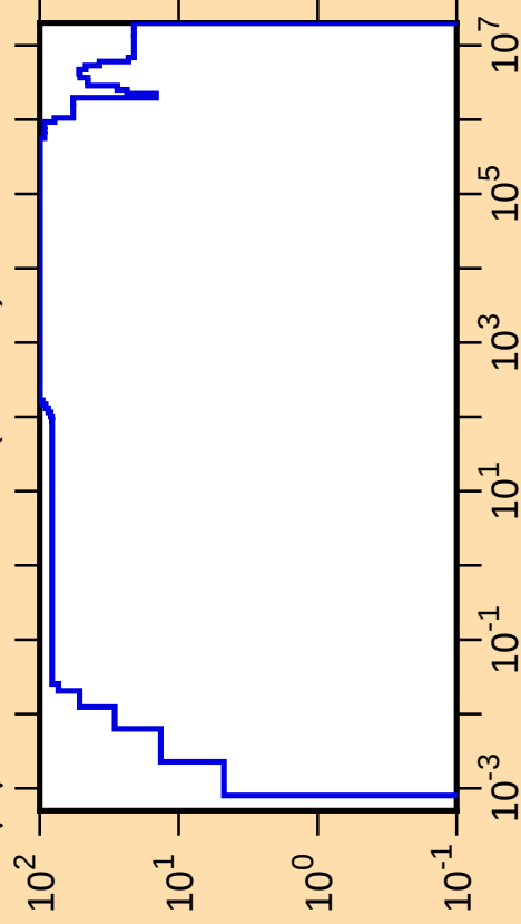
\Delta\mu/\mu vs. E for ^{239}\text{Th}(\text{mt251})
