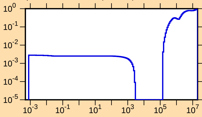
\mu vs. E for ^{239}\text{Th}(\text{mt251})
