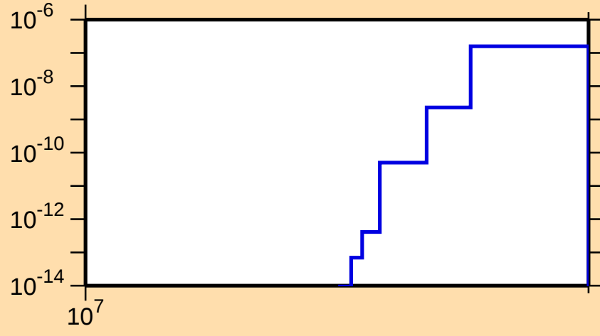
\sigma vs. E for ^{239}\text{Th}(n,\text{nd})
