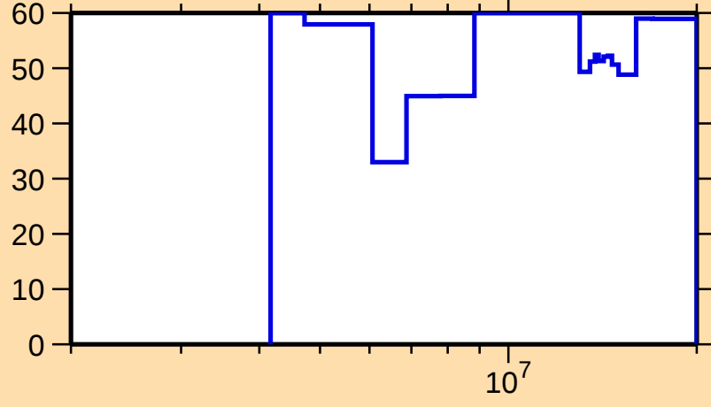
\Delta\sigma/\sigma vs. E for ^{239}\text{Th}(n,n\text{cont.})
