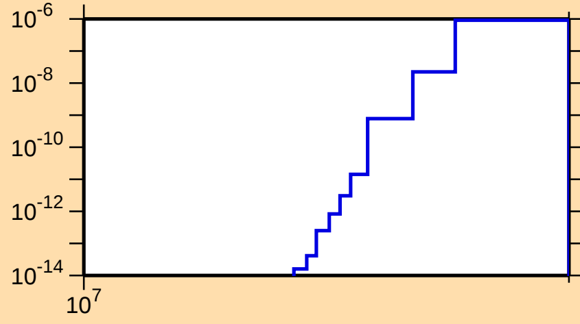
\sigma vs. E for ^{239}\text{Th}(n,\text{nt})
