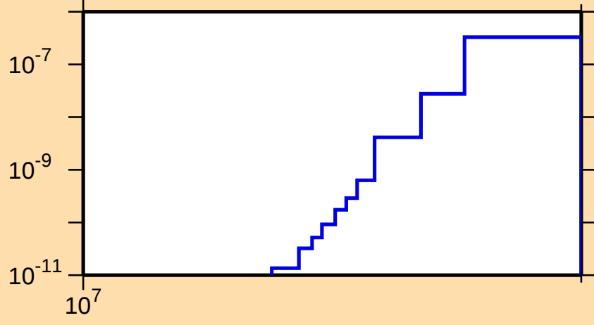
\sigma vs. E for ^{239}\text{Th}(n,2n\alpha)
