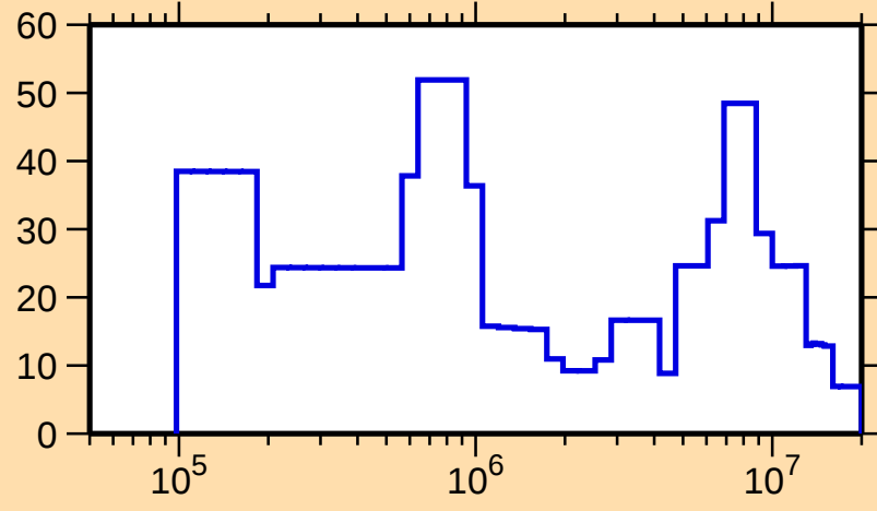
\Delta\sigma/\sigma vs. E for ^{239}\text{Th}(n,\text{tot.})
