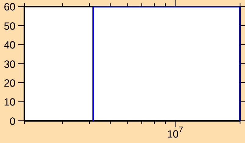
\Delta\sigma/\sigma vs. E for ^{239}\text{Th}(n,f)
