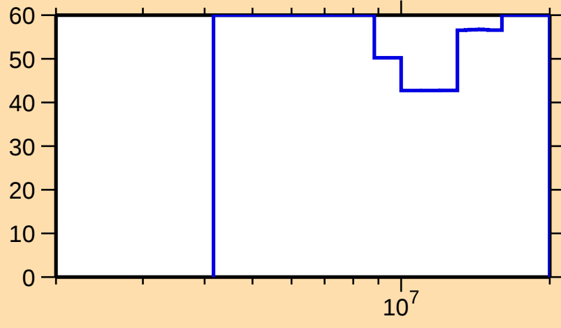
\Delta\sigma/\sigma vs. E for ^{239}\text{Th}(n,2n)
