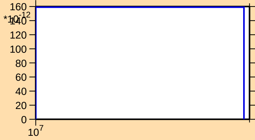
\sigma vs. E for ^{239}\text{Th}(n,2np)
