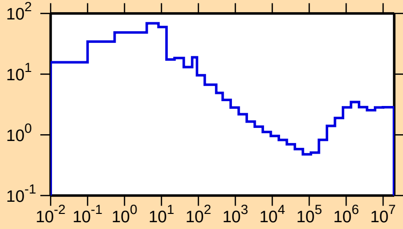
\sigma vs. E for ^{239}\text{Th}(n,\text{nonel.})
