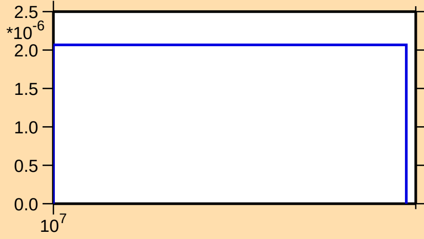
\sigma vs. E for ^{239}\text{Th}(n,np)
