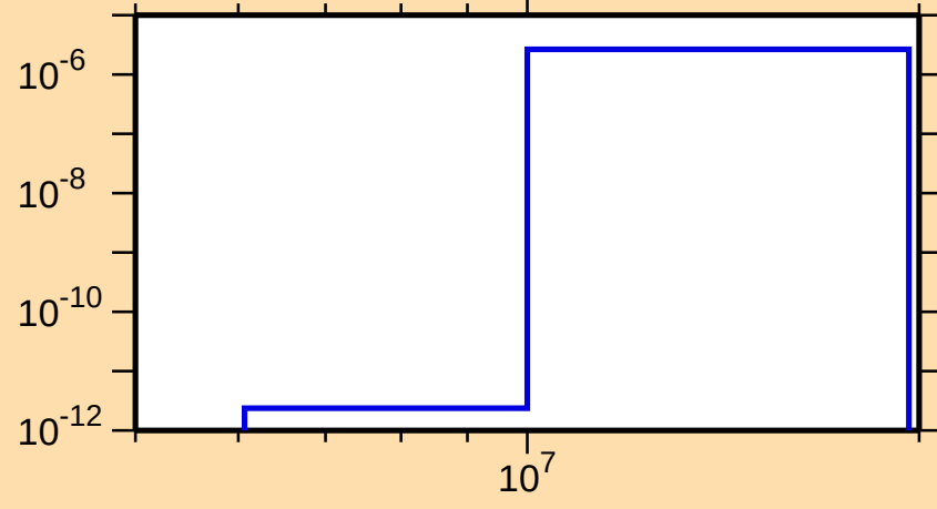
\sigma vs. E for ^{239}\text{Th}(n,n\alpha)
