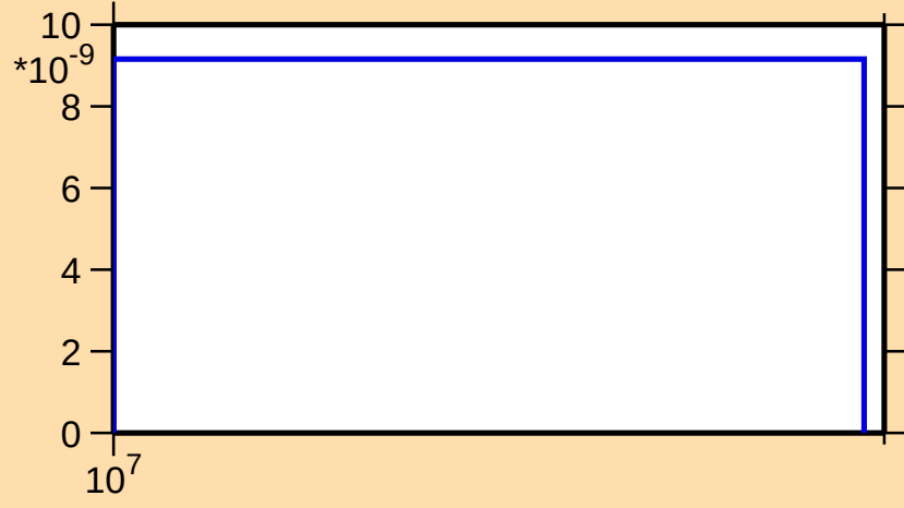
\sigma vs. E for ^{239}\text{Th}(n,\text{nt})
