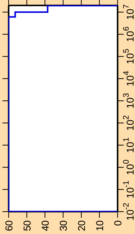
\Delta\sigma/\sigma vs. E for ^{239}\text{Th}(n,\text{nonel.})
