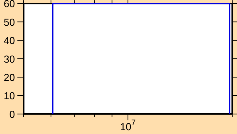
\Delta\sigma/\sigma vs. E for ^{239}\text{Th}(n,p)
