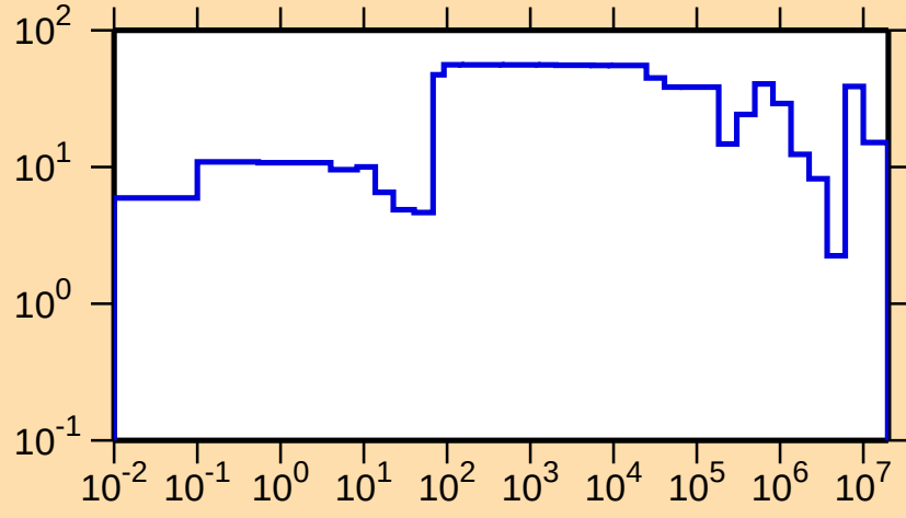
\Delta\sigma/\sigma vs. E for ^{239}\text{Th}(n,\text{tot.})
