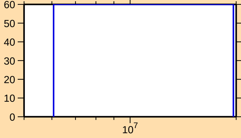
\Delta\sigma/\sigma vs. E for ^{239}\text{Th}(n,\text{inel.})
