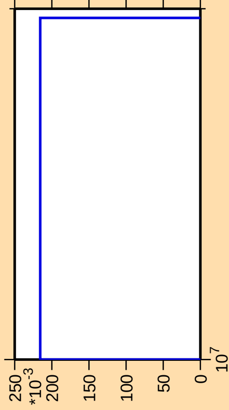
\Delta\sigma/\sigma vs. E for ^{239}\text{Th}(n,3n\alpha)
