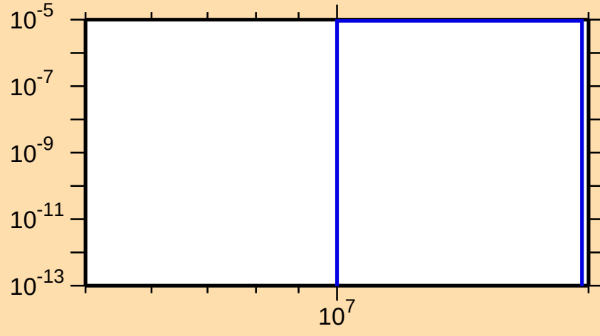
\sigma vs. E for ^{239}\text{Th}(n,t)
