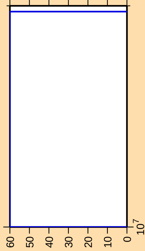
\Delta\sigma/\sigma vs. E for ^{239}\text{Th}(n,\text{nt})
