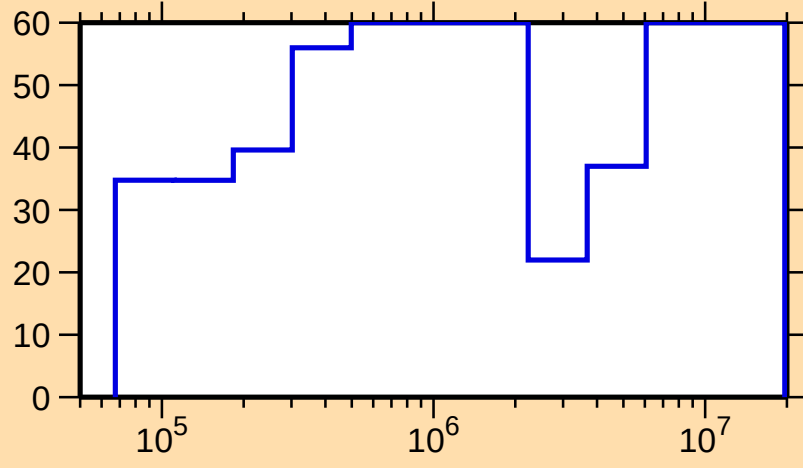
\Delta\sigma/\sigma vs. E for ^{239}\text{Th}(n,\text{el.})
