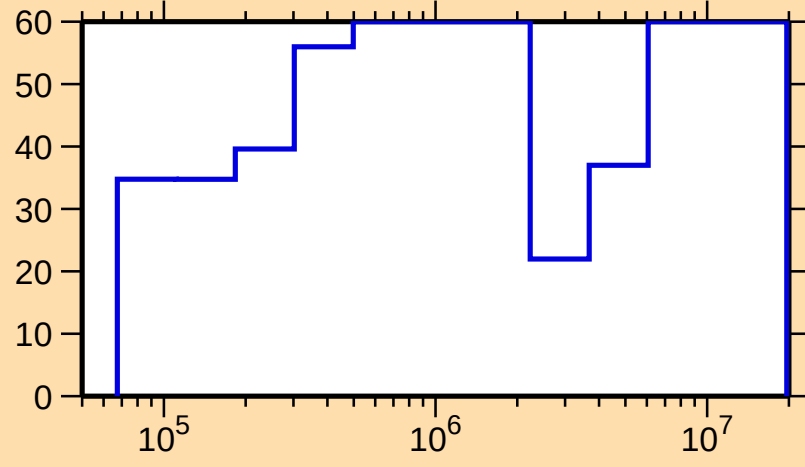
\Delta\sigma/\sigma vs. E for ^{239}\text{Th}(n,\text{el.})
