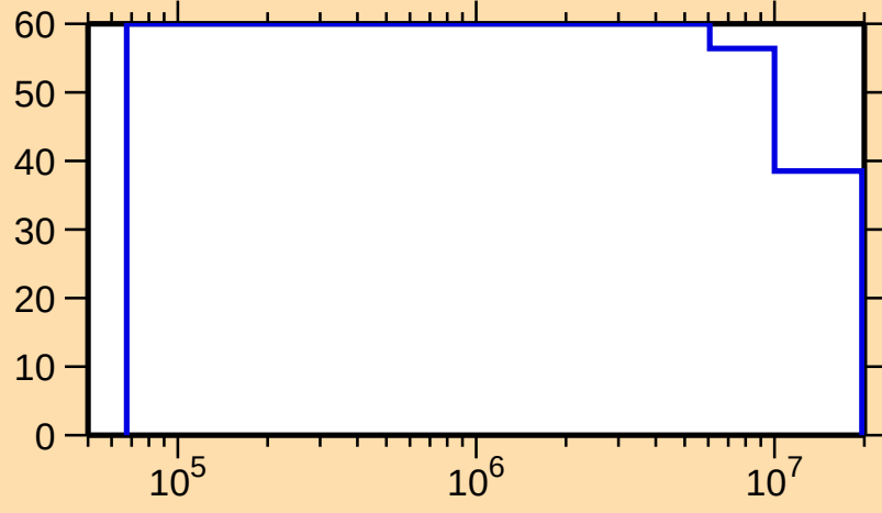
\Delta\sigma/\sigma vs. E for ^{239}\text{Th}(n,\text{nonel.})
