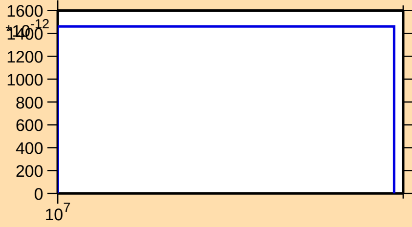
\sigma vs. E for ^{239}\text{Th}(n,\text{nd})
