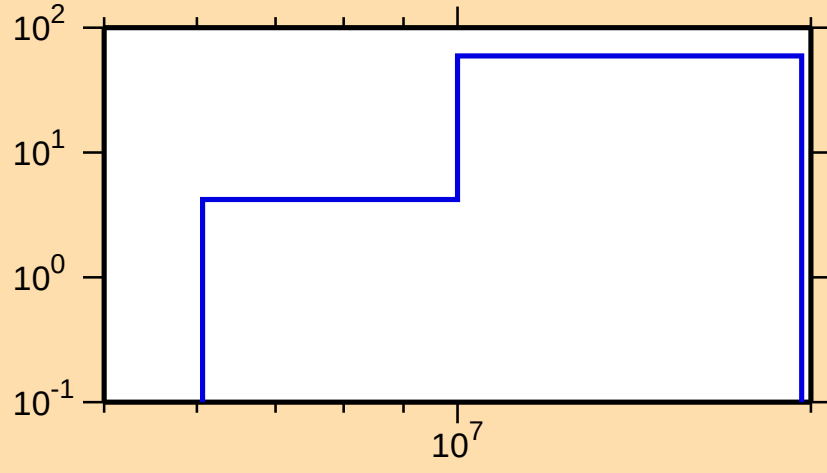
\Delta\sigma/\sigma vs. E for ^{239}\text{Th}(n,\text{ncont.})
