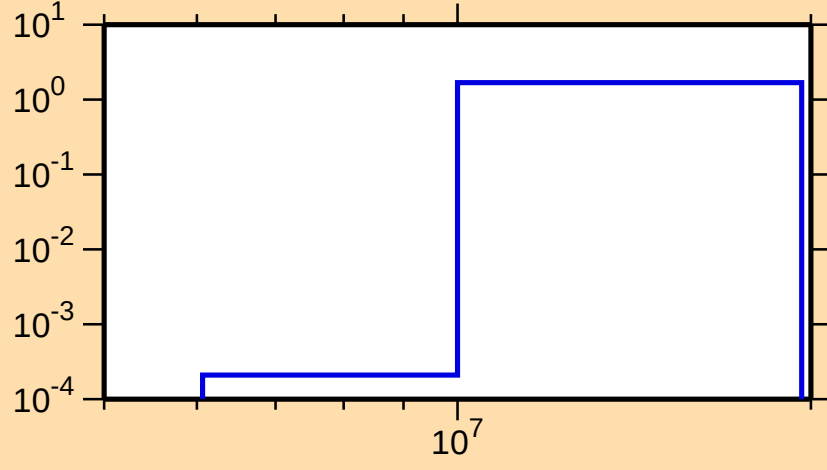
\sigma vs. E for ^{239}\text{Th}(n,3n)
