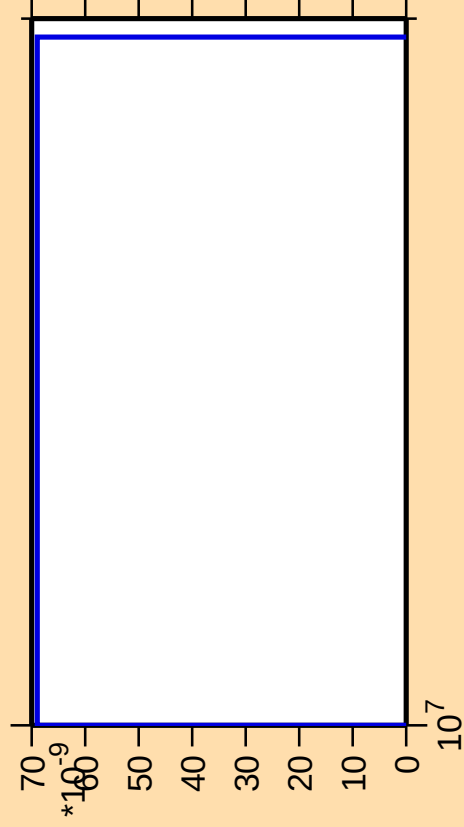
\Delta\sigma/\sigma vs. E for ^{239}\text{Th}(\text{mt } 42)
