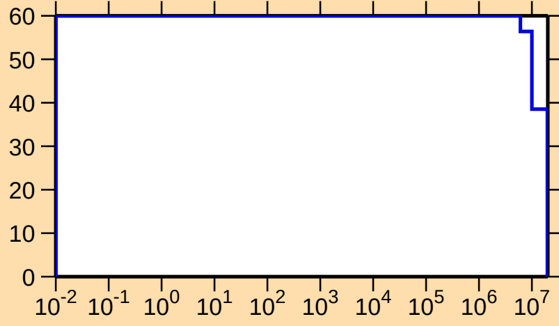
\Delta\sigma/\sigma vs. E for ^{239}\text{Th}(n,\text{nonel.})
