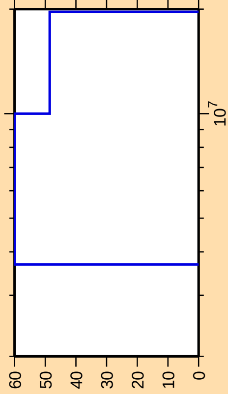
\Delta\sigma/\sigma vs. E for ^{239}\text{Th}(n,2n)
