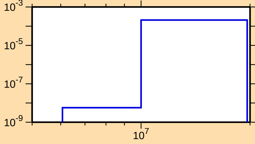
\sigma vs. E for ^{239}\text{Th}(n,p)
