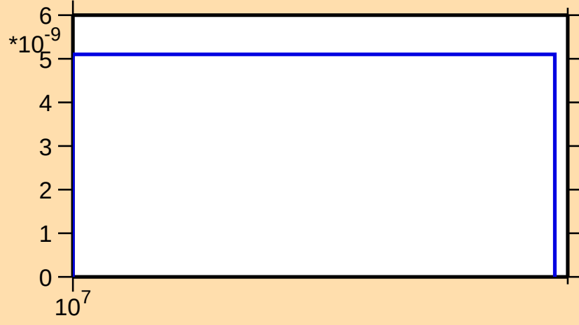
\sigma vs. E for ^{239}\text{Th}(n,2n\alpha)
