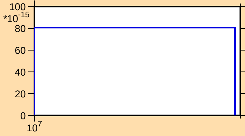
\sigma vs. E for ^{239}\text{Th}(n,3n\alpha)
