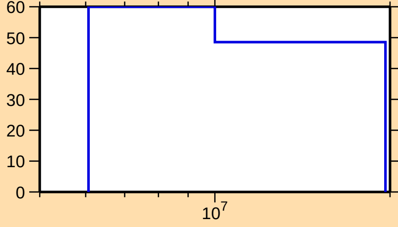
\Delta\sigma/\sigma vs. E for ^{239}\text{Th}(n,2n)
