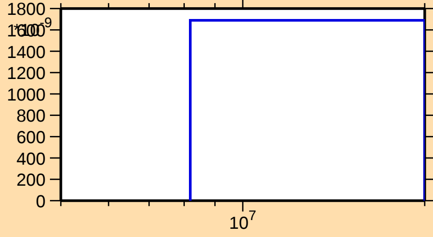
\sigma vs. E for ^{239}\text{Th}(n,np)
