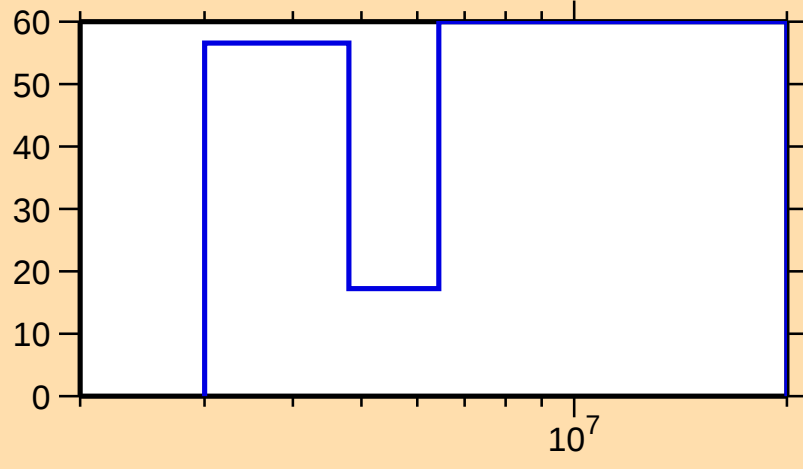
\Delta\sigma/\sigma vs. E for ^{239}\text{Th}(n,\text{inel.})
