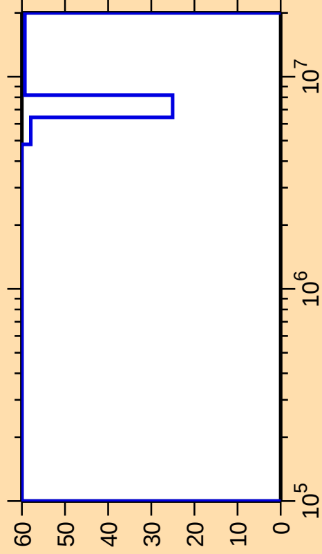
\Delta\sigma/\sigma vs. E for ^{239}\text{Th}(\text{n},\text{ncont.})
