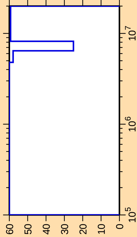
\Delta\sigma/\sigma vs. E for ^{239}\text{Th}(n,n_{\text{cont}})
