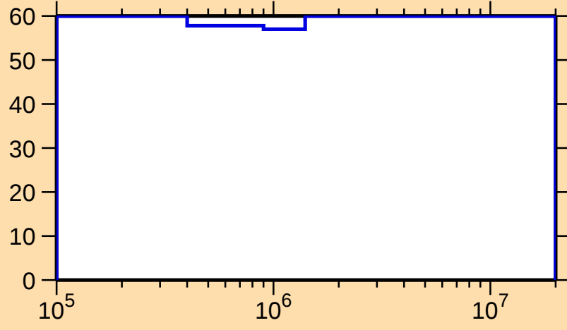
\Delta\sigma/\sigma vs. E for ^{239}\text{Th}(n,n_1)
