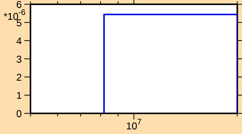
\sigma vs. E for ^{239}\text{Th}(n,d)
