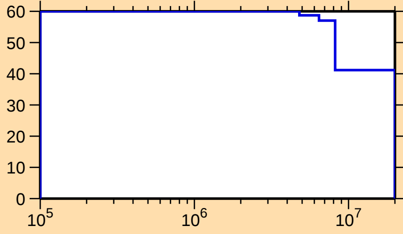
\Delta\sigma/\sigma vs. E for ^{239}\text{Th}(\text{n},\text{nonel.})
