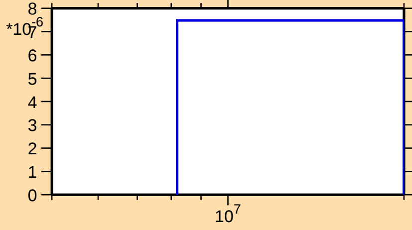
\sigma vs. E for ^{239}\text{Th}(n,t)
