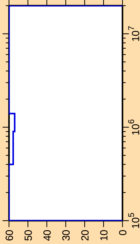
\Delta\sigma/\sigma vs. E for ^{239}\text{Th}(n,n_1)
