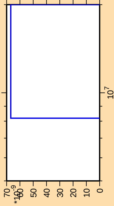
\Delta\sigma/\sigma vs. E for ^{239}\text{Th}(\text{mt } 42)
