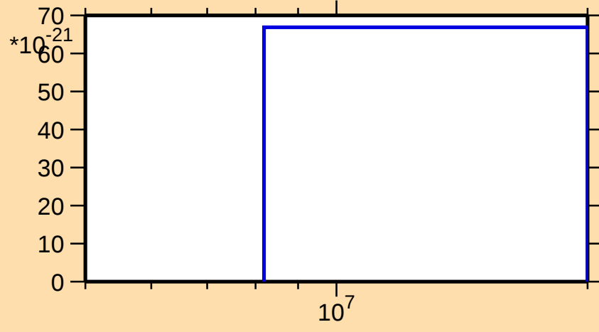
\sigma vs. E for ^{239}\text{Th}(\text{mt } 42)
