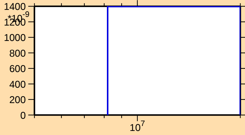
\sigma vs. E for ^{46}\text{Ti}(n,t)
