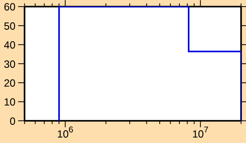
\Delta\sigma/\sigma vs. E for ^{46}\text{Ti}(n,\gamma)
