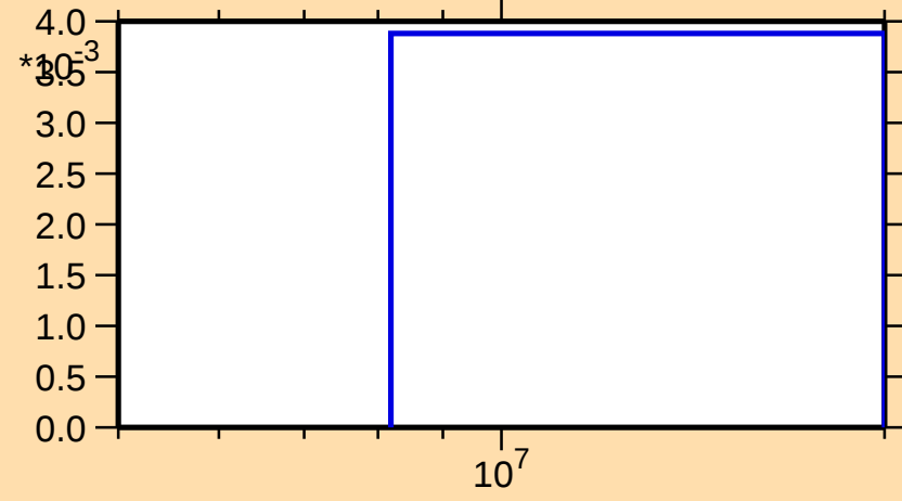
\sigma vs. E for ^{46}\text{Ti}(n,d)
