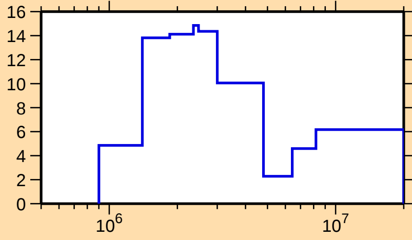
\Delta\sigma/\sigma vs. E for ^{46}\text{Ti}(n,\text{el.})
