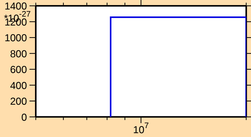
\sigma vs. E for ^{46}\text{Ti}(n,2n\alpha)
