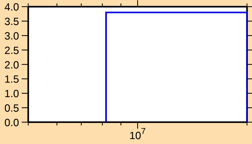
\Delta\sigma/\sigma vs. E for ^{46}\text{Ti}(n,\text{nonel.})
