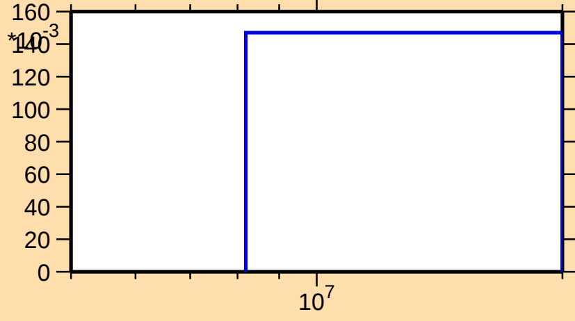
\sigma vs. E for ^{46}\text{Ti}(n,np)
