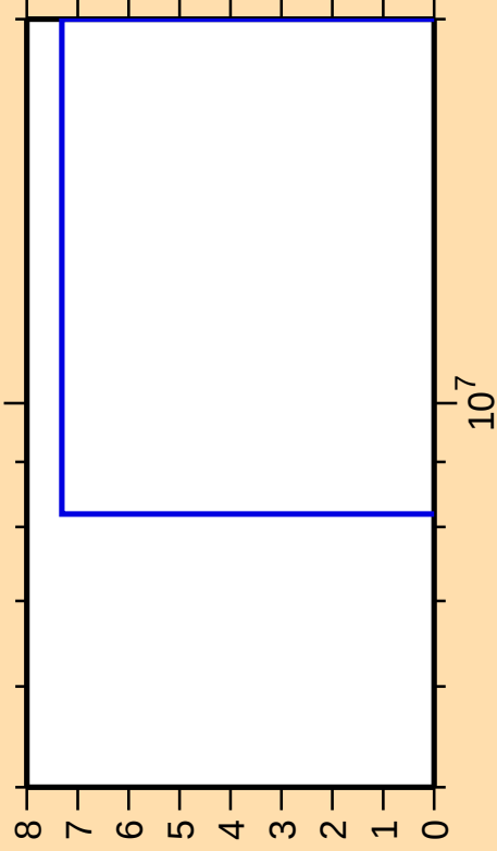
\Delta\sigma/\sigma vs. E for ^{46}\text{Ti}(n,n_1)
