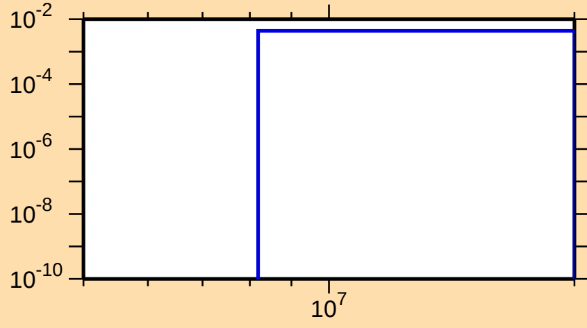
\sigma vs. E for ^{46}\text{Ti}(n,n\alpha)
