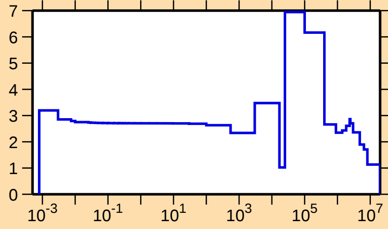
\sigma vs. E for ^{46}\text{Ti}(n,\text{el.})
