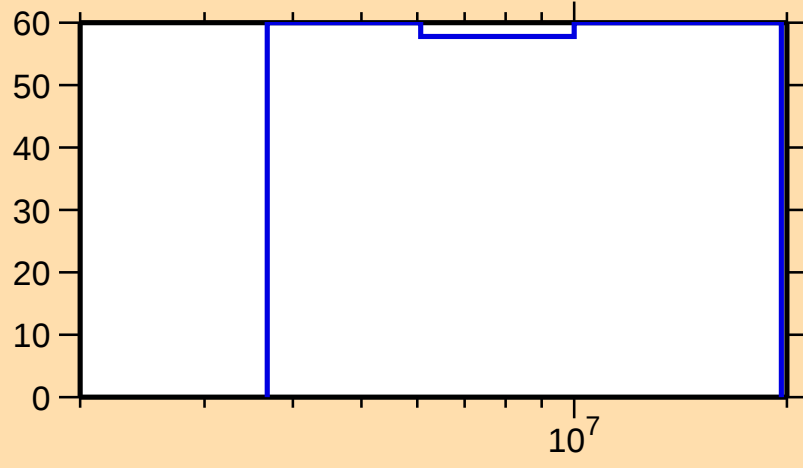
\Delta\sigma/\sigma vs. E for ^{51}\text{Ti}(n,p)
