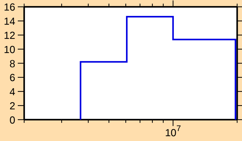
\Delta\sigma/\sigma vs. E for ^{51}\text{Ti}(\text{n},\text{el.})
