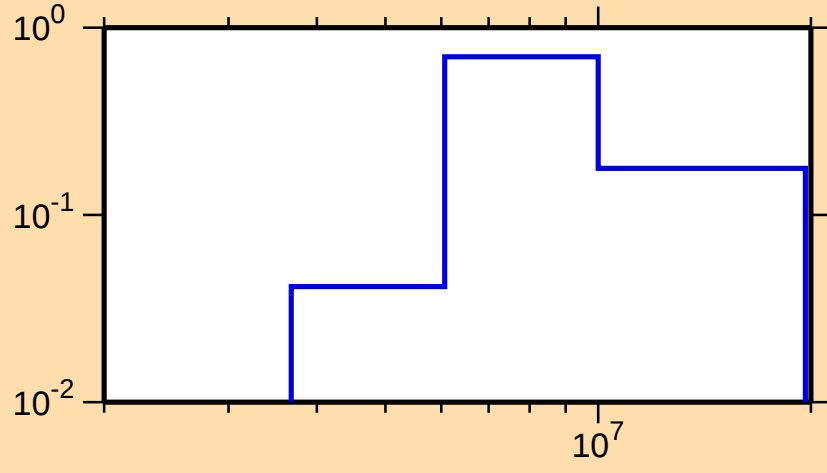
\sigma vs. E for ^{51}\text{Ti}(\text{n},\text{ncont.})
