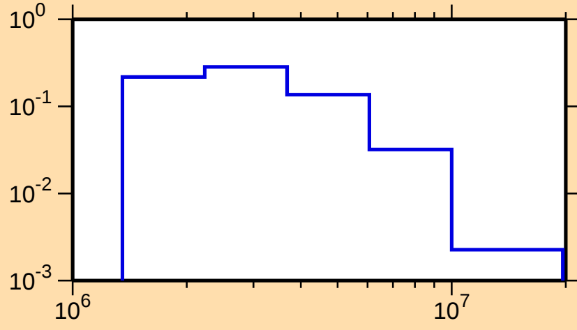
\sigma vs. E for ^{51}\text{Ti}(n,n_2)
