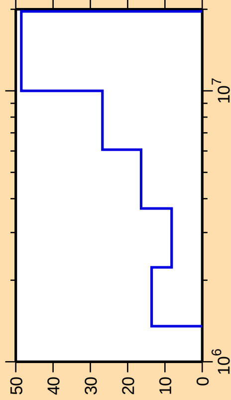
\Delta\sigma/\sigma vs. E for ^{51}\text{Ti}(n,n_2)
