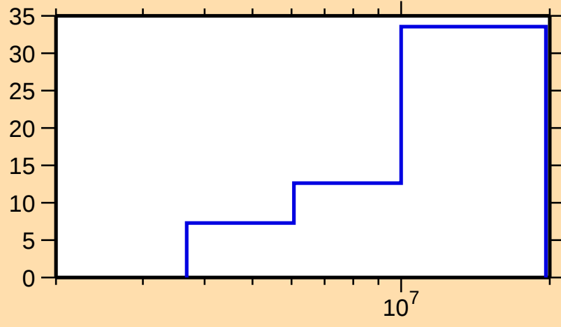
\Delta\sigma/\sigma vs. E for ^{51}\text{Ti}(\text{n},\text{inel.})
