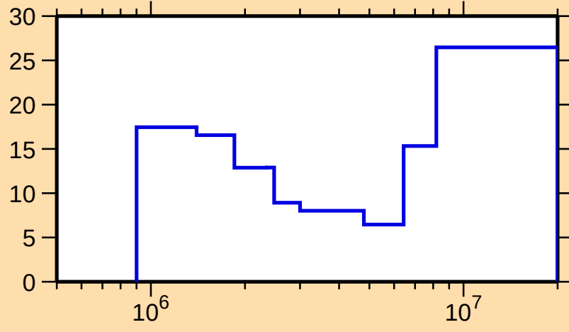
\Delta\sigma/\sigma vs. E for ^{51}\text{Ti}(n,\text{inel.})
