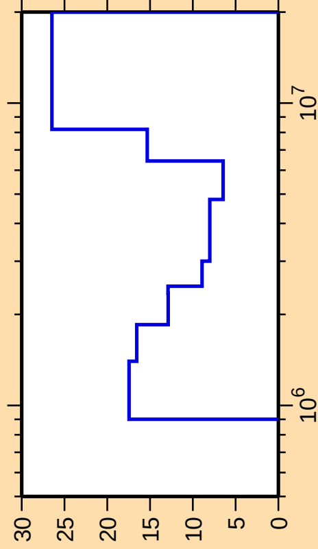
\Delta\sigma/\sigma vs. E for ^{51}\text{Ti}(\text{n,inel.})
