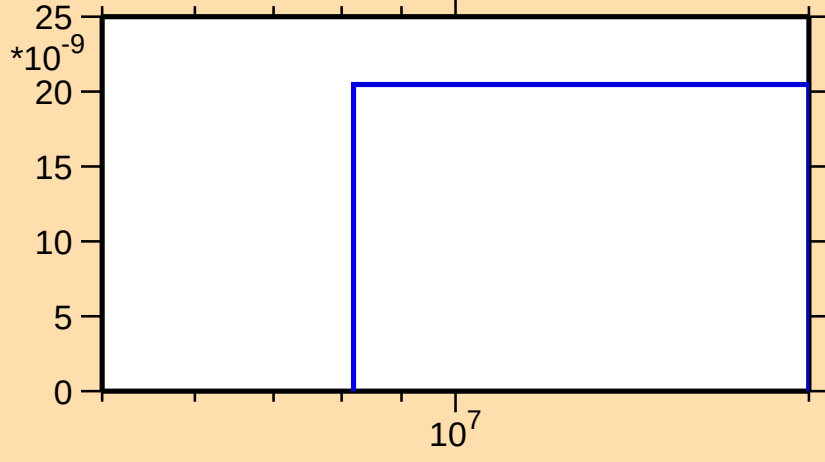
\sigma vs. E for ^{51}\text{Ti}(n,\text{nd})
