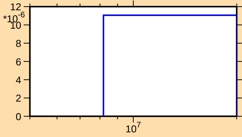
\sigma vs. E for ^{51}\text{Ti}(n,3n)
