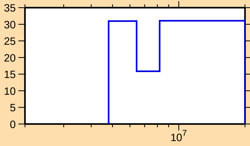
\Delta\sigma/\sigma vs. E for ^{51}\text{Ti}(n,n\text{cont.})
