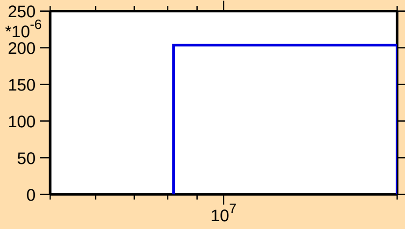
\sigma vs. E for ^{51}\text{Ti}(n,np)
