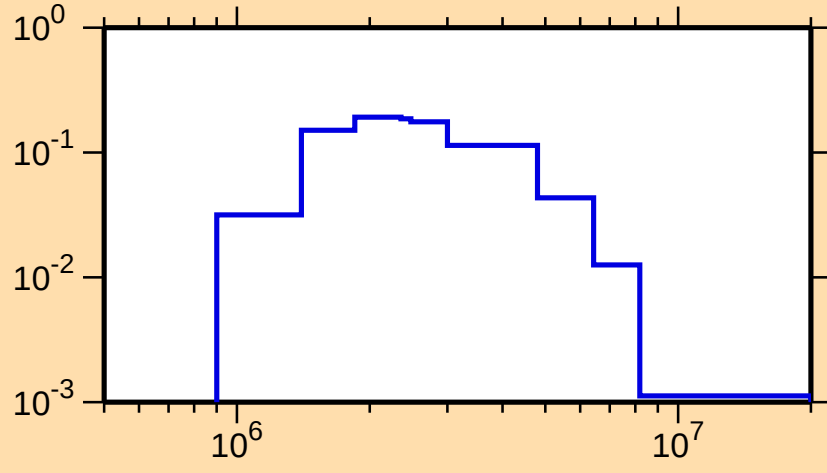
\sigma vs. E for ^{51}\text{Ti}(n,n_1)
