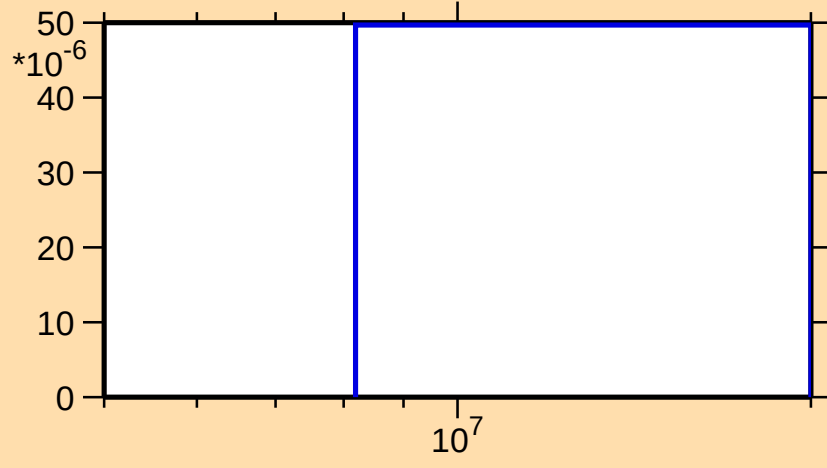
\sigma vs. E for ^{51}\text{Ti}(n,t)
