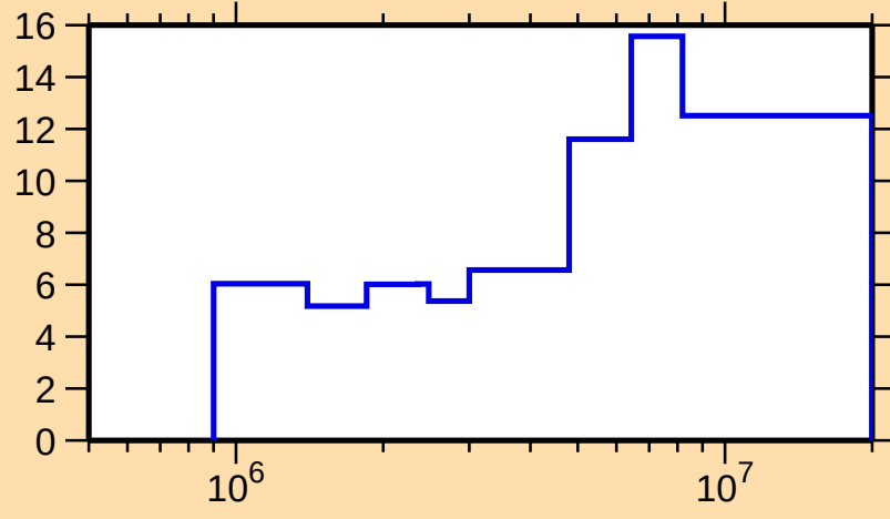
\Delta\sigma/\sigma vs. E for ^{51}\text{Ti}(\text{n,el.})
