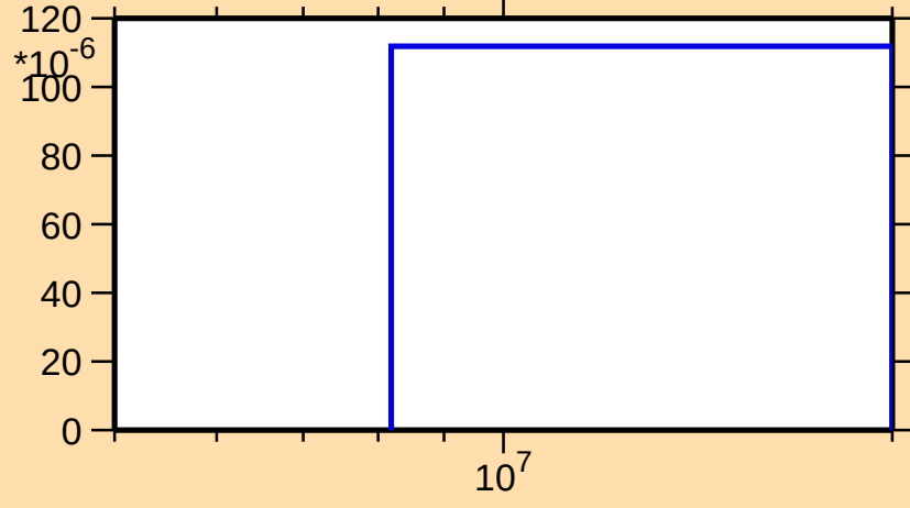
\sigma vs. E for ^{51}\text{Ti}(n,n\alpha)
