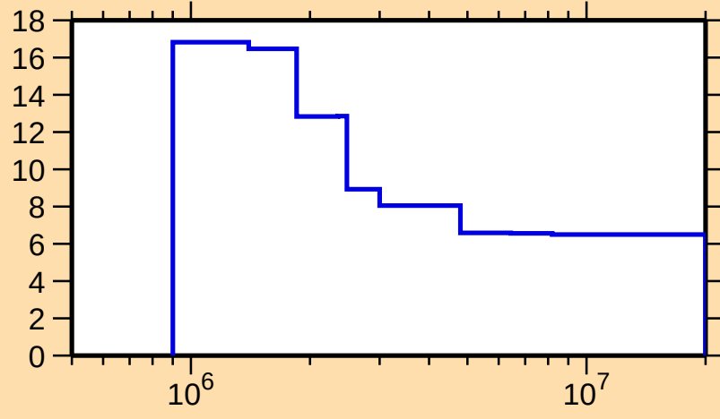
\Delta\sigma/\sigma vs. E for ^{51}\text{Ti}(n,\text{nonel.})
