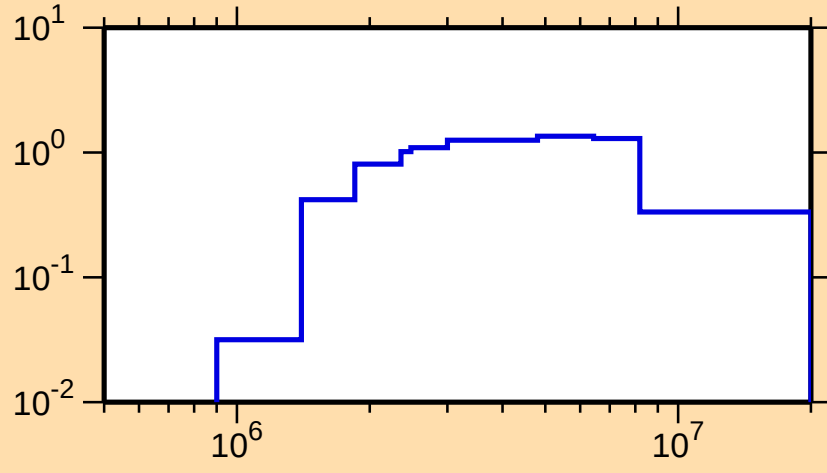
\sigma vs. E for ^{51}\text{Ti}(n,\text{inel.})
