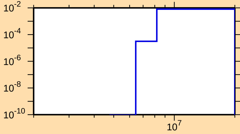
\sigma vs. E for ^{51}\text{Ti}(n,p)
