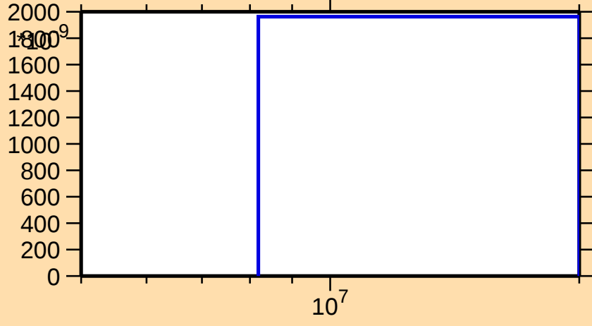
\sigma vs. E for ^{180}\text{Tl}(n,\text{nd})
