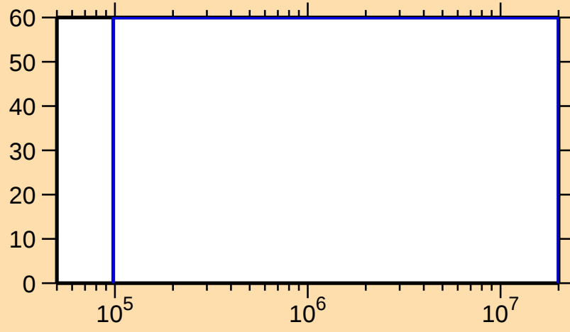
\Delta\sigma/\sigma vs. E for ^{185}\text{Tl}(n,n\text{cont.})
