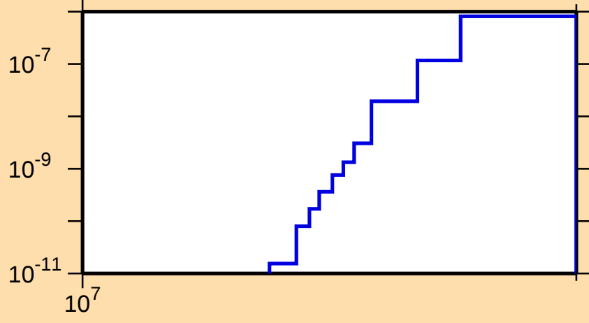
\sigma vs. E for ^{185}\text{Tl}(n,\text{nd})
