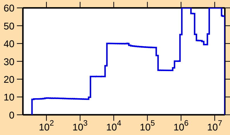
\Delta\sigma/\sigma vs. E for ^{185}\text{Tl}(n,\text{tot.})
