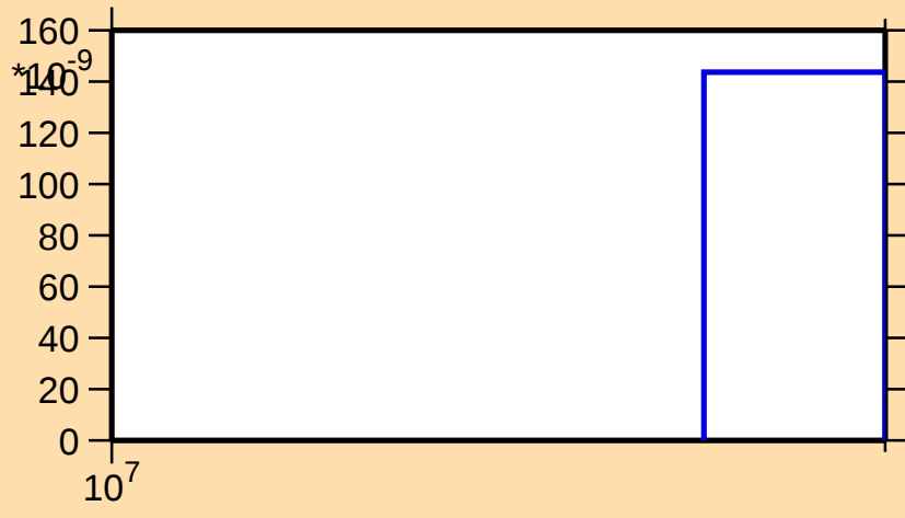
\sigma vs. E for ^{185}\text{Tl}(n,3n)
