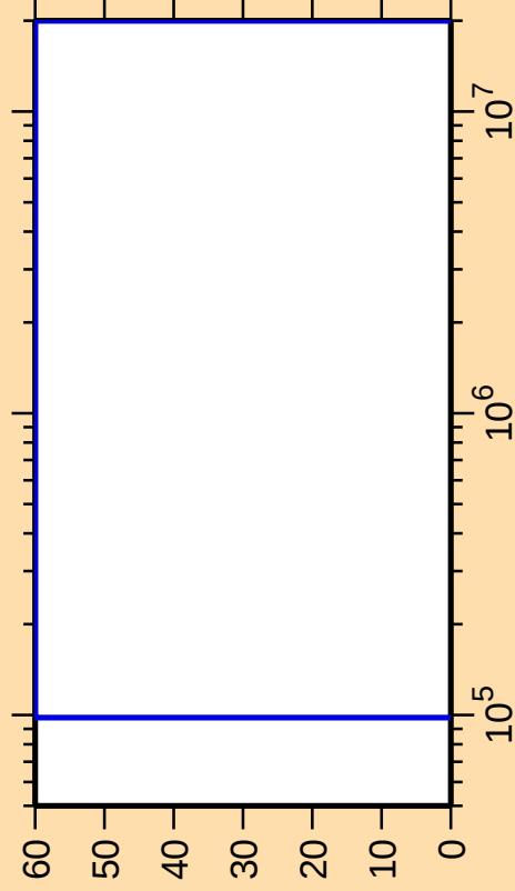
\Delta\sigma/\sigma vs. E for ^{185}\text{Tl}(n,\text{ncont.})
