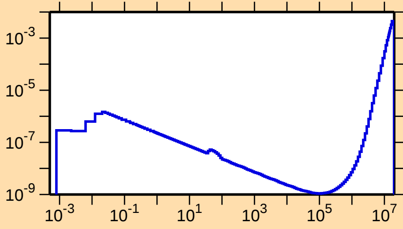
\sigma vs. E for ^{185}\text{Tl}(n,p\alpha)
