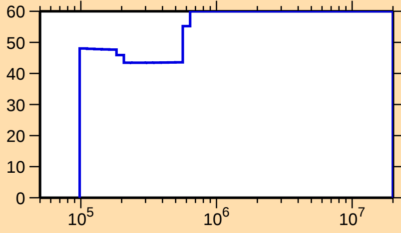
\Delta\sigma/\sigma vs. E for ^{185}\text{Tl}(n,\text{el.})
