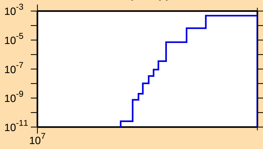
\sigma vs. E for ^{185}\text{Tl}(n,2np)
