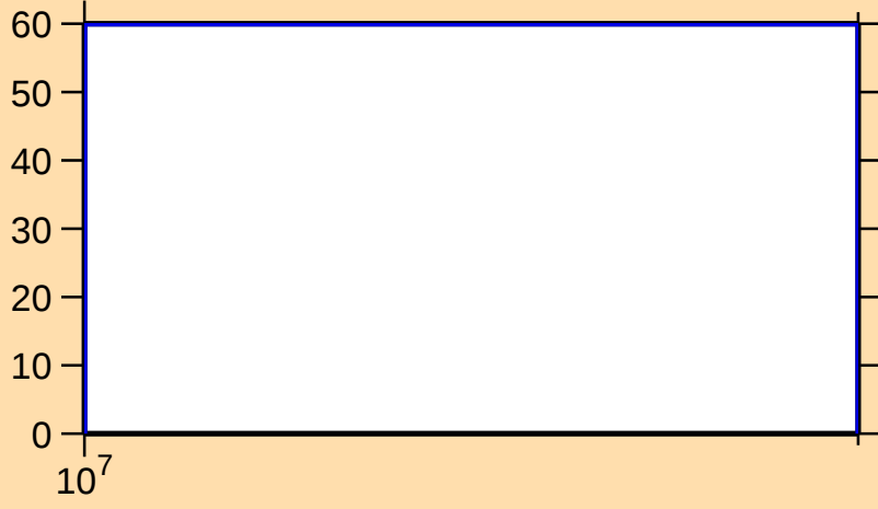
\Delta\sigma/\sigma vs. E for ^{185}\text{Tl}(n,\text{el.})
