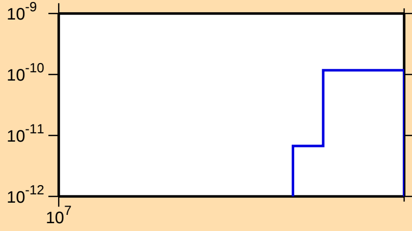
\sigma vs. E for ^{185}\text{Tl} (mt 34)
