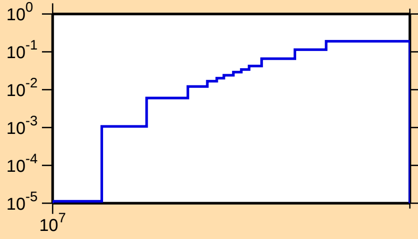
\sigma vs. E for ^{185}\text{Tl}(n,2n)
