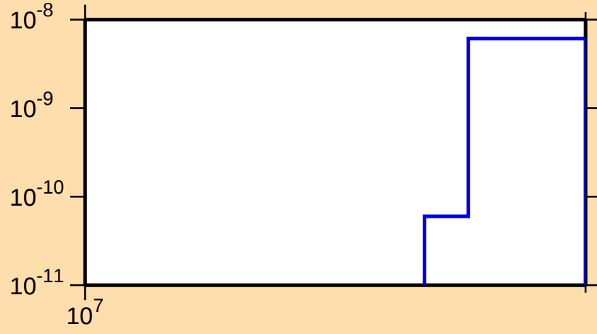
\sigma vs. E for ^{185}\text{Tl}(n,\text{nt})
