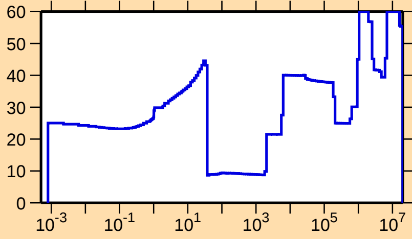
\Delta\sigma/\sigma vs. E for ^{185}\text{Tl}(n,\text{tot.})
