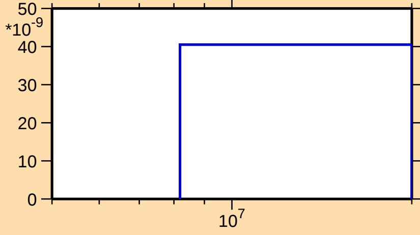
\sigma vs. E for ^{185}\text{Tl}(n,\text{pd})
