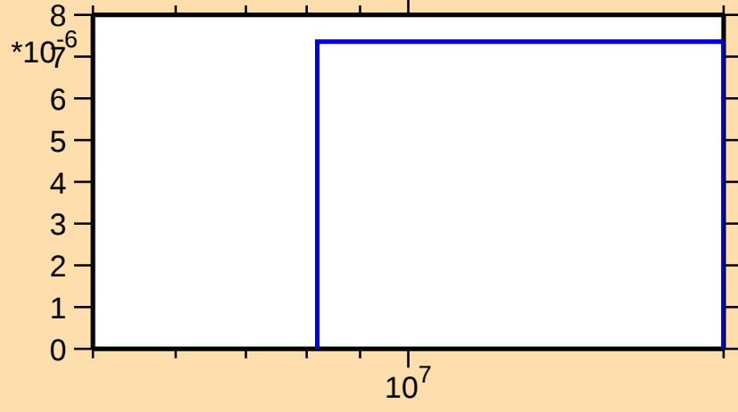
\sigma vs. E for ^{185}\text{Tl}(n,2np)
