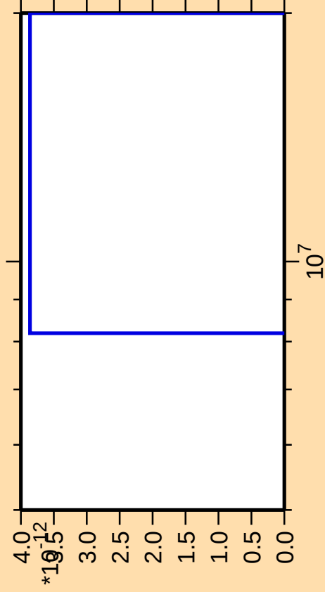
\Delta\sigma/\sigma vs. E for ^{185}\text{Tl}(\text{mt } 42)
