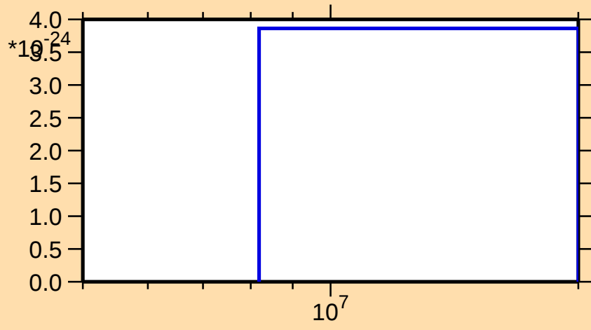
\sigma vs. E for ^{185}\text{Tl}(\text{mt } 42)
