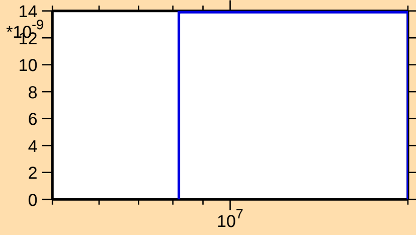
\sigma vs. E for ^{185}\text{Tl}(n,\text{nd})
