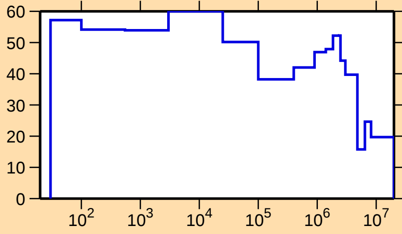
\Delta\sigma/\sigma vs. E for ^{185}\text{Tl}(n,\text{nonel.})
