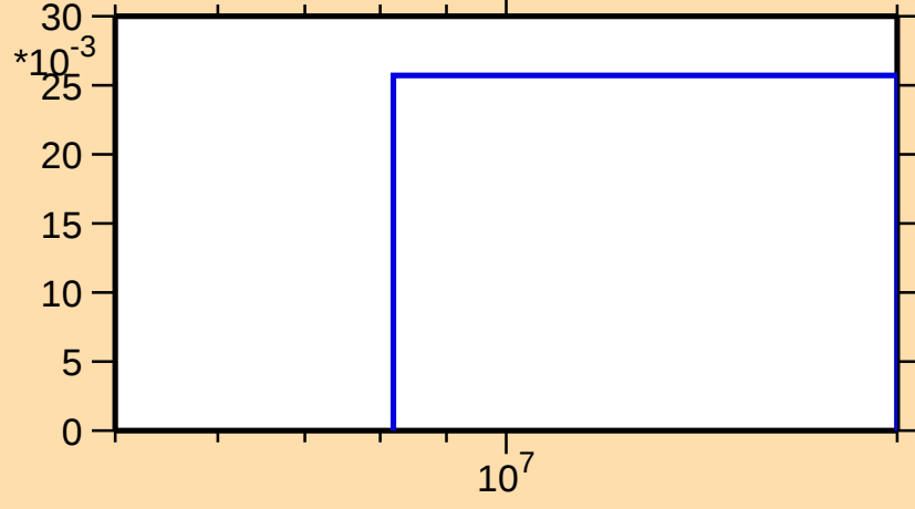
\sigma vs. E for ^{185}\text{Tl}(n,2n)
