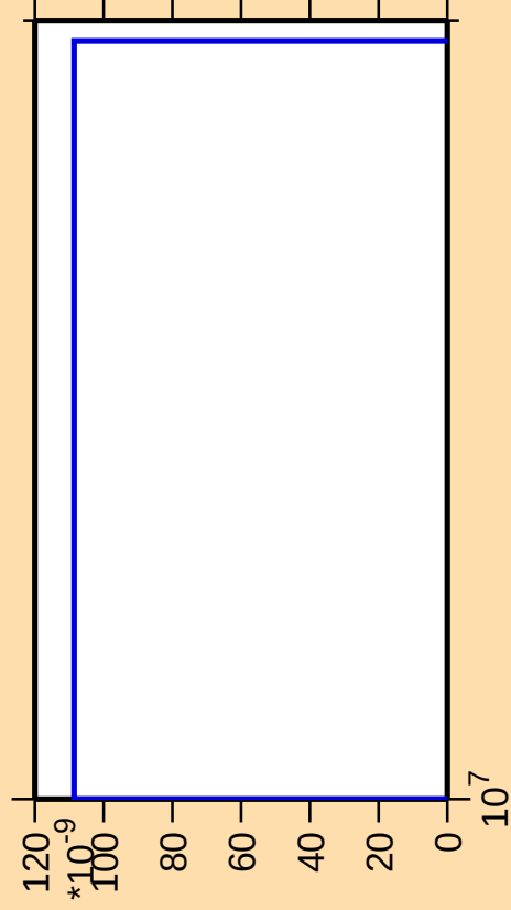
\Delta\sigma/\sigma vs. E for ^{188}\text{Tl}(\text{mt } 42)
