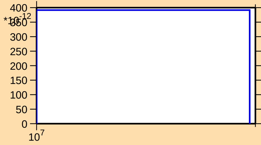
\sigma vs. E for ^{188}\text{Tl}(n,3n\alpha)
