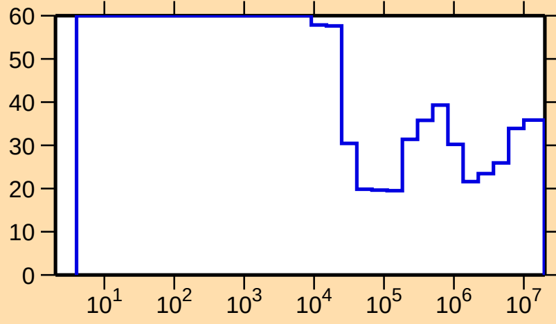
\Delta\sigma/\sigma vs. E for ^{188}\text{Tl}(n,\text{tot.})
