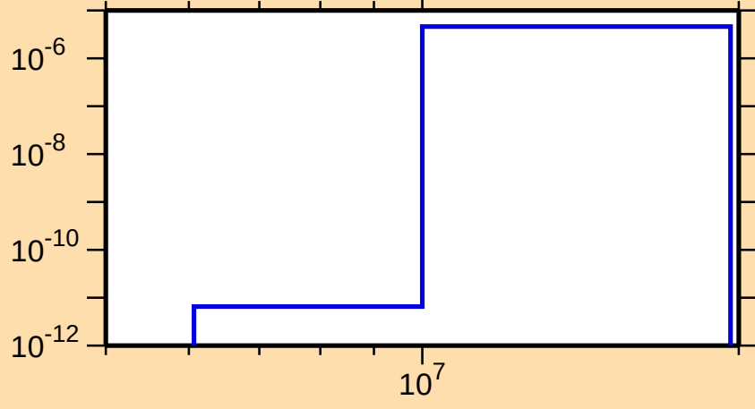
\sigma vs. E for ^{188}\text{Tl}(n,2n\alpha)
