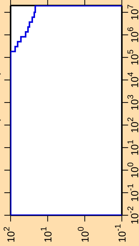
\Delta\sigma/\sigma vs. E for ^{188}\text{Tl}(n,\text{nonel.})
