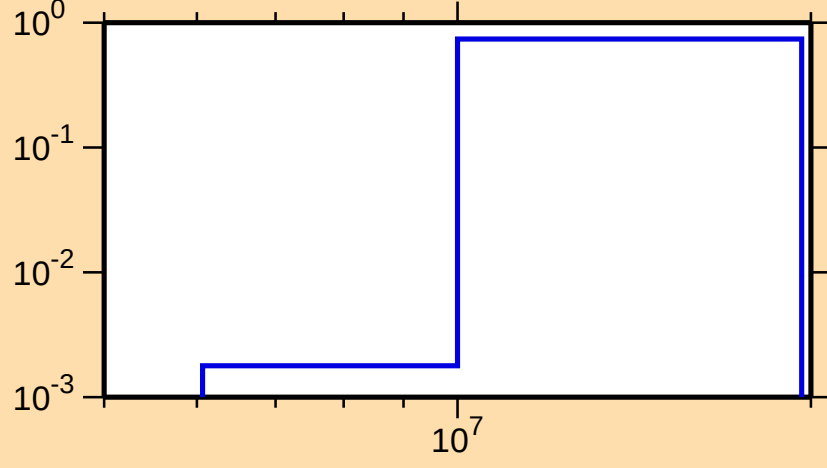
\sigma vs. E for ^{188}\text{Tl}(n,2n)
