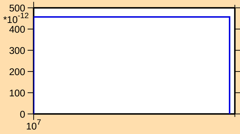
\sigma vs. E for ^{188}\text{Tl}(n,\text{pt})
