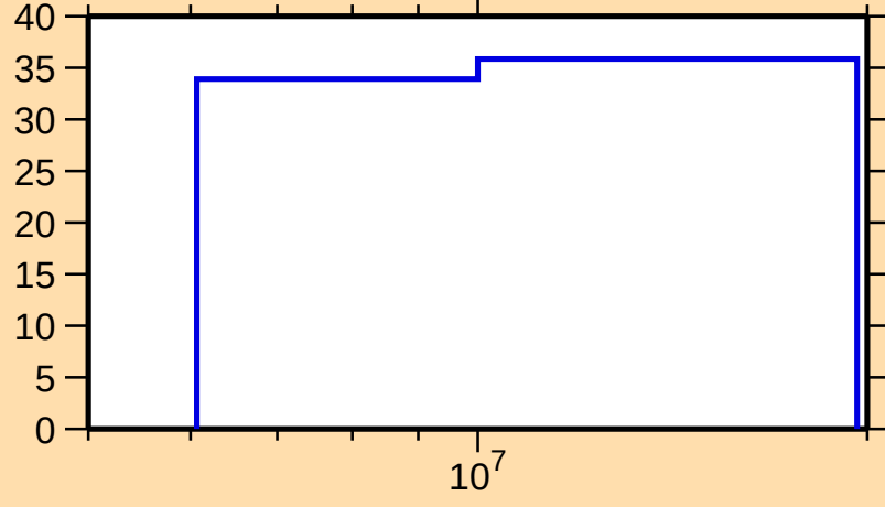
\Delta\sigma/\sigma vs. E for ^{188}\text{Tl}(n,\text{tot.})
