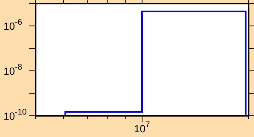
\sigma vs. E for ^{188}\text{Tl}(n,\text{He}3)
