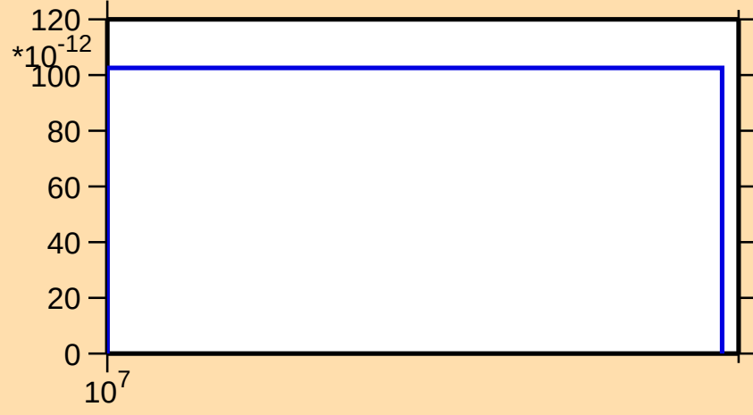
\sigma vs. E for ^{188}\text{Tl}(n,\text{nt})
