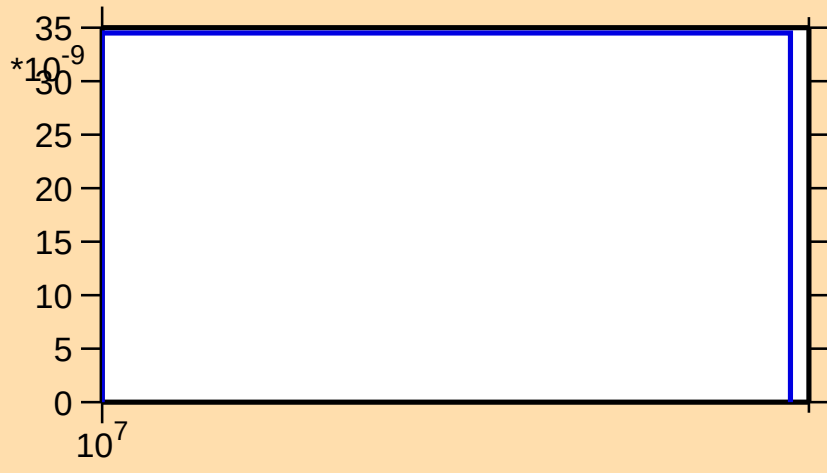
\sigma vs. E for ^{188}\text{Tl}(n,3n)
