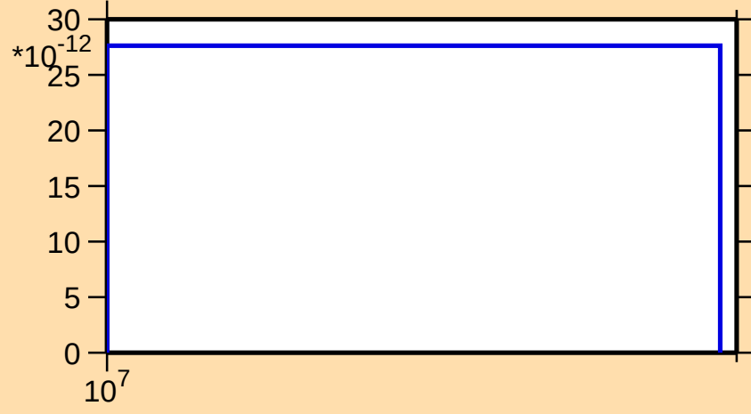
\sigma vs. E for ^{188}\text{Tl}(\text{mt } 34)
