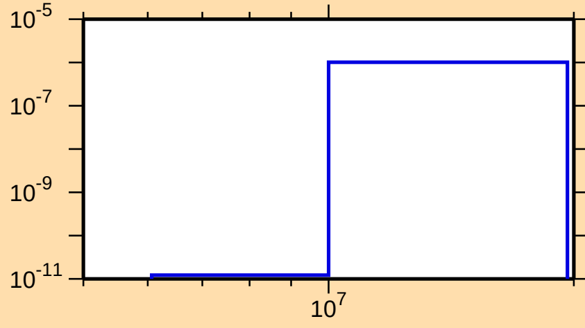
\sigma vs. E for ^{188}\text{Tl}(\text{mt } 45)
