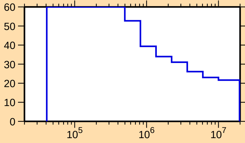
\Delta\sigma/\sigma vs. E for ^{188}\text{Tl}(n,n\text{onel.})
