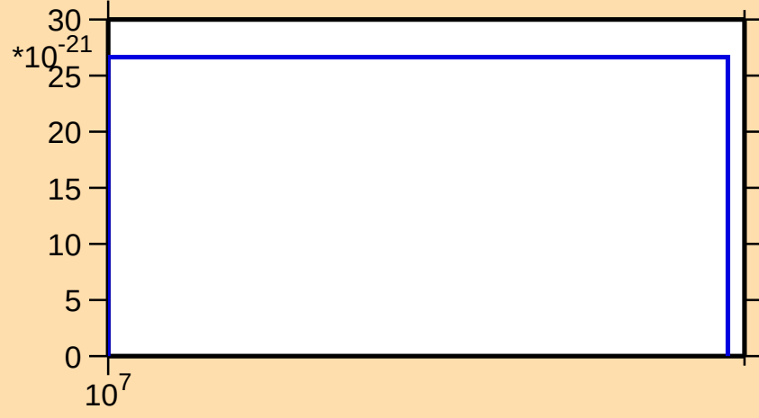
\sigma vs. E for ^{188}\text{Tl}(\text{mt } 42)
