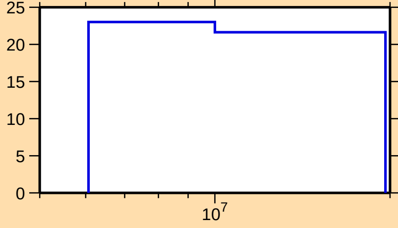
\Delta\sigma/\sigma vs. E for ^{188}\text{Tl}(n,\text{nonel.})
