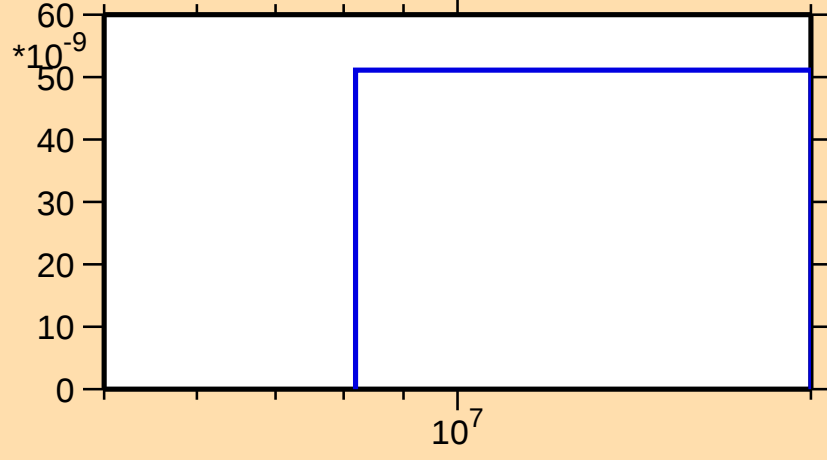
\sigma vs. E for ^{188}\text{Tl}(n,3n)
