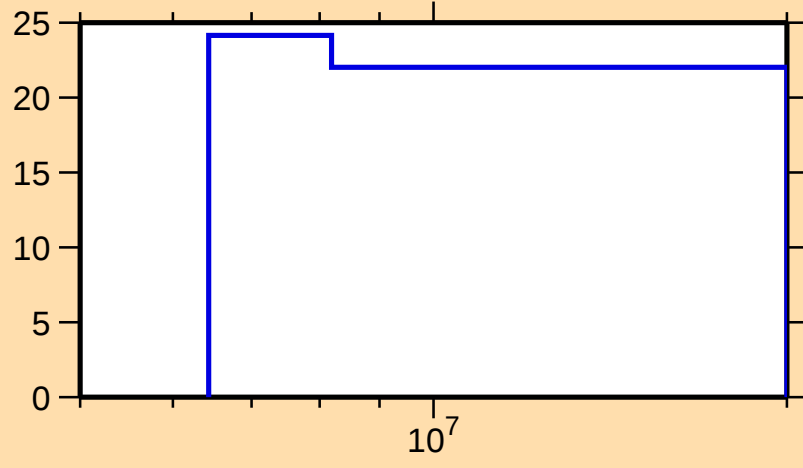
\Delta\sigma/\sigma vs. E for ^{188}\text{Tl}(n,\text{nonel.})
