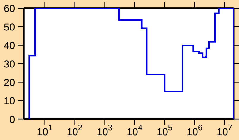
\Delta\sigma/\sigma vs. E for ^{188}\text{Tl}(n,\text{el.})
