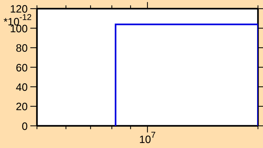
\sigma vs. E for ^{188}\text{Tl}(n,nt)
