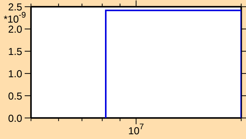
\sigma vs. E for ^{188}\text{Tl}(n,\text{pd})
