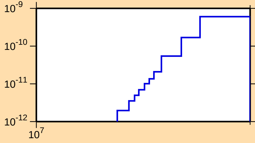
\sigma vs. E for ^{191}\text{Tl}(\text{mt117})
