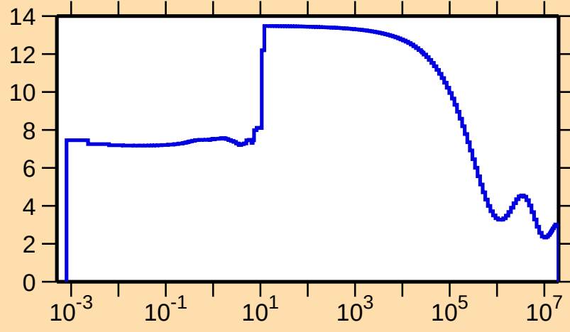
\sigma vs. E for ^{191}\text{Tl}(n,\text{el.})
