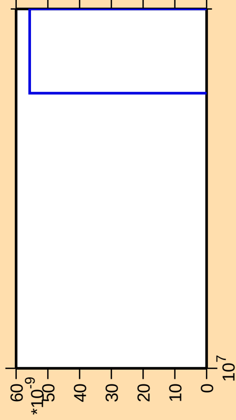
\Delta\sigma/\sigma vs. E for ^{191}\text{Tl} (mt 42)
