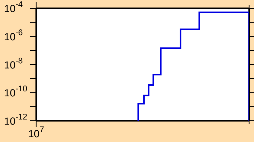
\sigma vs. E for ^{191}\text{Tl}(n,2np)
