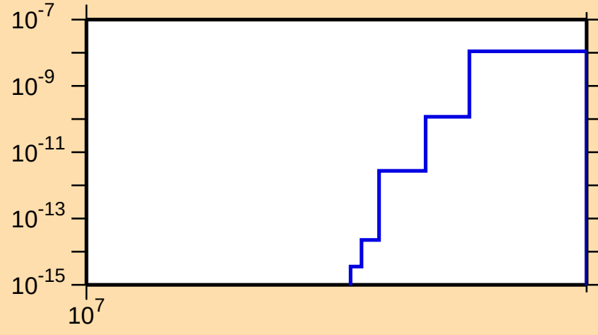
\sigma vs. E for ^{191}\text{Tl}(n,nt)
