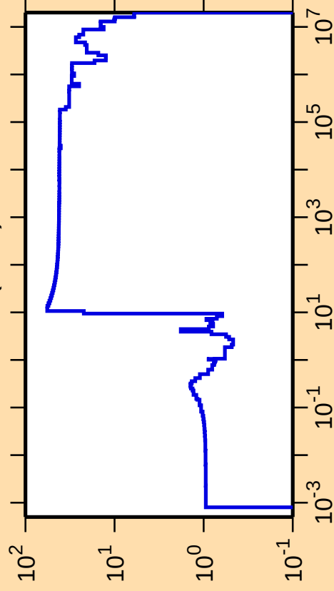
\Delta\sigma/\sigma vs. E for ^{191}\text{Tl}(n,\text{el.})
