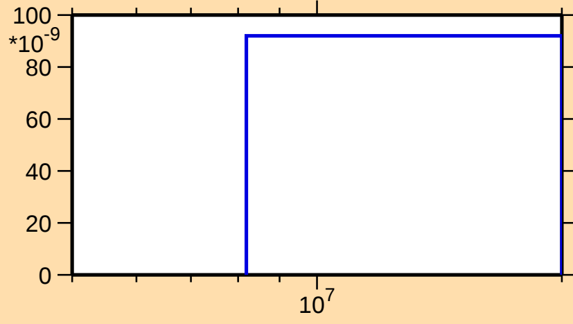
\sigma vs. E for ^{191}\text{Tl}(n,\text{He}3)
