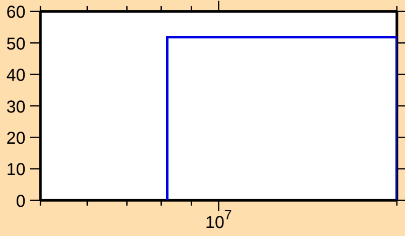
\Delta\sigma/\sigma vs. E for ^{191}\text{Tl}(n,2n)
