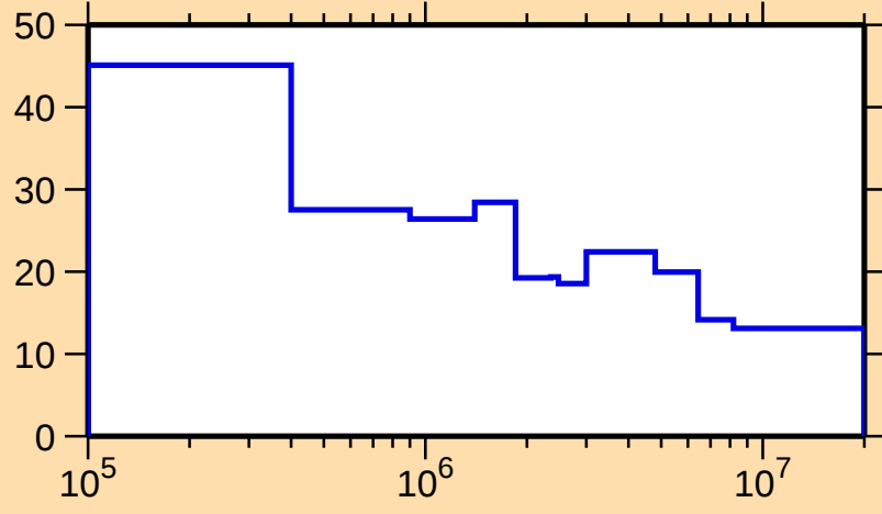
\Delta\sigma/\sigma vs. E for ^{192}\text{Tl}(n,\text{nonel.})
