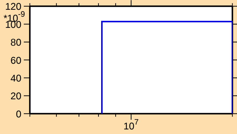
\sigma vs. E for ^{192}\text{Tl}(n,\text{He3})
