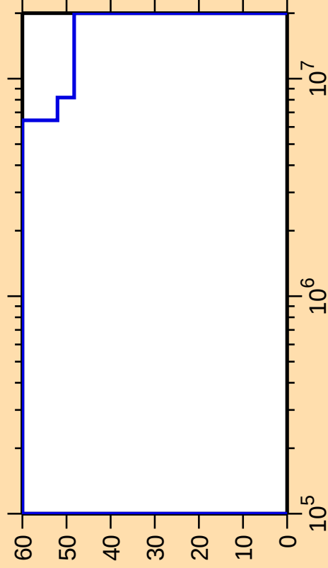
\Delta\sigma/\sigma vs. E for ^{192}\text{Tl}(n,p)
