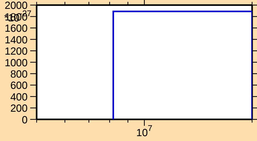
\sigma vs. E for ^{192}\text{Tl}(\text{mt } 42)
