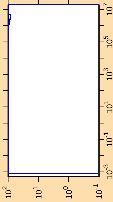
\Delta\sigma/\sigma vs. E for ^{193}\text{Tl}(n,\alpha)
