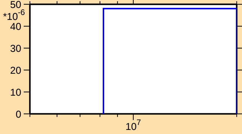
\sigma vs. E for ^{193}\text{Tl}(n,t)
