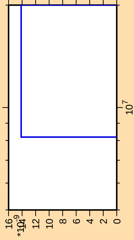
\Delta\sigma/\sigma vs. E for ^{193}\text{Tl} (mt 42)
