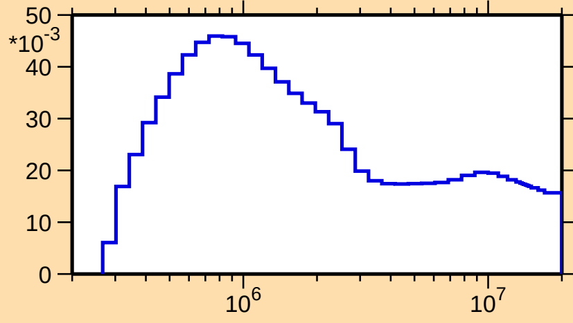
\sigma vs. E for ^{194}\text{Tl}(n,n_4)
