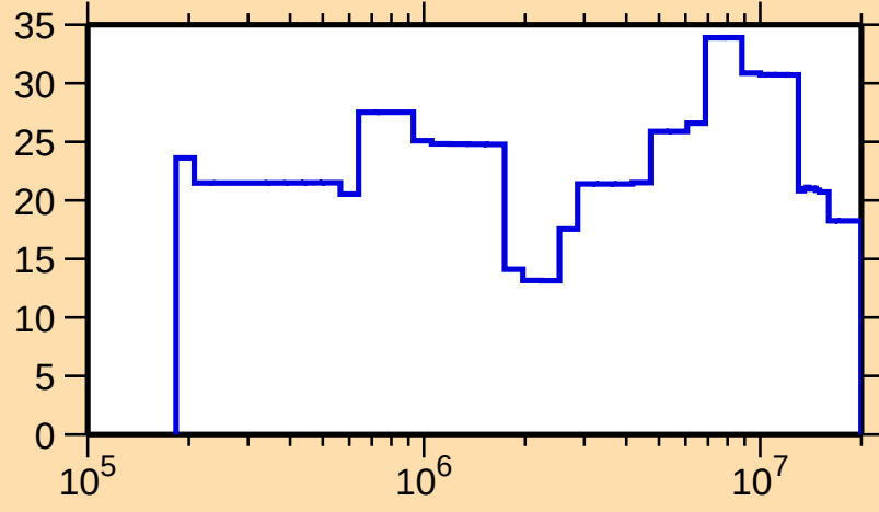
\Delta\sigma/\sigma vs. E for ^{194}\text{Tl}(n,\text{el.})
