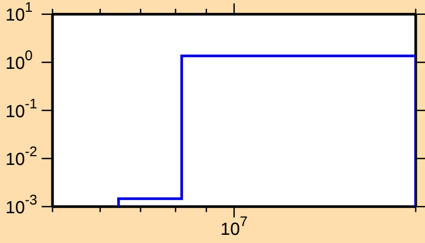
\sigma vs. E for ^{194}\text{Tl}(n,2n)
