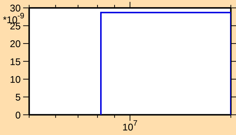
\sigma vs. E for ^{194}\text{Tl}(n,2n\alpha)
