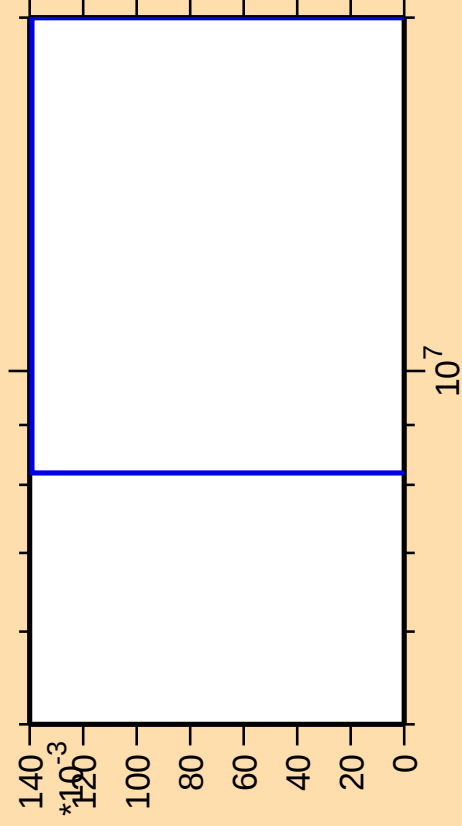
\Delta\sigma/\sigma vs. E for ^{194}\text{Tl}(n,\text{pt})
