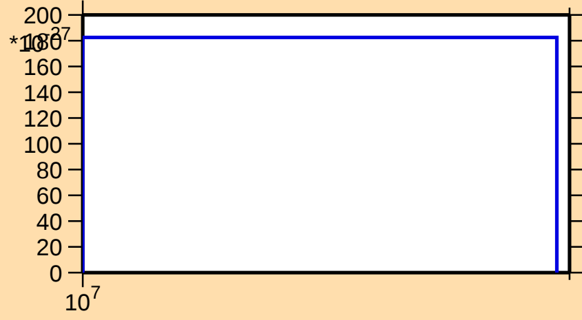
\sigma vs. E for ^{196}\text{Tl}(\text{mt } 42)
